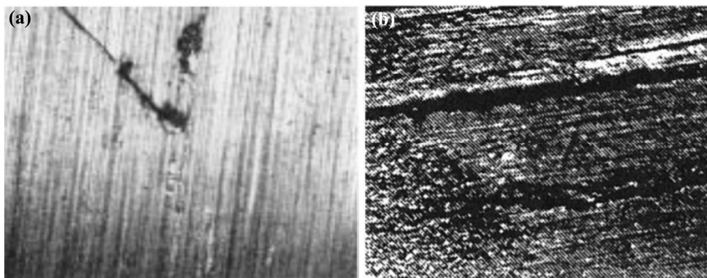
Fig. 8 (a) Molten spark tracks. Reproduced with permission from Ref. [93], © IEEE 2000. (b) 60 times magnification of a spark track. Reproduced with permission from Ref. [85], © IEEE 1991.
