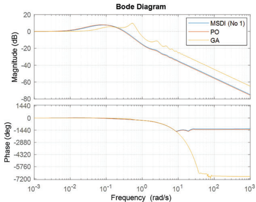
Figure 11: Bode diagram
