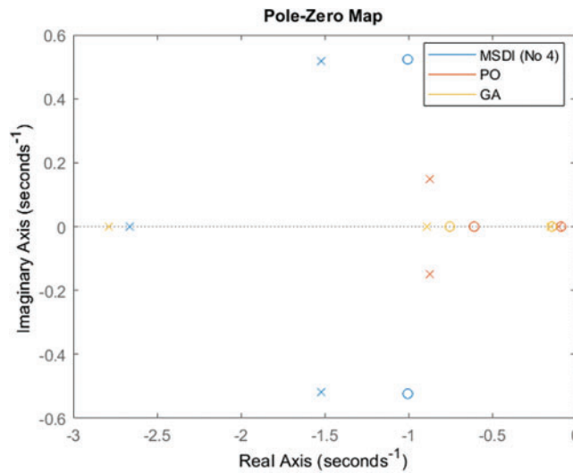
Figure 6: Pole-zero map
