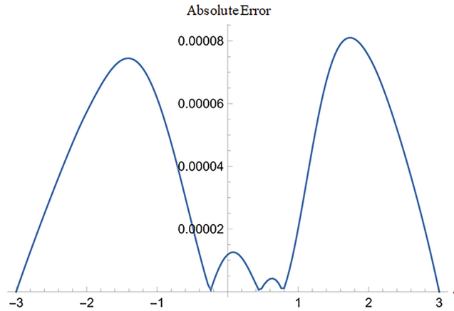
Figure 5: Absolute error distribution for Example 2 at t = 1 when h = 0.04 , \eta = 0.5 and \Delta t = 0.0001 . The symmetric error patterns confirm the stability of our method, with errors remaining bounded throughout the computational domain
