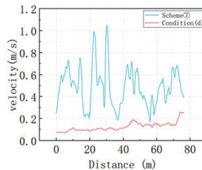
Figure 13: Wind speed analysis scheme at 1.5 m for each design option
