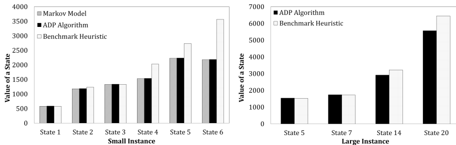
Fig. 2. Performance of the ADP Algorithm in the Small and Large Instance
