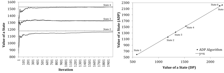
Fig. 1. Convergence and Approximation Accuracy of the ADP Algorithm
