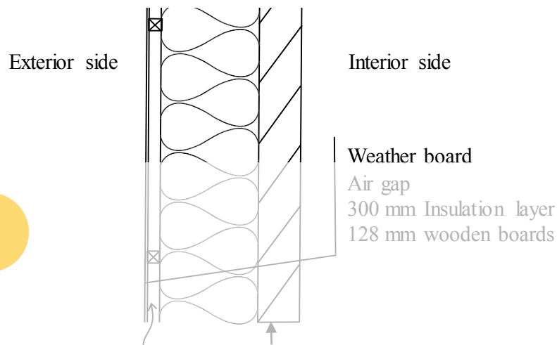
Figure 2. Insulated wooden wall that is investigated. The monitoring position is marked by the arrow.
