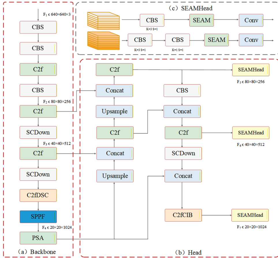
Figure 1: All the overall architecture of the proposed YOLOv10_DSE. (a) Backbone feature extraction network consisting of C2f, C2fDSC; (b) Head network consisting of key modules such as, SEAMHead, inner_CIoU; (c) A detection head employing self-ensemble attention mechanisms (SEAMHead) is applied to both regression heads and classification heads
