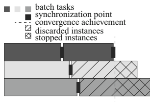
Fig. 6 Theoretical trace of the asynchronous framework. Different gray colors of the rectangles represent different batches. Each batch contains all the tasks from the execution of the instances ( ExecuteInstance ) to the check of the convergence ( CheckConvergence ). The black rectangles are the synchronization points. The dashed vertical line denotes the achievement of the algorithm convergence after four iterations. The two types of parallel diagonal lines indicate that the instances of the unfinished batches are discarded (left with respect to the dashed line) or stopped (right with respect to the dashed line)
