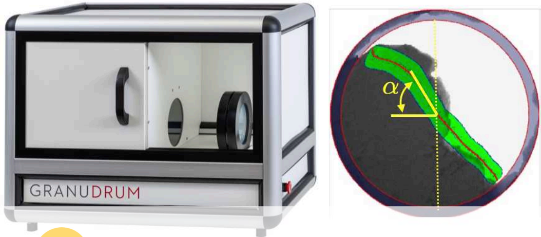
Figure 1: (Left) Picture of the GranuDrum instrument used to perform the flow measurement in the rotating drum. (Right) Snapshot taken during the image treatment for one rotating speed. In the background, a picture selected in the series of 50 images is shown. The average interface position is plotted in red and the standard deviation is plotted in green. The flowing angle \alpha measurement at the center of the interface is highlighted in yellow.
