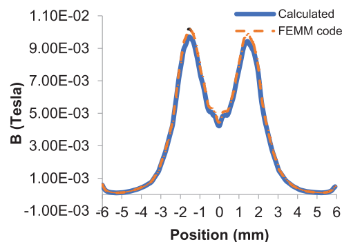
Figure 4: Evaluation of the magnetic induction B , comparison between calculated and FEMM results
