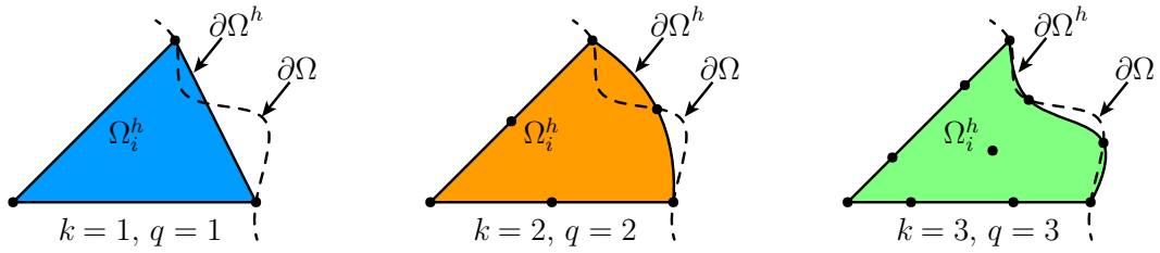
Figure 3: Illustration of a degree adaptation in an element where the same degree of approximation is used for both the solution and the geometry.
