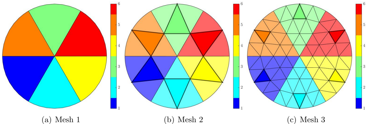
Figure 4: First three NEFEM meshes where the colour indicates the degree of approximation used in each element and the highlighted element represents the region where the error is measured for each degree of approximation.
