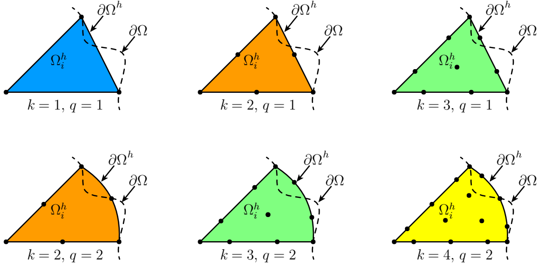
Figure 1: Illustration of a degree adaptation in an element with linear (top) and quadratic (bottom) approximation of the geometry.
