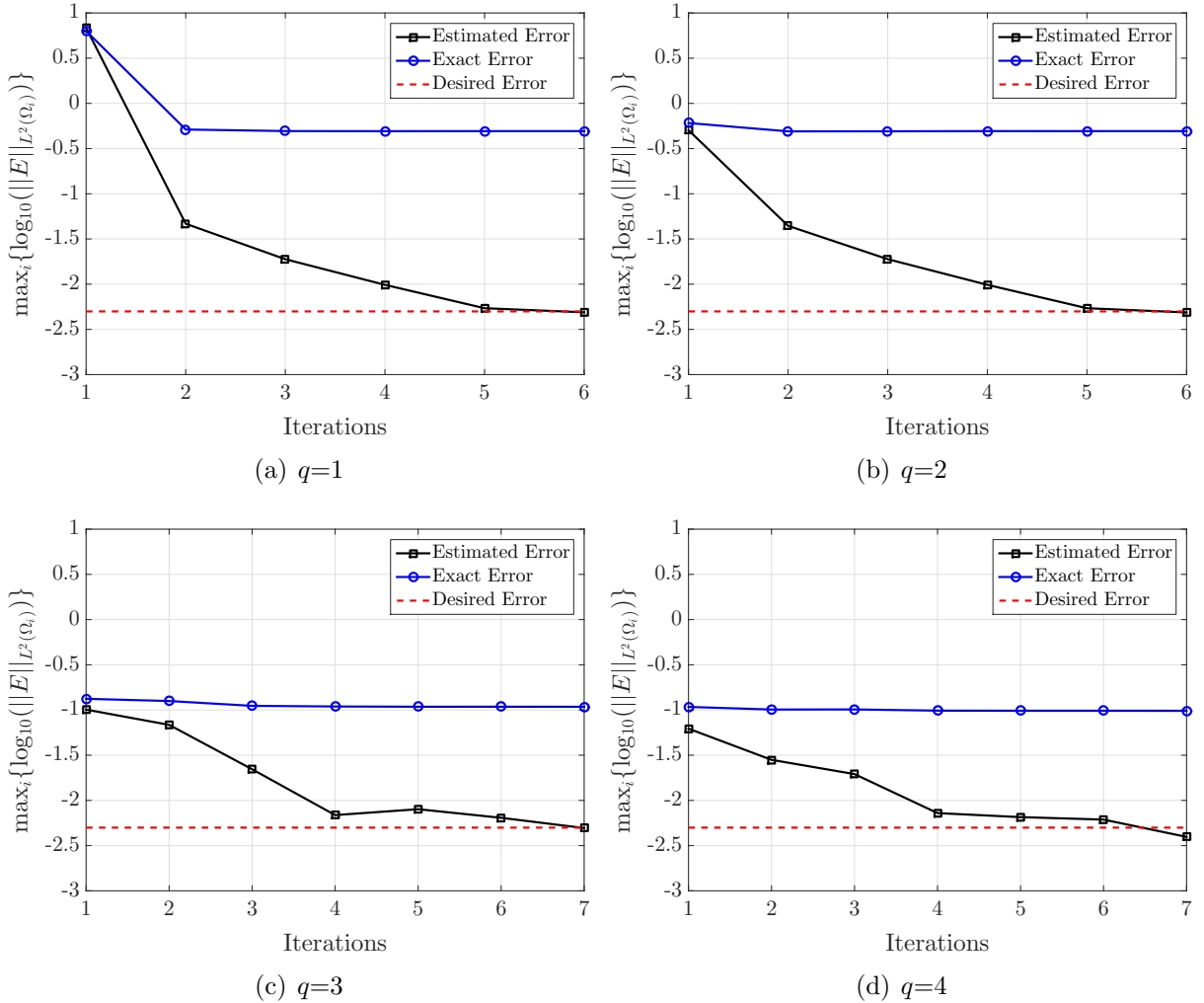
Figure 10: Evolution of the estimated and exact errors during a degree adaptivity process for different degrees of the polynomials used to approximate the geometry ( q ).
