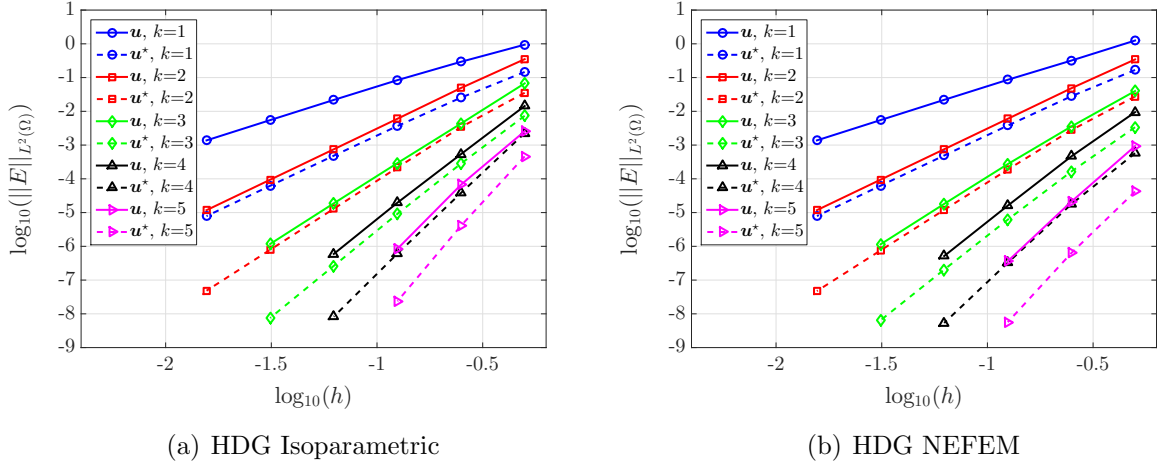
Figure 5: Error of the solution \mathbf{u} and the postprocessed solution \mathbf{u}^* in the \mathcal{L}_2(\Omega_e) norm for different degrees of approximation in each element.
