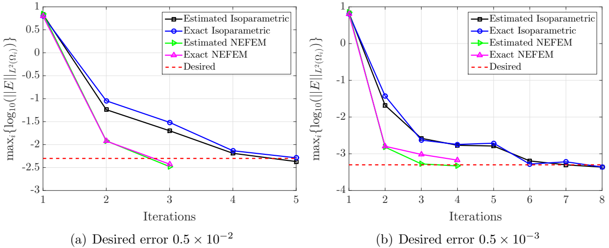
Figure 14: Estimated and exact errors for isoparametric and NEFEM.
