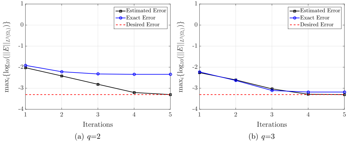
Figure 20: Evolution of the estimated and exact errors during the degree adaptivity process for q = 2 and q = 3 with isoparametric HDG in the coarse mesh with 2,443 elements and a desired error of 0.5 \times 10^{-3} .
