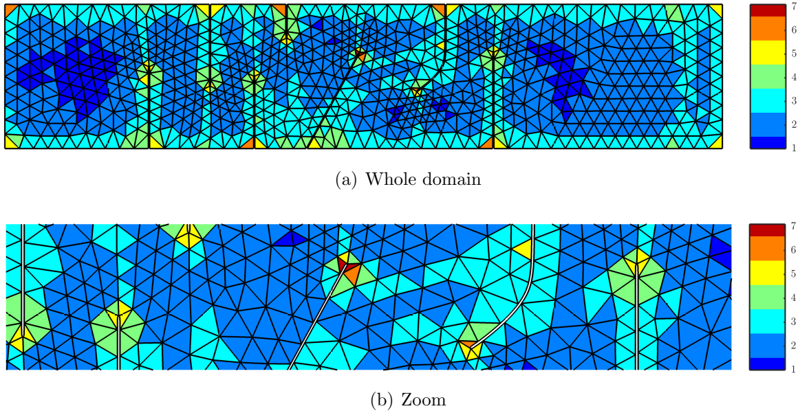
Figure 26: Mesh and degree of approximation of the converged degree adaptive procedure with HDG-NEFEM for the computation of the flow in a channel with high curvature.
