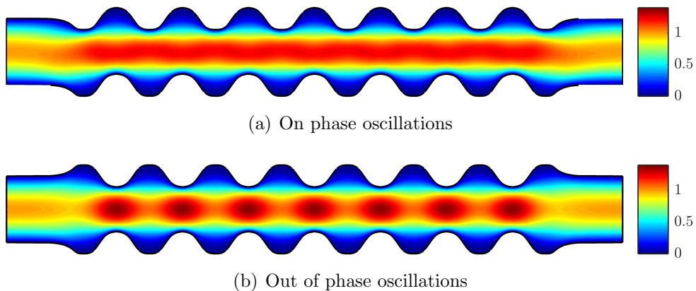
Figure 24: Magnitude of velocity computed with HDG-NEFEM after convergence of the degree adaptive procedure on the meshes shown in Figure 23.
