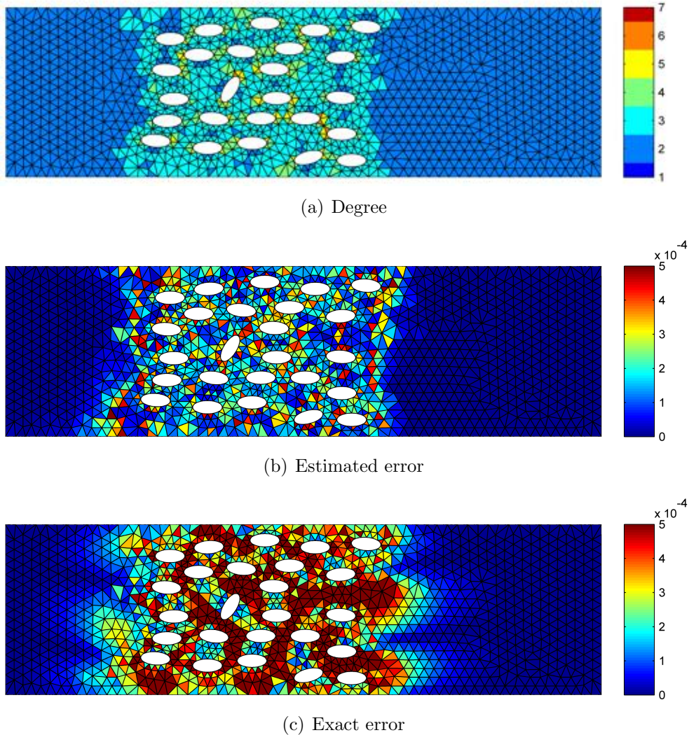
Figure 16: Final degree distribution, estimated and reference errors for an adaptive computation with isoparametric HDG and quadratic approximation of the curved boundaries in a coarse mesh with 2,443 elements.
