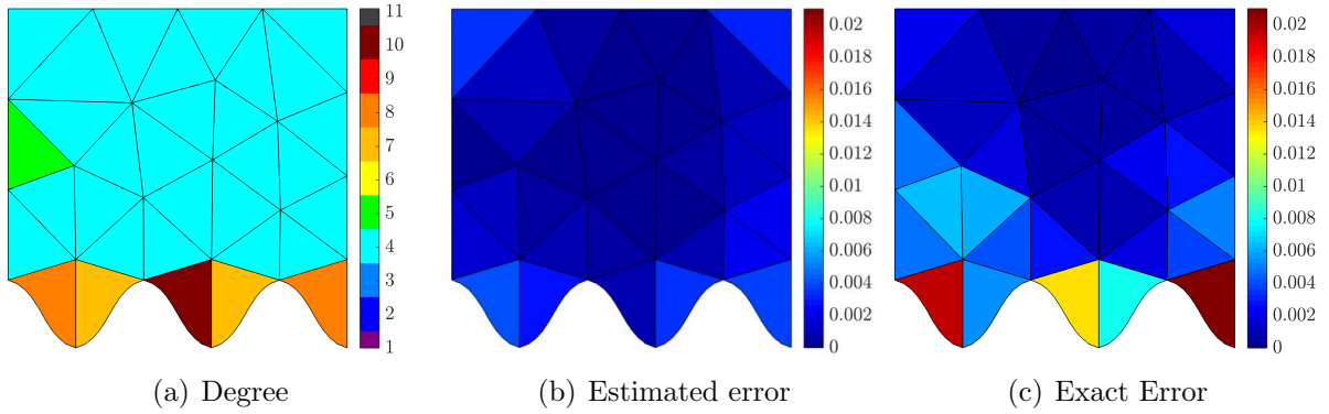
Figure 11: Sixth iteration of the degree adaptivity procedure with no geometric update using HDG isoparametric elements and q = 4 .
