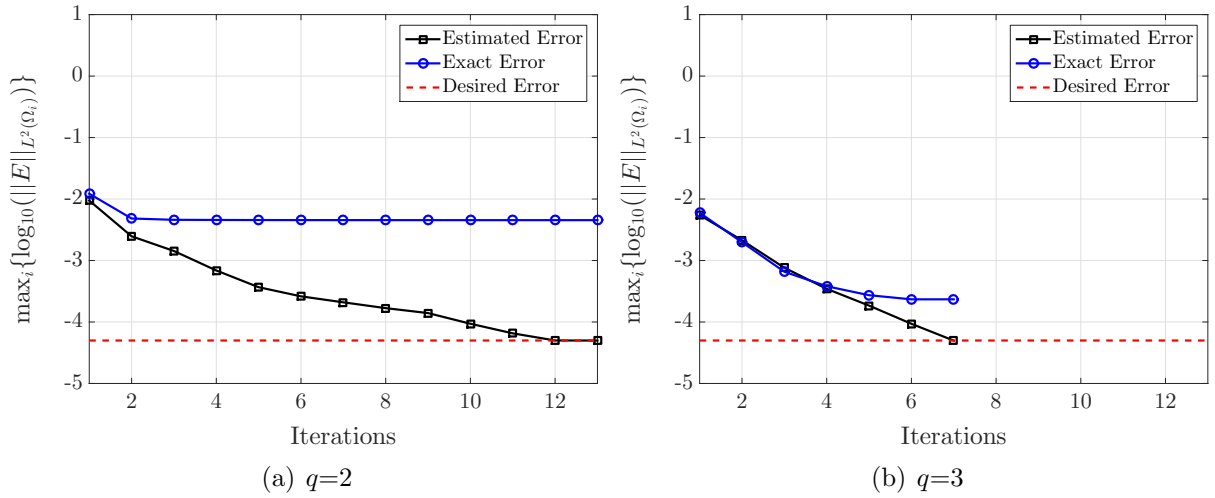
Figure 21: Evolution of the estimated and exact errors during the degree adaptivity process for q = 2 and q = 3 with isoparametric HDG in the coarse mesh with 2,443 elements and a desired error of 0.5 \times 10^{-4} .
