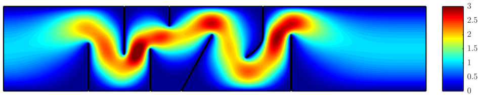
Figure 27: Velocity computed with HDG-NEFEM after convergence of the degree adaptive procedure in the mesh of Figure 26.
