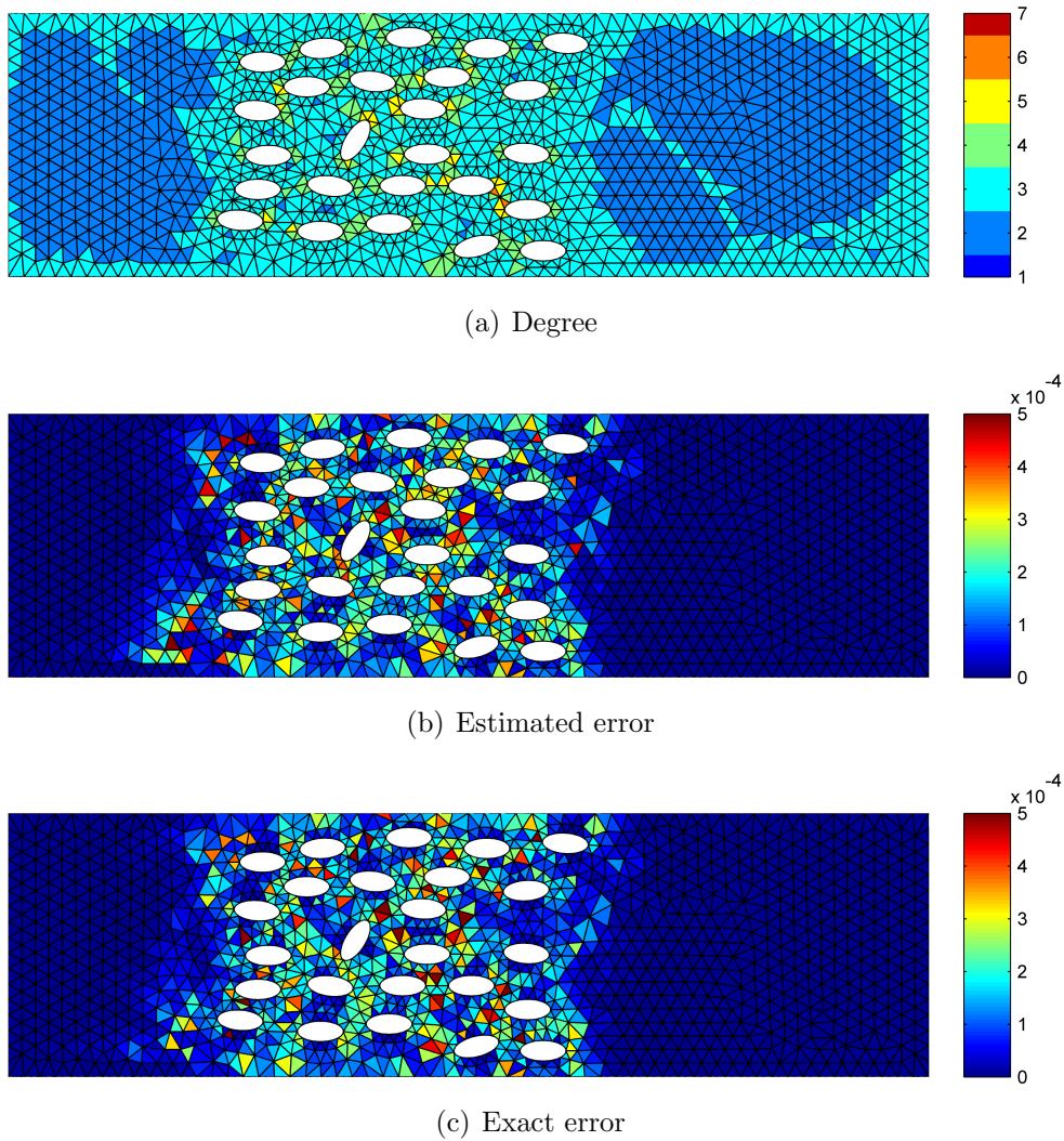
Figure 18: Final degree distribution, estimated and reference errors for an adaptive computation with HDG-NEFEM in a coarse mesh with 2,443 elements.
