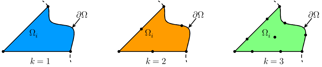
Figure 2: Illustration of a degree adaptation in a NEFEM element.
