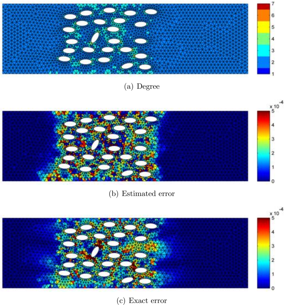
Figure 17: Final degree distribution, estimated and reference errors for an adaptive computation with isoparametric HDG and quadratic approximation of the curved boundaries in a finer mesh with 4,048 elements.
