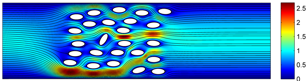
Figure 19: Magnitude of velocity and isolines computed with HDG-NEFEM on the mesh shown in Figure 18 (a) after four iterations of the degree adaptive process.
