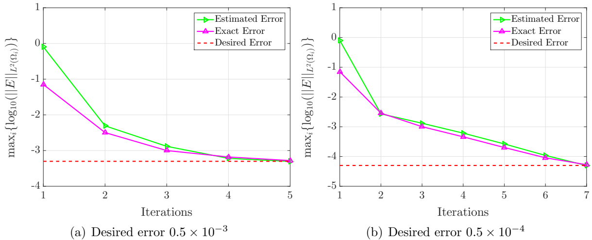
Figure 22: Evolution of the estimated and exact errors during the degree adaptivity process for NEFEM HDG in the coarse mesh with 2,443 elements.
