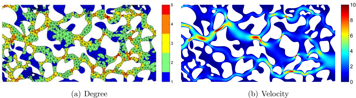
Figure 25: Mesh and degree of approximation of the converged degree adaptive procedure with HDG-NEFEM and velocity field.
