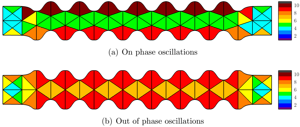
Figure 23: Mesh and degree of approximation of the converged degree adaptive procedure with HDG-NEFEM for the computation of the flow in a channel with oscillations of the top and bottom boundaries.
