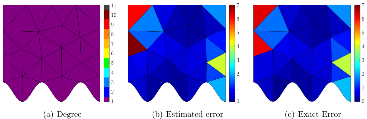
Figure 12: First iteration of the degree adaptivity procedure with geometric update using HDG NEFEM elements.
