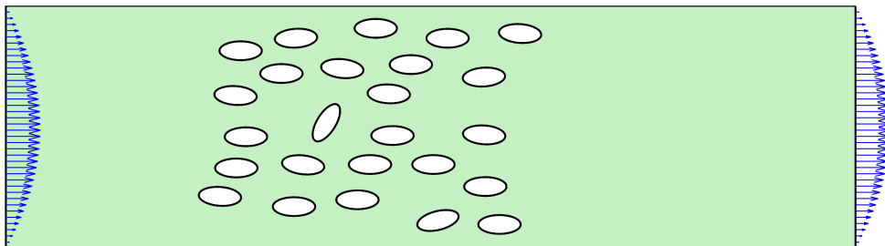
Figure 15: Computational domain and boundary conditions for the problem involving a flow in a channel with randomly distributed ellipses.
