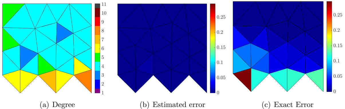
Figure 9: Sixth iteration of the degree adaptivity procedure with no geometric update using HDG isoparametric elements and q = 1 .
