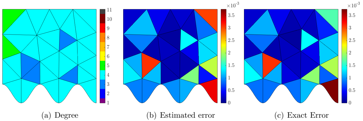
Figure 13: Third iteration of the degree adaptivity procedure with geometric update using HDG NEFEM elements.
