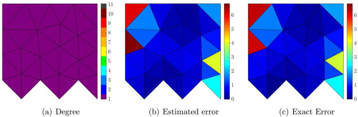
Figure 8: First iteration of the degree adaptivity procedure with HDG isoparametric elements.
