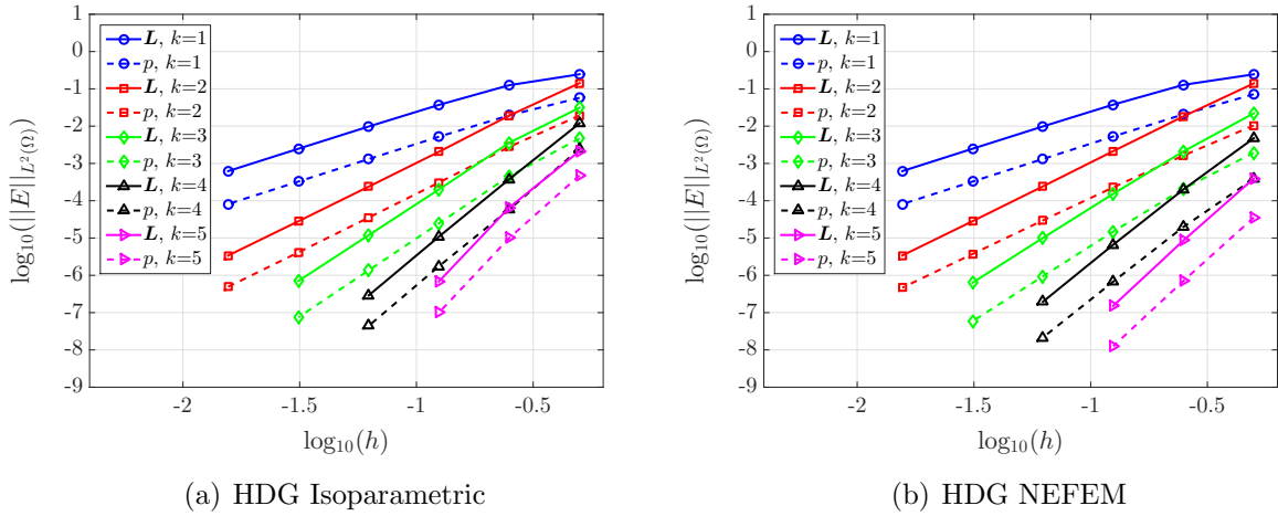
Figure 6: Error of the dual variable \mathbf{L} and the pressure p in the \mathcal{L}_2(\Omega_e) norm for different degrees of approximation in each element.
