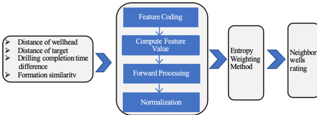
Figure 2: Multi-dimensional comprehensive evaluation system of offset wells.
