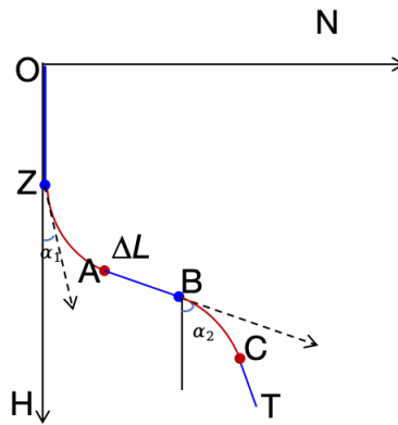
Figure 4: A 2D five-segment well trajectory.
