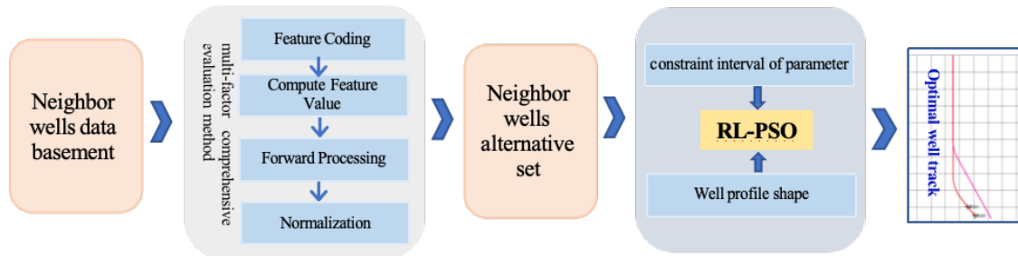
Figure 3: Intelligent well trajectory design flowchart.
