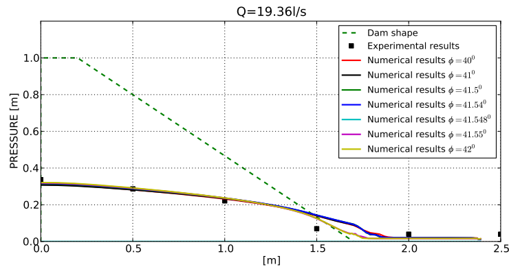
Figure 5.44: Case B21. Bottom pressure distribution at stationary regime for Q = 19.36\text{ l/s} . Porosity n = 0.4 , D_{50} = 35\text{ mm} . Numerical and experimental comparison for different internal friction angles \phi .
