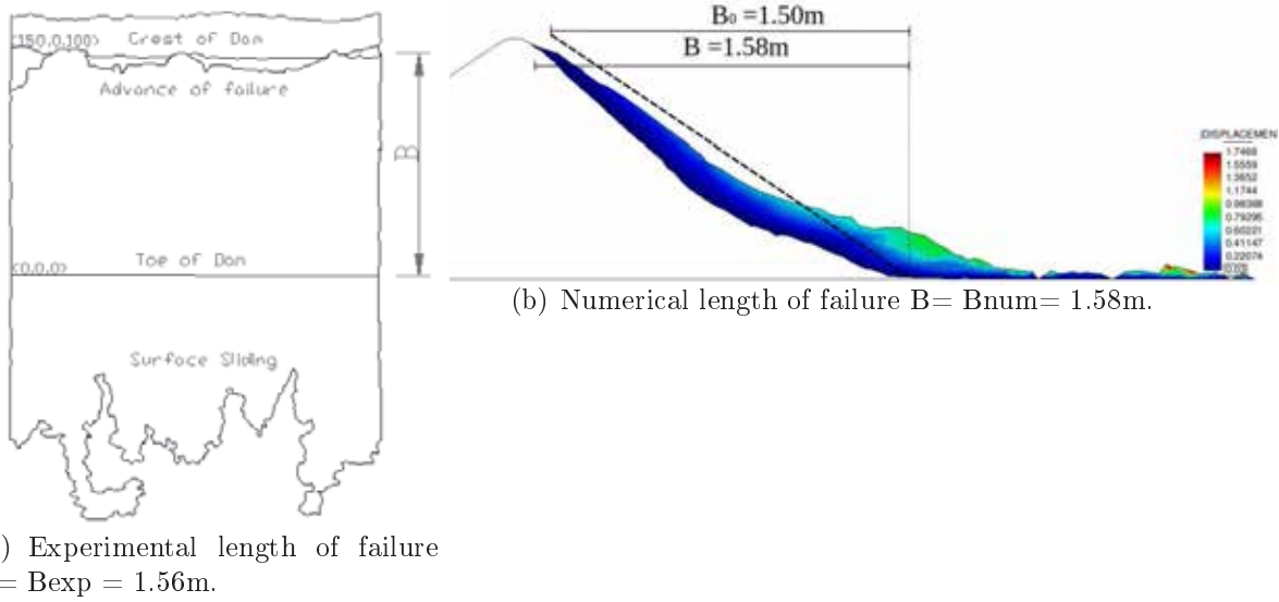
Figure 5.23: Case A23. 2D comparison between experimental and numerical length of failure.
