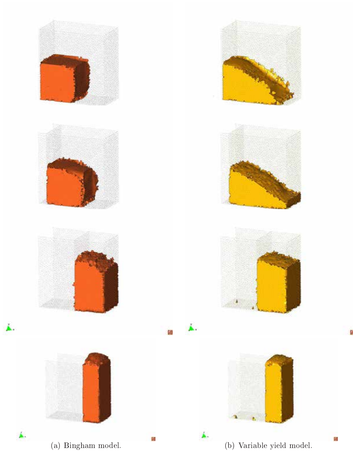
Figure 3.25: 3D pushed slope. Difference between the Bingham and the variable viscosity models in the initial pushing phase.
