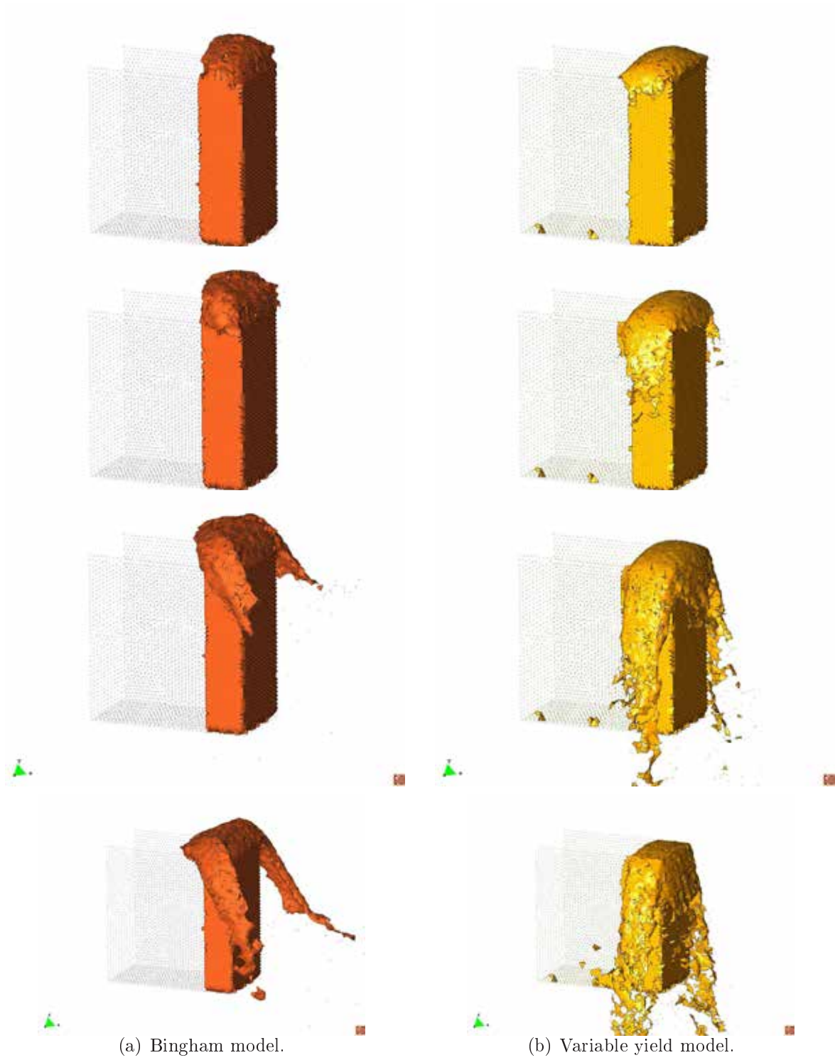
Figure 3.26: 3D pushed slope. Difference between the Bingham and the variable viscosity models in the squeezing phase.
