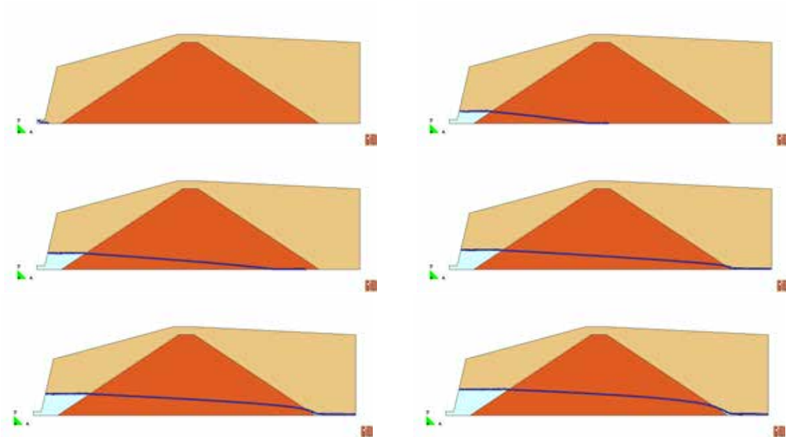
Figure 5.8: Case A1. Evolution of the seepage line in a dam with porosity n = 0.4 and D_{50} = 35mm . Q = 25,46l/s .
