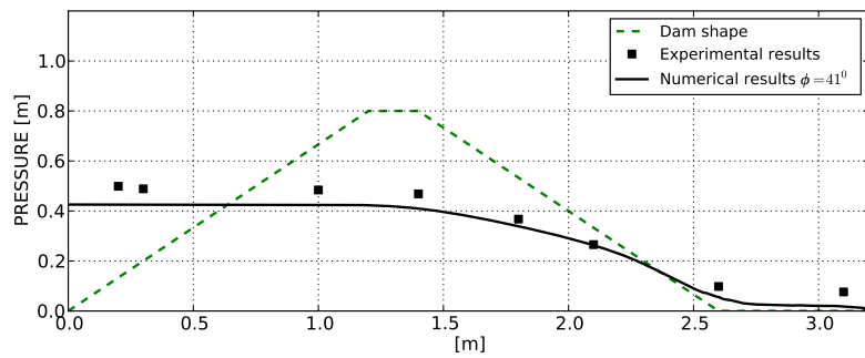
Figure 5.63: Case C22. Bottom pressure distribution at stationary regime for Q = 39.56l/s . Porosity n = 0.4 , D_{50} = 35mm . Numerical and experimental comparison.
