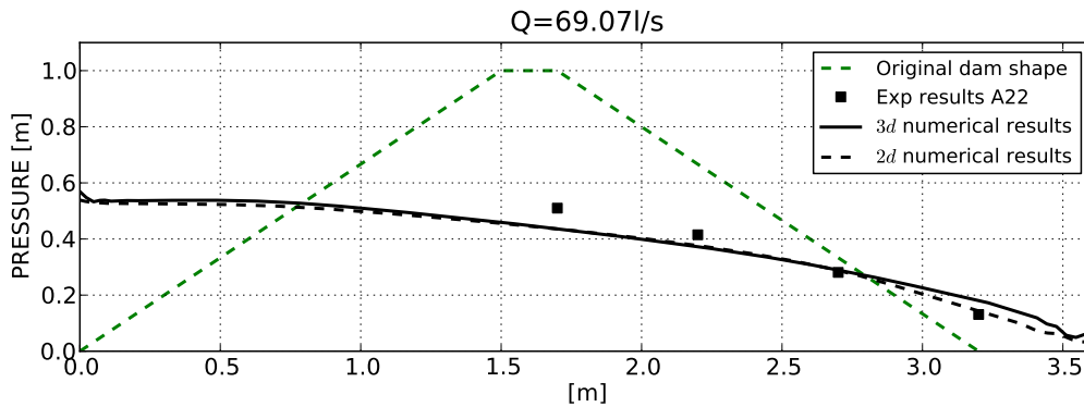
Figure 5.30: Case A22 3D. Bottom pressure distribution at stationary regime for Q = 69.07\text{ l/s} . Porosity n = 0.4 , D_{50} = 35\text{ mm} . 2D and 3D numerical results compared with experimental data points.
