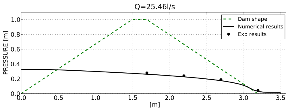
Figure 5.9: Case A1. Bottom pressure distribution at stationary regime for Q = 25,46l/s . Porosity n = 0.4 , D_{50} = 35mm . Numerical and experimental comparison.
