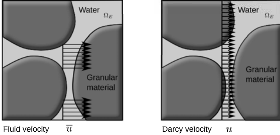
Figure 2.1: Graphical description of fluid velocity \bar{u} (averaged over the empty volume \Omega_E ) and Darcy velocity u (averaged over the total control volume \Omega ).
