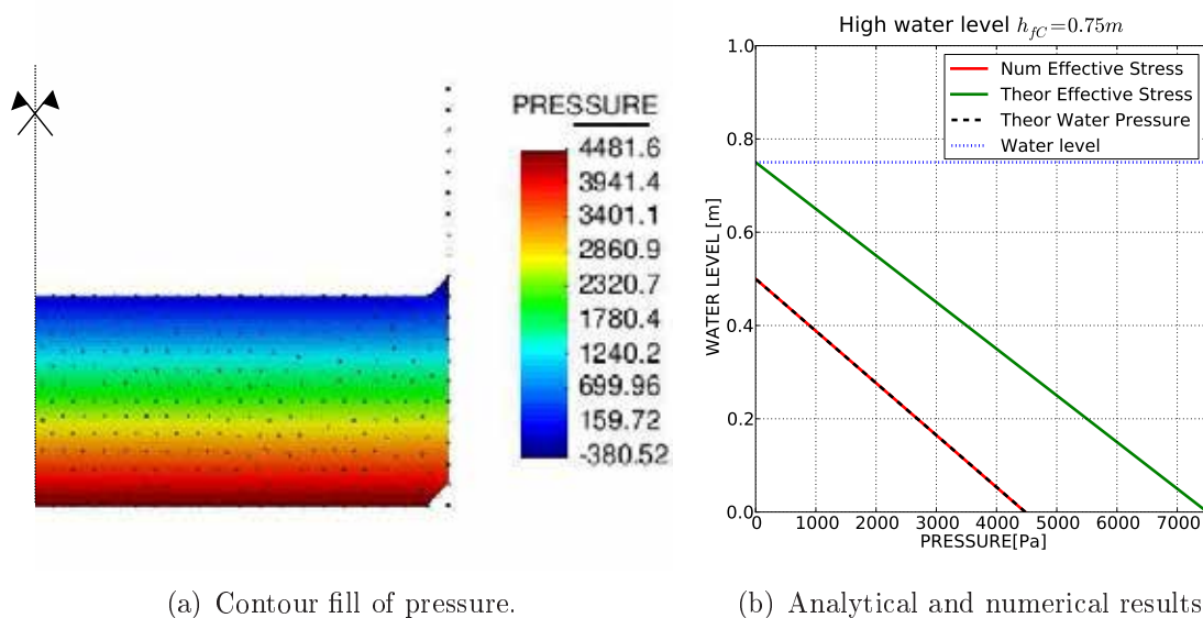
Figure 4.6: Case C. h_{fC} = 0.75m Effective Pressure p'_s .
