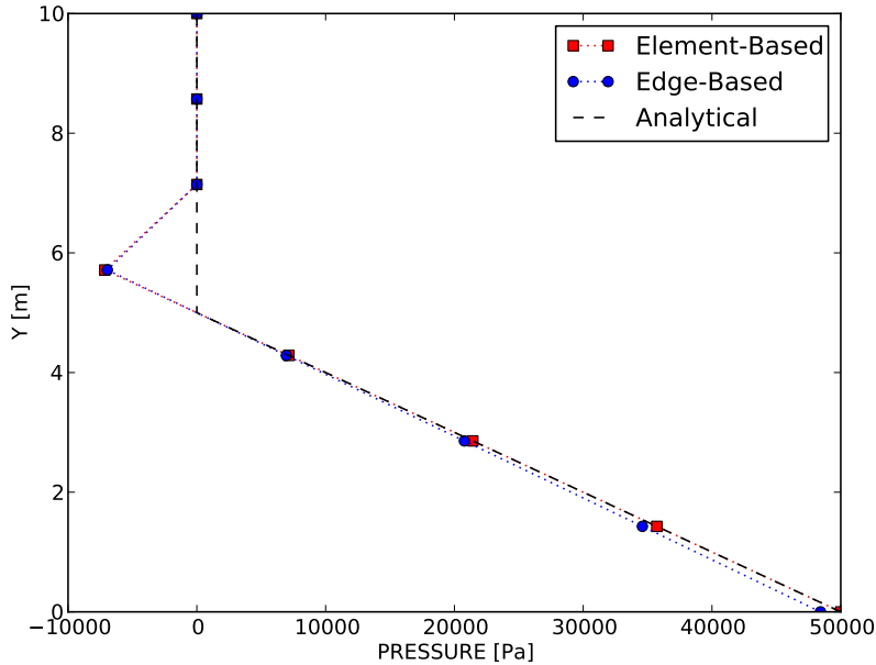
Figure 2.14: Pressure distribution in a vertical section. Comparison between the two algorithms.
