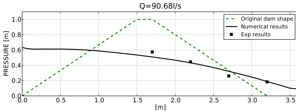
Figure 5.26: Case A23. Bottom pressure distribution at stationary regime for Q = 90.68l/s . Porosity n = 0.4 , D_{50} = 35mm . Numerical and experimental comparison.
