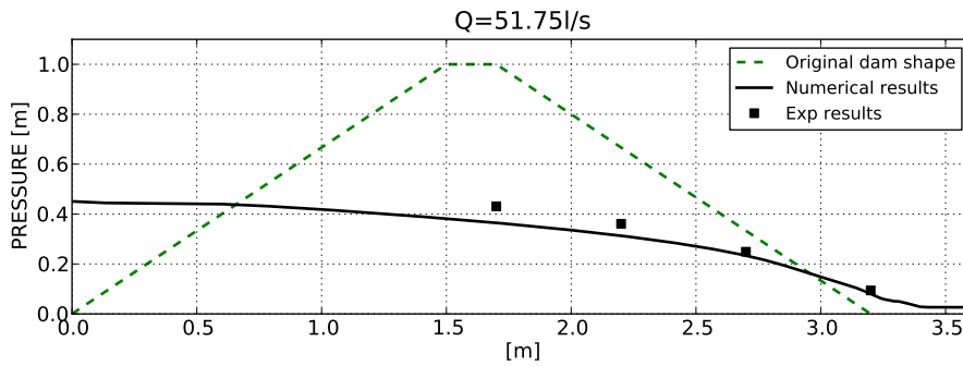
Figure 5.24: Case A21. Bottom pressure distribution at stationary regime for Q = 51.75\text{l/s} . Porosity n = 0.4 , D_{50} = 35\text{mm} . Numerical and experimental comparison.
