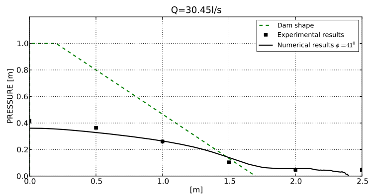
Figure 5.49: Case B22. Bottom pressure distribution at stationary regime for Q = 30.45 \text{ l/s} . Porosity n = 0.4 , D_{50} = 35 \text{ mm} . Numerical and experimental comparison.
