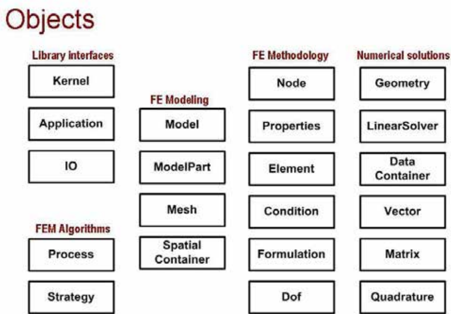
Figure A.1: List of the principal object in Kratos. Image taken from [47].
