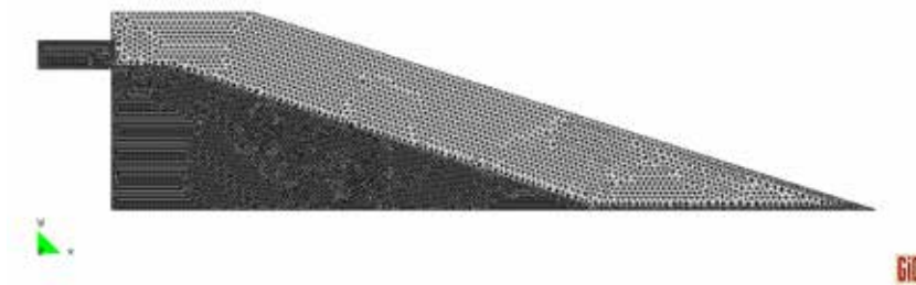
Figure 5.36: Case B1(b-c).Mesh used in the calculation.
