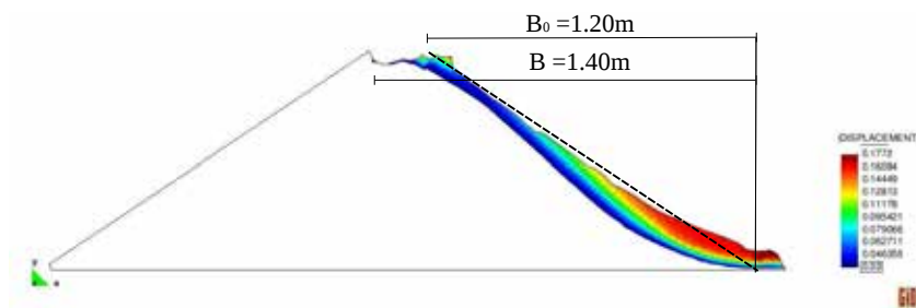
Figure 5.61: Case C23. 2D comparison between experimental and numerical length of failure.
