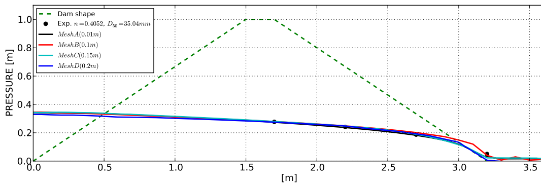
Figure 5.11: Case A1. Influence of the mesh.
