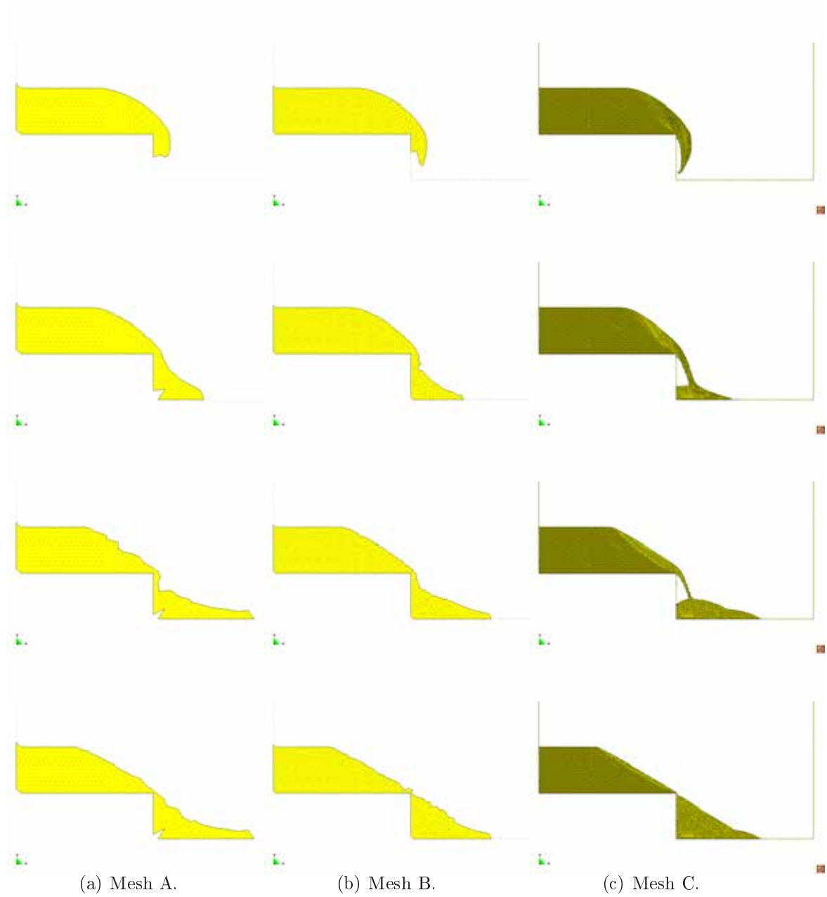
Figure 3.29: Settlements for a granular slope with internal friction angle \phi = 30^\circ for the three different mesh sizes indicated in Figure 3.28.
