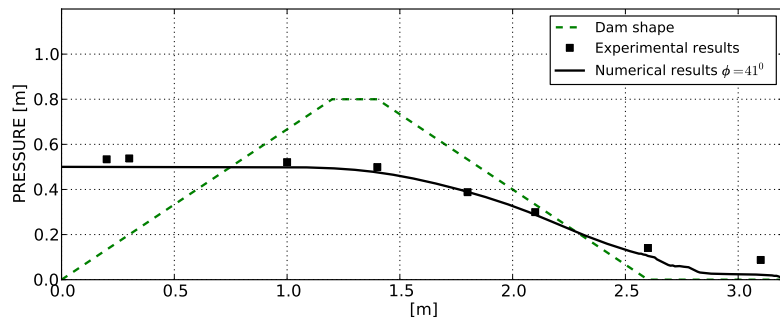
Figure 5.64: Case C23. Bottom pressure distribution at stationary regime for Q = 39.56l/s . Porosity n = 0.4 , D_{50} = 35mm . Numerical and experimental comparison.
