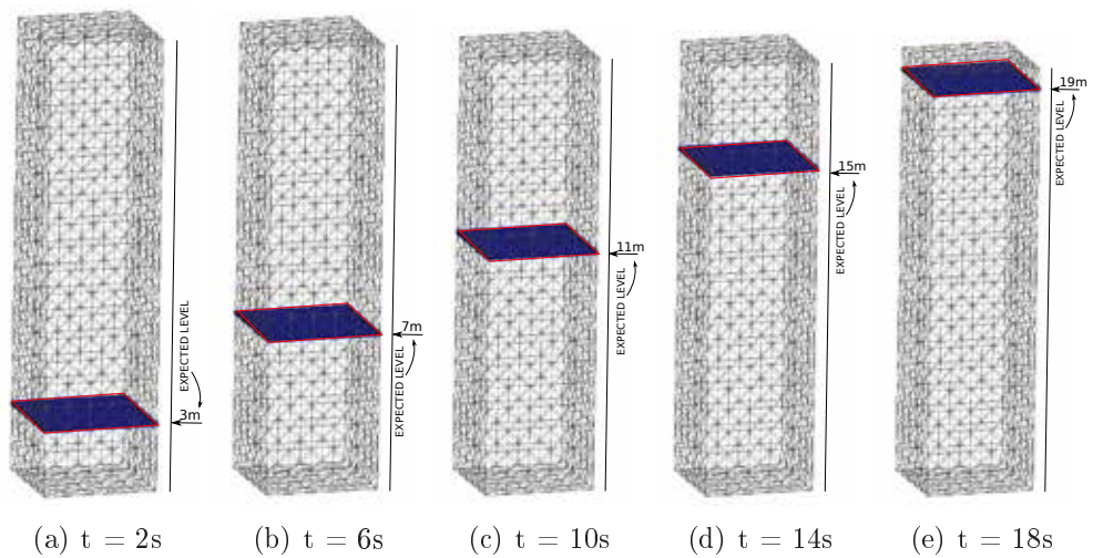
Figure 2.23: 3D vertical column. Structured medium mesh. Evolution of free surface for 1m/s bottom incoming velocity. On the right of each snapshot the expected level is indicated.
