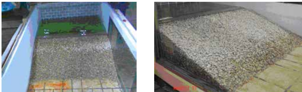
Figure 5.31: Core dam. Experimental setting.
