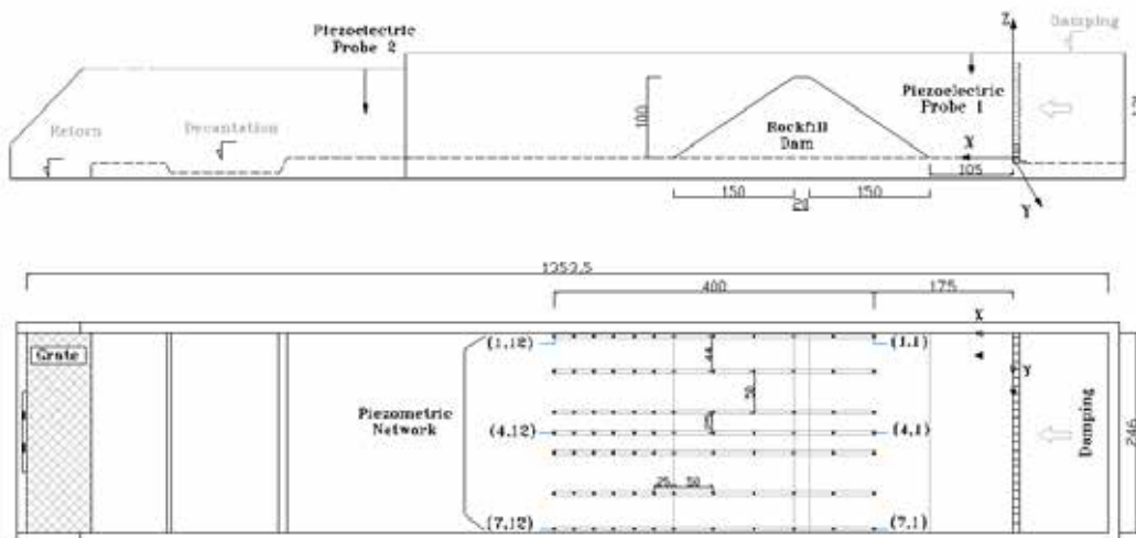
Figure 5.6: Case A. Geometry of the experimental setting and map of the sensors distribution.
