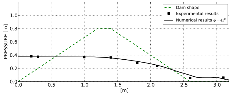
Figure 5.62: Case C21. Bottom pressure distribution at stationary regime for Q = 39.56l/s . Porosity n = 0.4 , D_{50} = 35mm . Numerical and experimental comparison.
