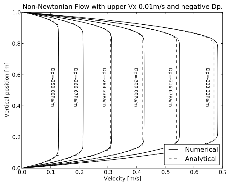
Figure 3.10: Velocity diagrams for different values of a negative gradient of pressure. Upper horizontal velocity 0.01m/s.
