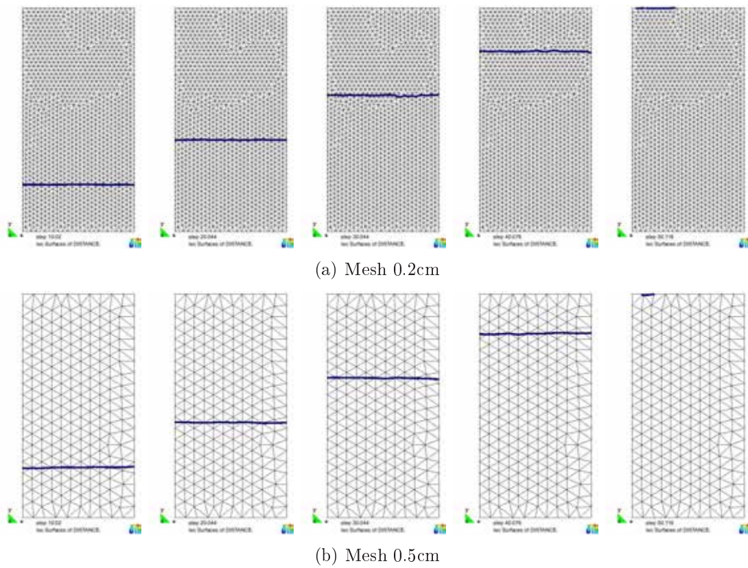
Figure 2.20: 2D Vertical column. Element-based algorithm. Evolution of free surface at 10 – 20 – 30 – 40 – 50 sec.
