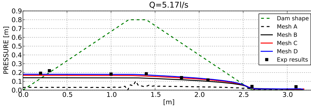
Figure 5.56: Case C. Bottom pressure distribution at stationary regime for Q = 5.17\text{ l/s} . Porosity n = 0.4 , D_{50} = 35\text{ mm} . Numerical and experimental comparison for the different meshes analyzed.
