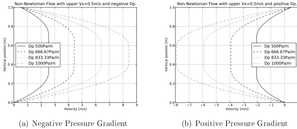
Figure 3.9: Velocity diagrams for different values of the gradient of pressure. Upper horizontal velocity 0.5m/s.
