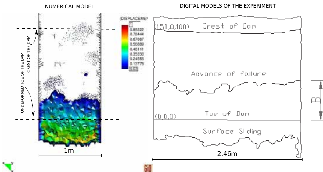
Figure 5.29: Case A22 3D. Numerical and experimental length of failure.
