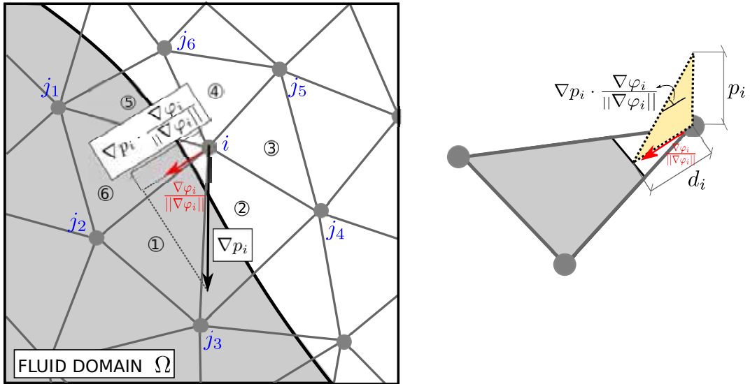
Figure 2.11: Graphical explanation of the evaluation of pressure on the first layer of non fluid nodes in order to respect the incompressibility condition.
