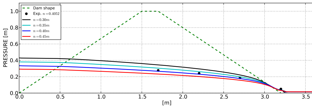
Figure 5.12: Case A1. Pressure head distribution for porosity n = 0.3, 0.35, 0.4 and 0.45 .
