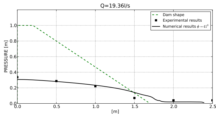
Figure 5.48: Case B21. Bottom pressure distribution at stationary regime for Q = 19.36 \text{ l/s} . Porosity n = 0.4 , D_{50} = 35 \text{ mm} . Numerical and experimental comparison.
