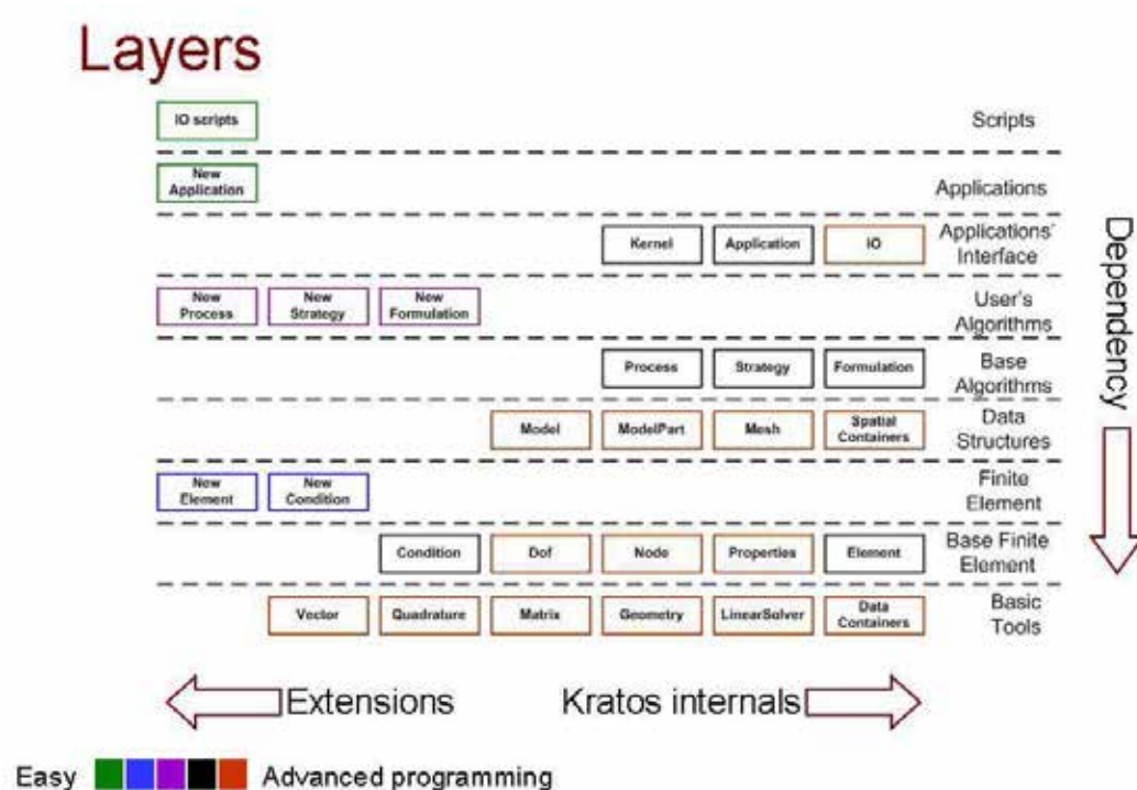
Figure A.2: Graphical summary of the multi.layer design. Image taken from [47].
