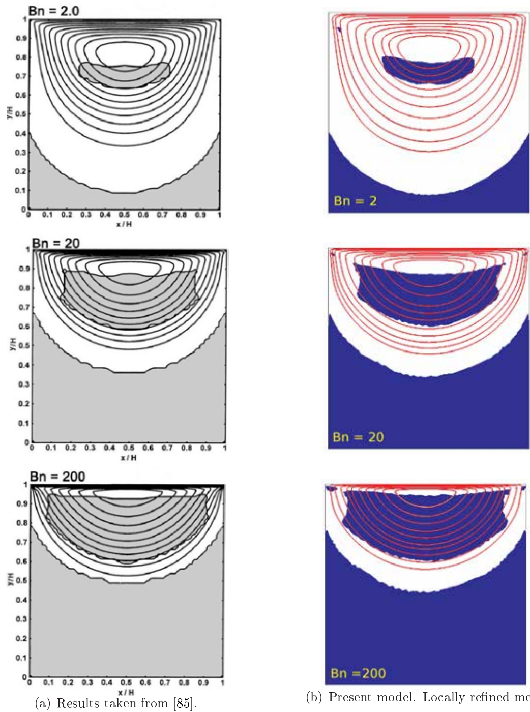
Figure 3.14: Cavity example. Streamlines and progressive evolution of the yielded area (white color) for increasing values of the Bingham number Bn ( Bn = 2, 20 and 200 respectively).
