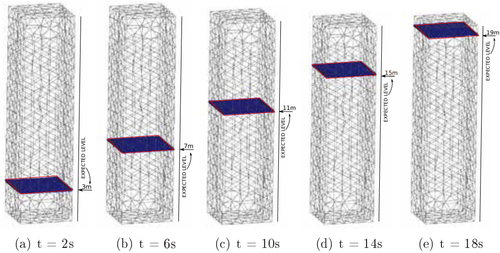
Figure 2.24: 3D vertical column. Unstructured medium mesh. Evolution of free surface for 1m/s bottom incoming velocity. On the right of each snapshot the expected level is indicated.
