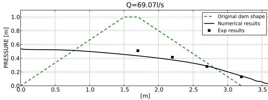
Figure 5.25: Case A22. Bottom pressure distribution at stationary regime for Q = 69.07l/s . Porosity n = 0.4 , D_{50} = 35mm . Numerical and experimental comparison.
