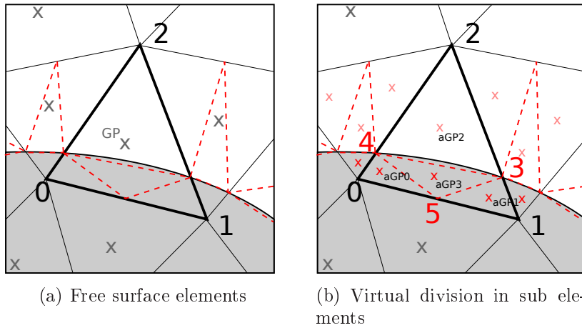
Figure 2.10: Splitting procedure for the elements cut by the free surface.
