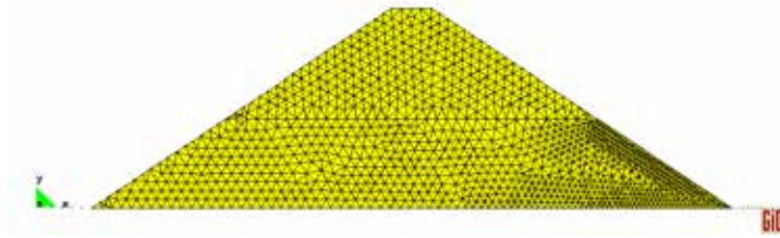
Figure 5.20: Case A2. 2D mesh of the dam model. 3.400 linear triangular elements.
