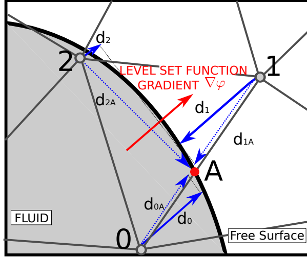
Figure 2.9: Calculation of nodal distances d_i on the nodes i of one element cut by the free surface.
