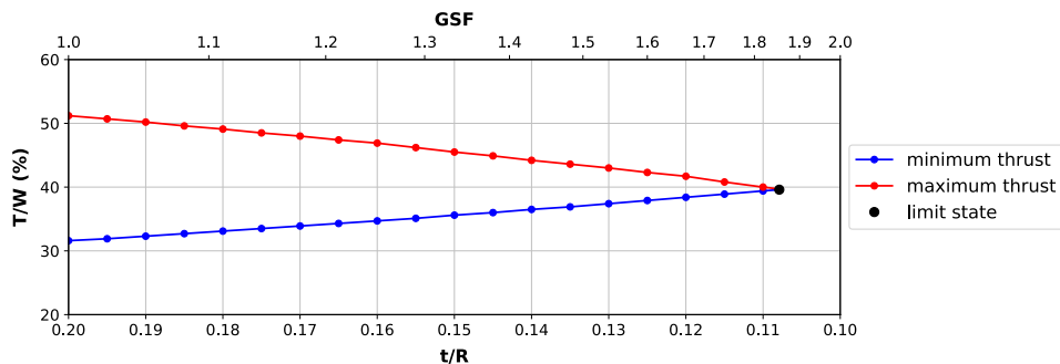
Figure 2. Methodology for deriving the minimum thickness and computing the geometric safety factor (GSF) for the semi-circular arch with t/R=0.20 , resulting in t'/R=0.1079 and \text{GSF}=1.85 .
