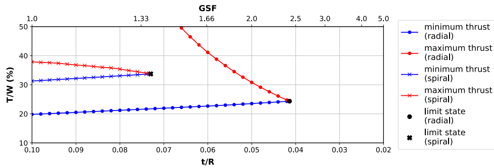
Figure 6. Methodology for deriving the minimum thickness and computing the GSF for the dome ( t/R=0.10 ), the radial diagram resulted in t'/R=0.036 and GSF_1=2.42 and the spiral diagram in t'/R=0.073 and GSF_2=1.37 . (Values of T/W higher than 50% not shown for clarity).
