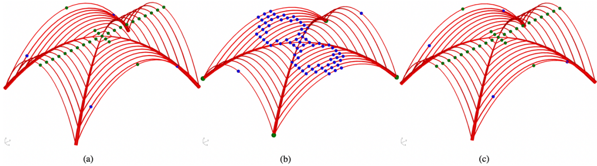
Figure 8. Cross form diagram: minimum (a) and maximum (b) thrust result for t/R=0.10 and thrust for minimum thickness (c) achieved with grid diagram with t'/R=0.061 . Maximum forces in plots are 203; 226; and 213kN.
