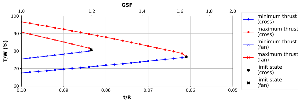
Figure 10. Methodology for deriving the minimum thickness and computing the GSF for the cross vault, cross diagram resulted in t/R=0.061 and GSF_1=1.64 and the fan diagram in t/R=0.084 and GSF_2=1.20 .
