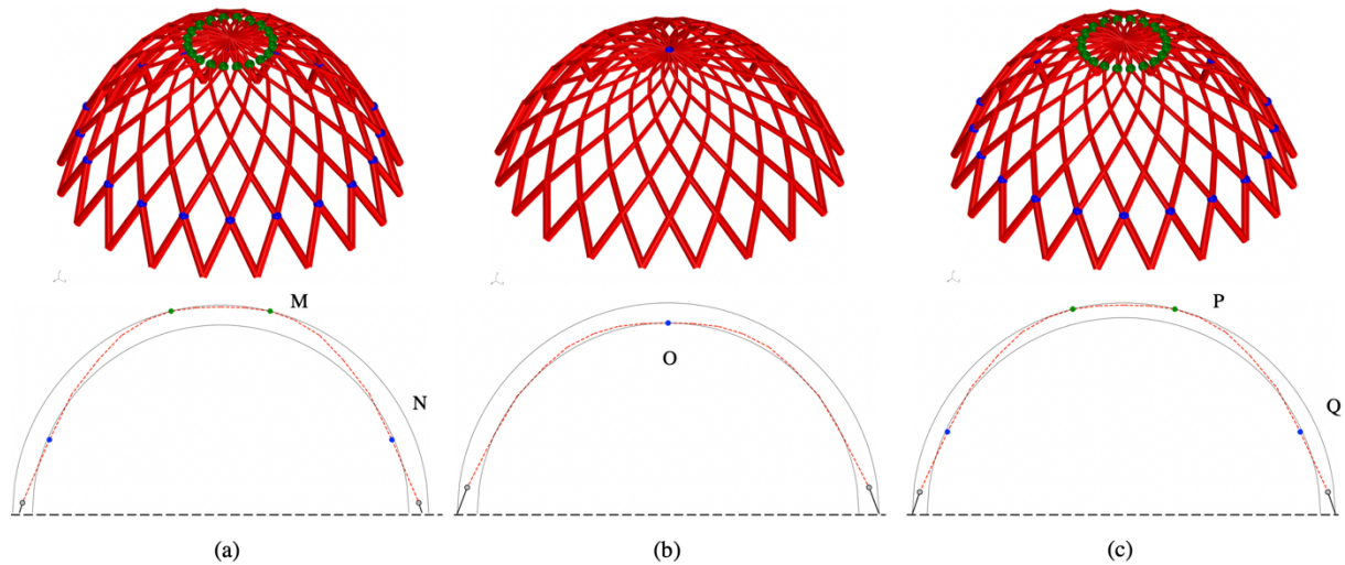
Figure 5. Minimum (a) and maximum (b) thrust solutions for the dome with the spiral diagram with t/R=0.10 and with limit thickness (c) achieved ( t/R=0.073 ). Maximum forces in the plots are 33; 35; and 34kN.
