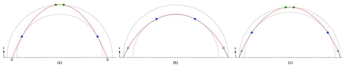
Figure 1: Solutions of minimum (a) and maximum (b) thrust for the semi-circular arch with t/R=0.20 and thrust for the minimum thickness (c) calculated as t'/R=0.1079 after incremental reduction of the thickness.
