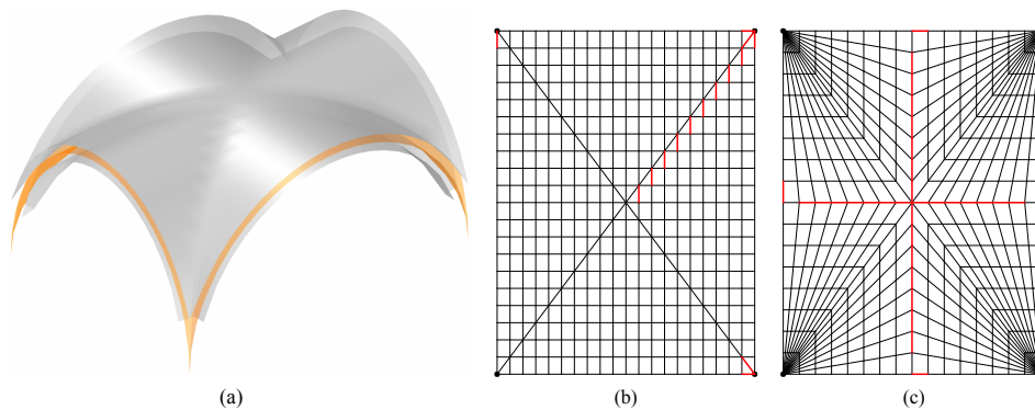
Figure 7. (a) Geometry considered for the rectangular cross-vault ( t/R=0.10 ), showing base surface (orange), intrados and extrados; (b) cross form diagram and; (c) fan form diagram showing the independent edges.
