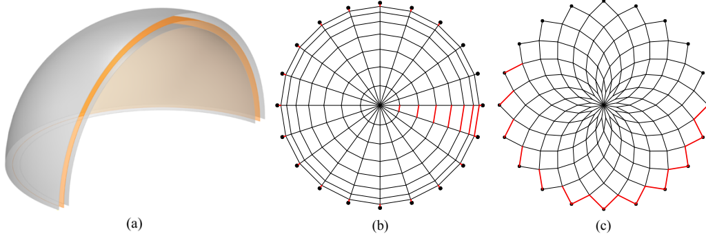
Figure 3. (a) Geometry of the dome with t/R=0.10 , showing base surface (orange), intrados and extrados (cut to enhance visualisation); (b) radial form diagram and; (c) spiral form diagram showing independent edges.
