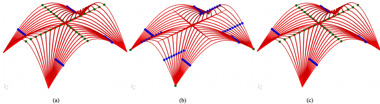
Figure 9. Cross form diagram: minimum (a) and maximum (b) thrust result for t/R=0.10 and thrust for minimum thickness (c) achieved with fan diagram with t'/R=0.084 . Maximum forces in plots are 68; 84; and 72kN.
