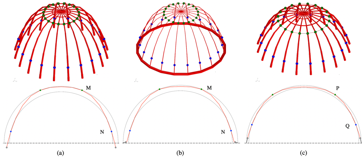
Figure 4. Minimum (a) and maximum (b) thrust solutions for the dome with the radial diagram with t/R=0.10 and with limit thickness (c) achieved ( t'/R=0.041 ). Maximum forces in the plots are 70; 1000; and 72kN.
