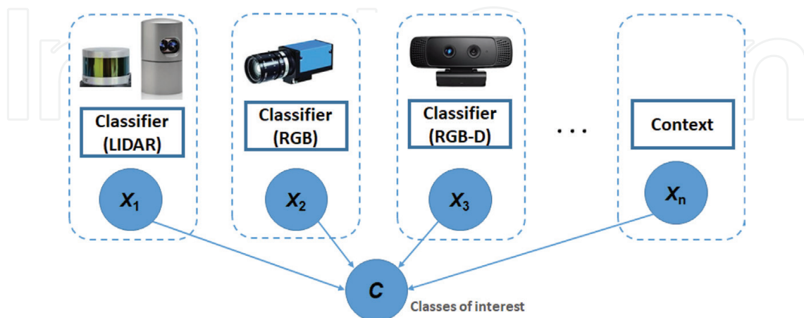
Figure 1. Topology of a BN where all the parent nodes \{X_1, X_2, \dots, X_n\} contribute to a common effect, which is the set of classes (node C ) of interest in a given robotic domain.
