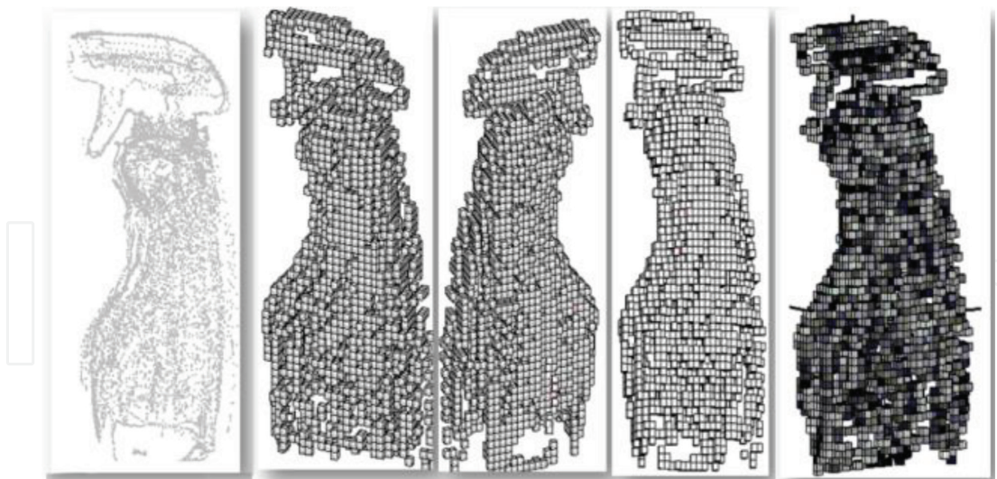
Figure 6. Object shape representation by in-hand exploration of a spray bottle. The first image (left to right) is the raw data (point cloud), next three images are different views of the voxels representation of the object shape, and the last image is the occupancy representation of the cells, the darkest ones represent the lower probabilities (less explored regions).
