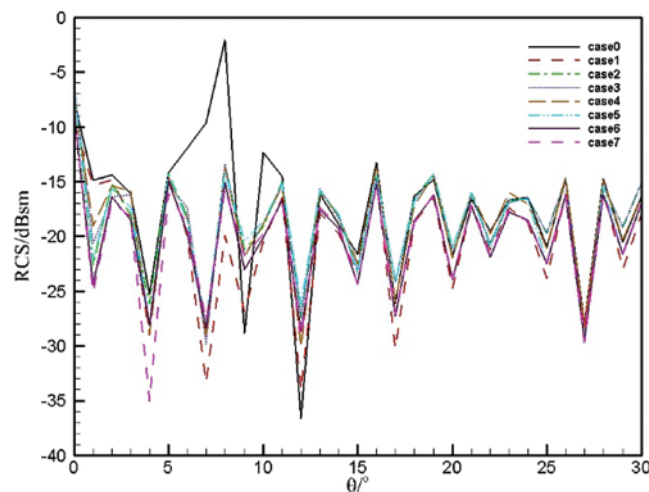
Figure 7: RCS curves of the S-shaped inlet in the horizontal polarization in the yaw plane
