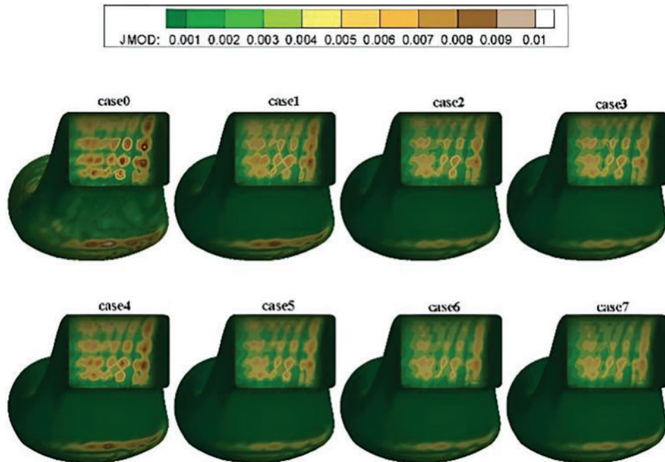
Figure 9: Induced current distribution at in the vertical polarization \theta = 8^\circ (unit: \text{mA/m}^2 )
