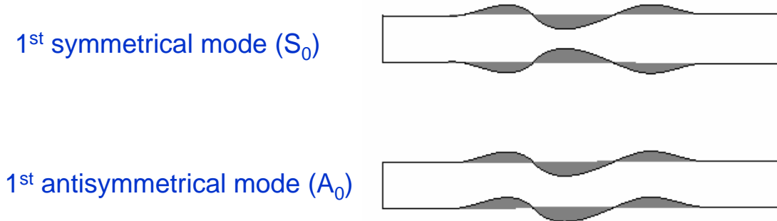
Figure 2.1: Example of S_0 and A_0 modes
