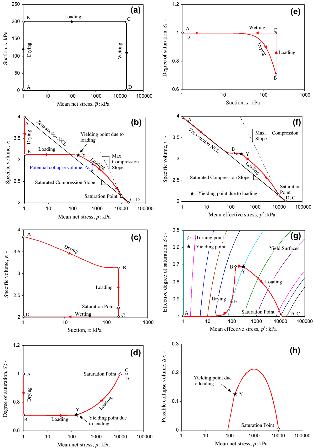
Fig. 4. Drying–loading (isotropic, to fully saturated) path and calculated responses: (a) s vs. \bar{p} , (b) v vs. \bar{p} , (c) v vs. s , (d) S_r vs. \bar{p} , (e) S_r vs. s , (f) v vs. p' , (g) S_{e'} vs. p' , (h) \Delta v vs. \bar{p} .
