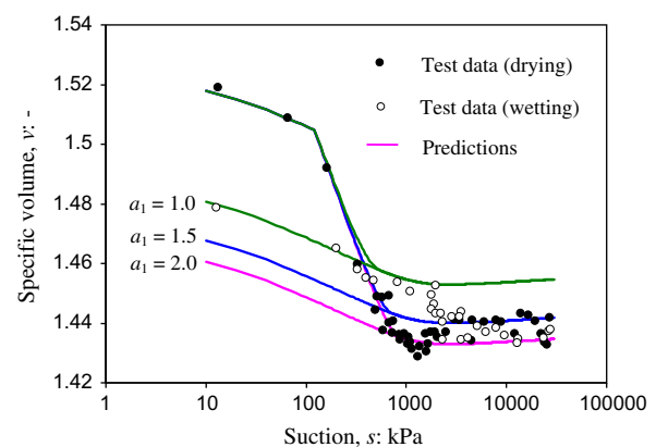
Fig. 7. Drying and wetting test results and model simulations (data after data after [5]).
