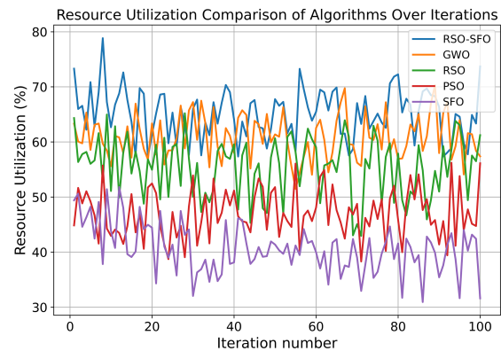
Figure 4: Resource utilization comparison of algorithms over iterations
