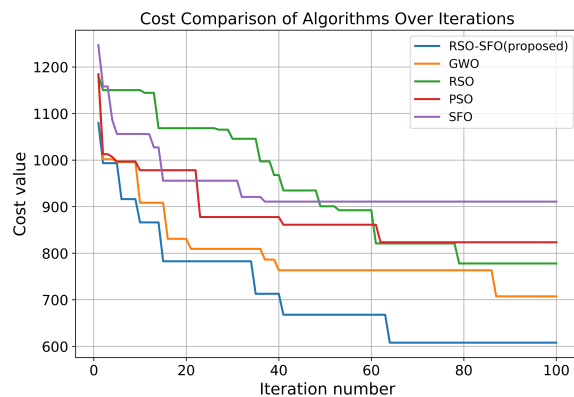
Figure 5: Cost comparison of algorithms over iterations
