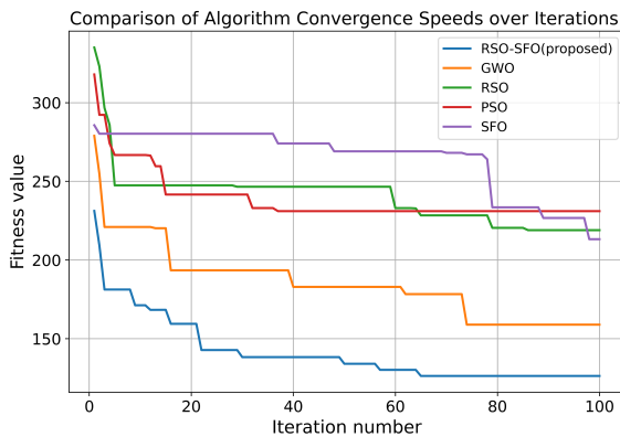
Figure 3: Comparison of algorithm convergence speeds
