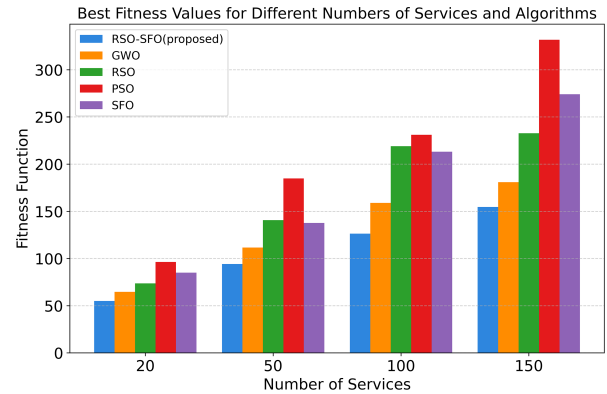
Figure 8: Best fitness values for different numbers of services and algorithms
