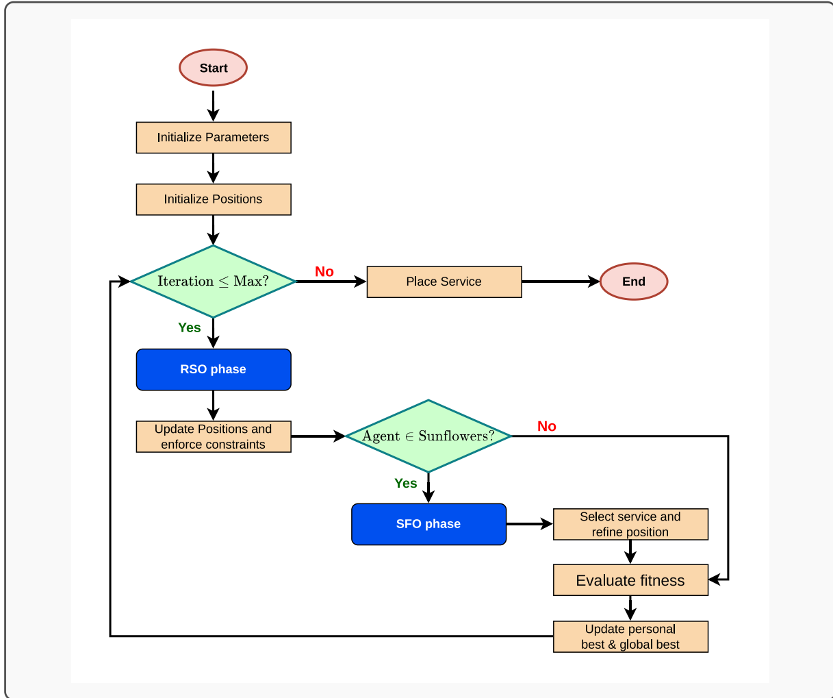
Figure 2: Unified RSO–SFO hybrid optimization framework
