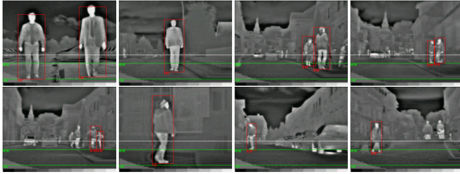
Fig. 7. Results of pedestrian detection in different situations: with complex or simple scenario or with one or more pedestrians. The distance (meters) is displayed below the boxes. The two horizontal green lines encode the range in which pedestrians are searched for, while the horizontal white line encodes the horizon.
