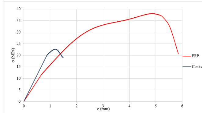
Figure 5. Comparison between FRP and pure concrete specimens.
