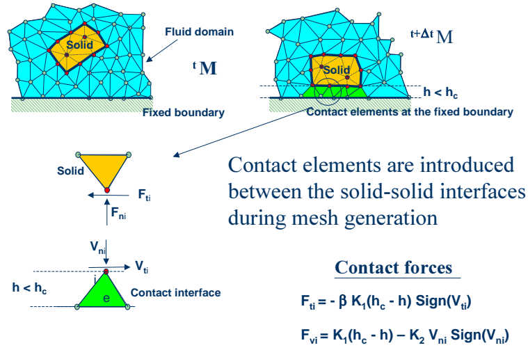
Figure 9: Contact conditions at a solid-solid interface
