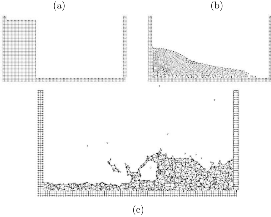
Figure 4: Breakage of a water column. (a) Discretization of the fluid domain and the solid walls. Boundary nodes are marked with circles. (b) and (c) Mesh in the fluid and solid domains at two different times.
