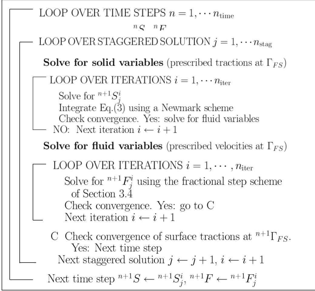
Box 1. Staggered scheme for the FSI problem
