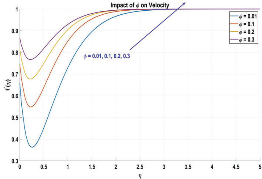
Figure 1: Volume fraction of nanoparticles vs. velocity of nanofluid
