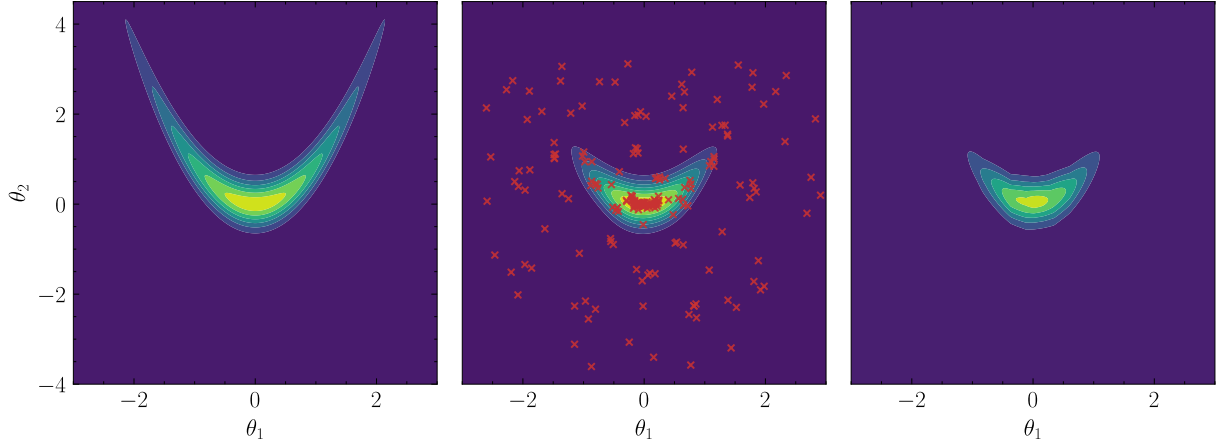
Figure 2: From left to right: True posterior, surrogate GP posterior with training sample locations, and the normalizing flow approximation of the surrogate GP posterior.
