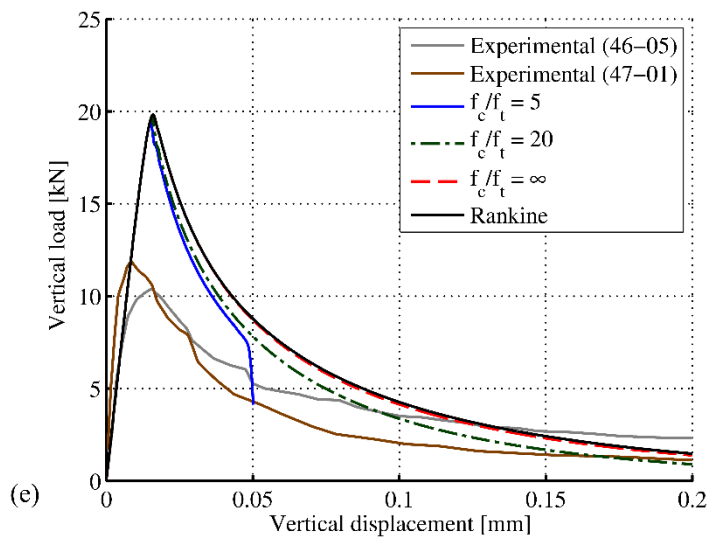
Figure 12. Load-path 4b: contour of the selected crack propagation direction in the damaged elements for Mohr-Coulomb's criterion and f_c/f_t = 5 (a), f_c/f_t = 20 (b), f_c/f_t = \infty (c); for Rankine's criterion and f_c/f_t = 20 (d) and load vs displacement ( P-\delta ) for different compressive to tensile strength ratios (e).
