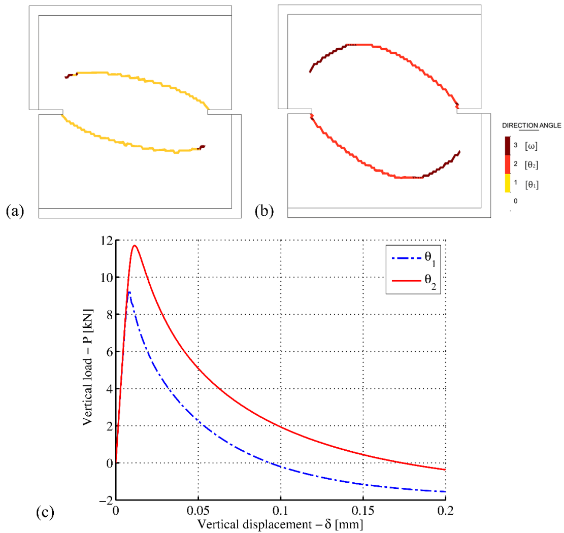
Figure 13. Load-path 4c for f_c/f_t = 20 : contour of the selected crack propagation direction in the damaged elements: case \theta_1 (a), case \theta_2 (b) and load vs displacement ( P - \delta ) for the two possible fracture planes (c).
