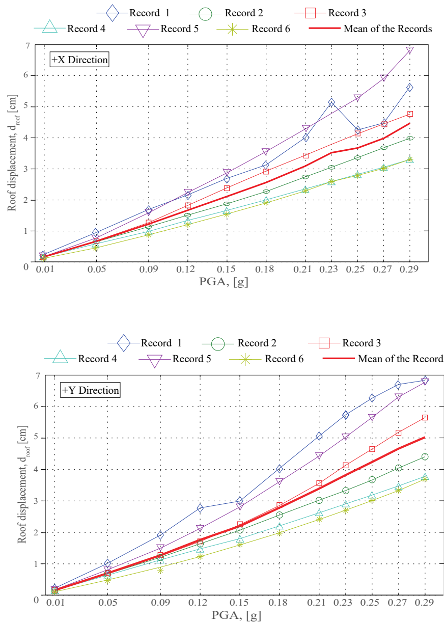
Fig. 7 IDA results for the URM building for both directions. Relationship between PGA and d_{\text{roof}}
