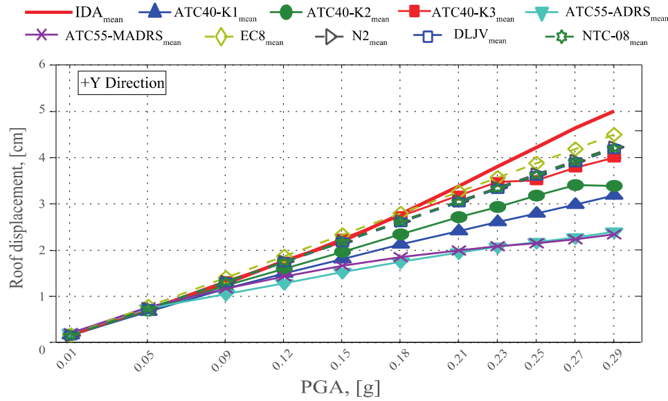
Fig. 10 Comparison between NSPs and IDAs mean results for +Y direction.
