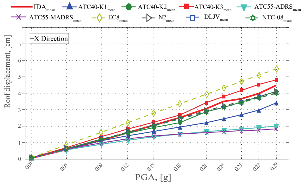
Fig. 9 Comparison between NSPs and IDAs mean results for +X direction.
