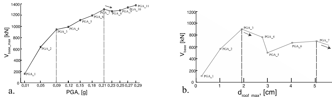
Fig. 13 Selection of the yielding and ultimate points for the IDA. Ground motion 1, +Y direction.
