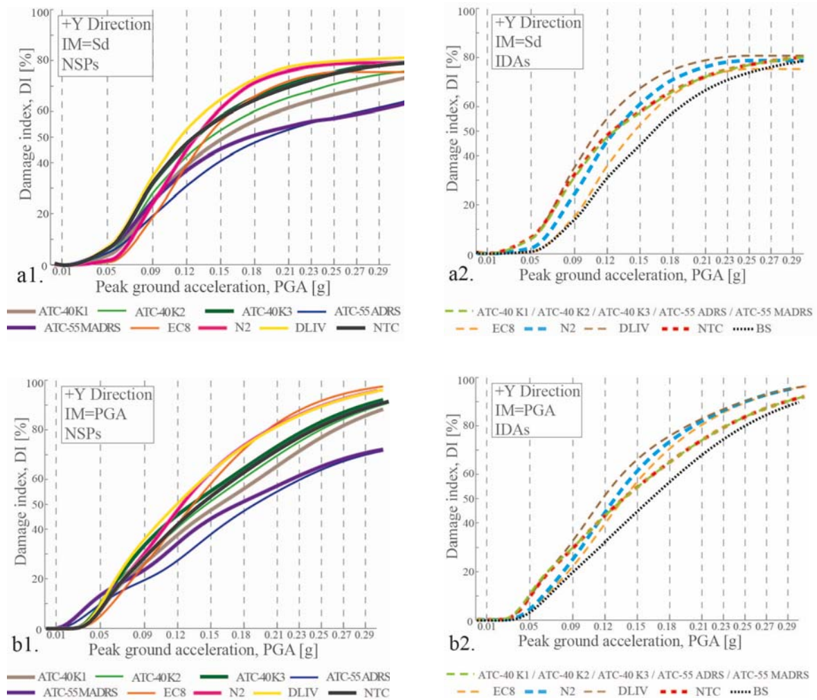
Fig. 15 Comparison of damage curves (+Y direction). a1)NSPs damage curves - RISK-UE methodology; a2)IDAs damage curves - RISK-UE methodology; b1)NSPs damage curves - MSA methodology; b2)IDAs damage curves – MSA methodology. (Legend: ATC-40 Ki: ATC 40 procedure; ATC-55 (ADRS and MADRS): ATC-55 procedure; EC8: Eurocode 8; N2: method N2; DLIV: De Luca, Iervolino and Vamvatsikos procedure (De Luca et al. 2011); NTC: Norme Tecniche delle Costruzioni -Italian Construction Code- (NTC-08 2008); BS: IDA damage curve based on shear base time history).
