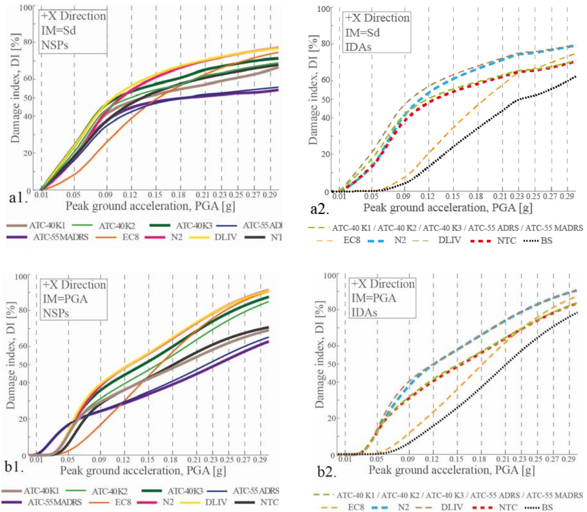
Fig. 14 Comparison of damage curves (+X direction). a1)NSPs damage curves - RISK-UE methodology; a2)IDAs damage curves - RISK-UE methodology; b1)NSPs damage curves - MSA methodology; b2)IDAs damage curves – MSA methodology. (Legend: ATC-40 Ki: ATC 40 procedure; ATC-55 (ADRS and MADRS): ATC-55 procedure; EC8: Eurocode 8; N2: method N2; DLIV: De Luca, Iervolino and Vamvatsikos procedure (De Luca et al. 2011); NTC: Norme Tecniche delle Costruzioni -Italian Construction Code- (NTC-08 2008); BS: IDA damage curve based on shear base time history).
