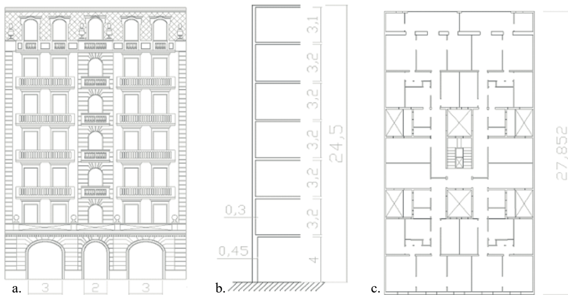
Fig. 3 The analyzed building. Architectural floor plans a) Façade; b) Side elevation; c) Intermediate floor plan [dimensions are in m]
