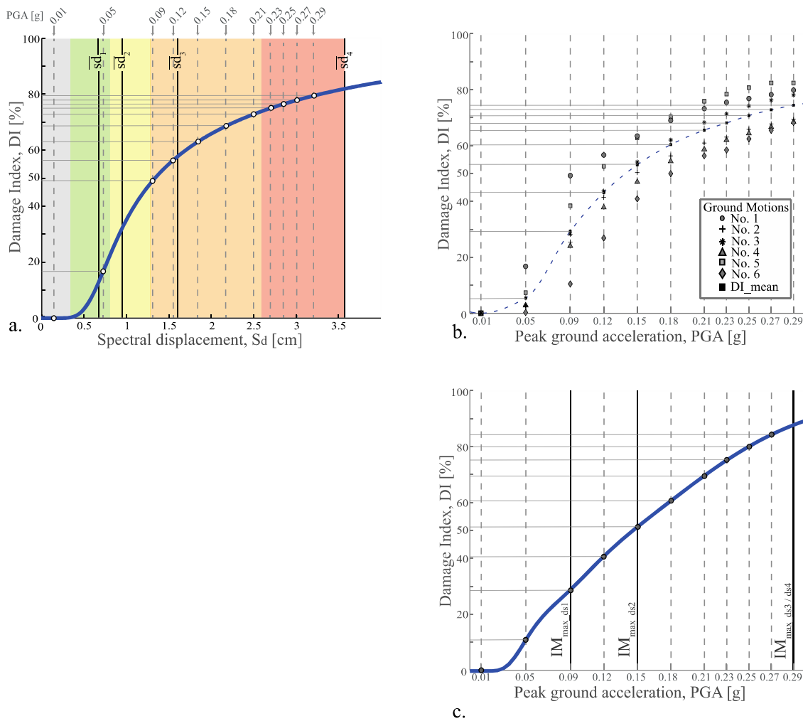
Fig. 12 Vulnerability curves for the example method (ATC-40 procedure with an hysteretic factor K2). a) ( S_d vs DI ) vulnerability curve for one ground motion, IM=S_d ; b) Mean ( PGA vs DI ) damage curve for the six ground motions, IM=S_d ; c) ( PGA vs DI ) damage curve for the six ground motions, IM=PGA .
