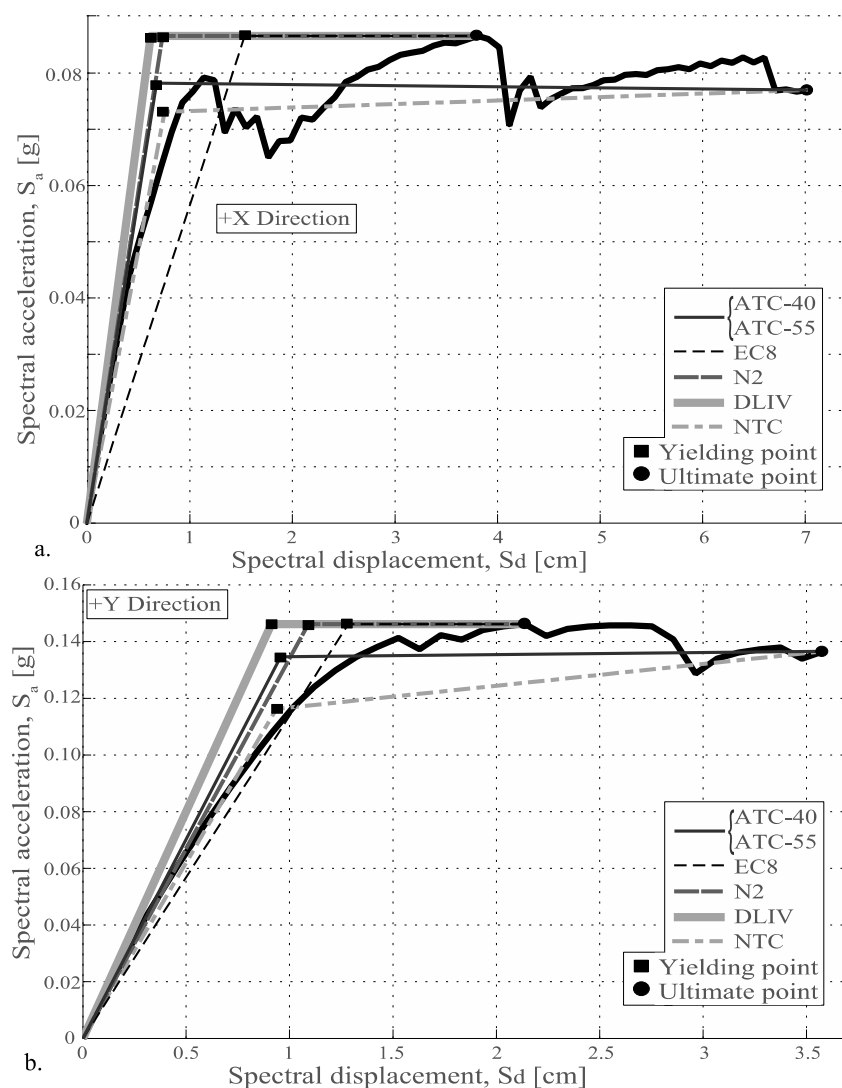
Fig. 8 Bilinear representation, in acceleration-displacement format, of the capacity curve corresponding to the different NSPs. a) +X direction; b) +Y direction.
