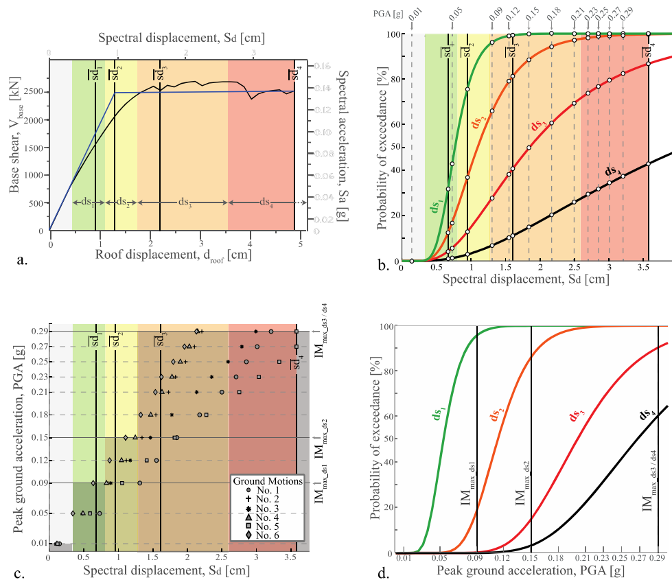
Fig. 11 Damage states and fragility curves for the example method (ATC-40 procedure with hysteretic factor K2). a) Bilinear representation and damage states; b) (S_d vs P(ds_i)) fragility curves for one ground motion, IM=S_d ; c) MSA procedure. Spectral displacements for each analyzed PGA for the six ground motions; d) MSA procedure. Fragility curves ( PGA vs P(ds_i) ), IM=PGA .
