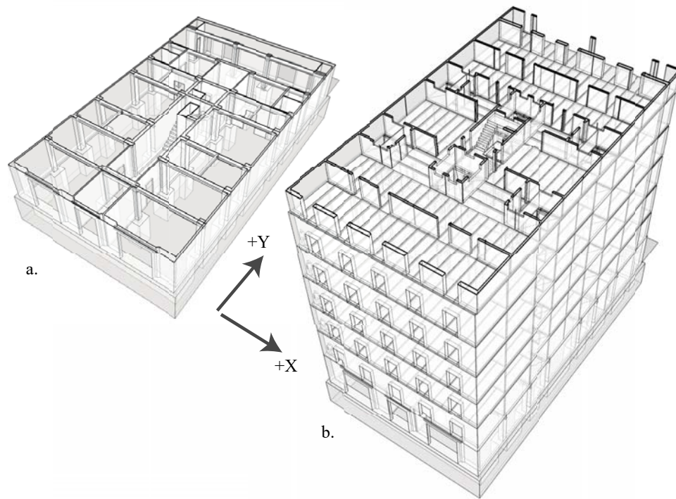
Fig. 4 The analyzed building and the axis the analysis. a) base level; b) upper levels
