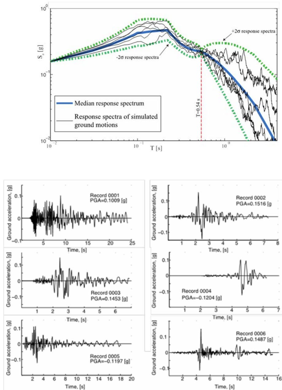
Fig. 6 Record selection according to the conditional spectrum approach with the 5% damped response spectrum for Soil Zone II of Barcelona as target spectrum.
