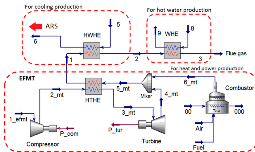
Figure 6. Diagram of the simulation model for the CCHP plant in Aspen Hysys V8.4.
