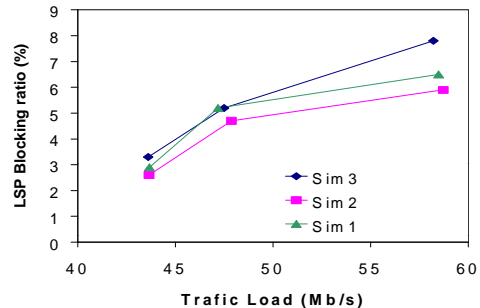
Fig. 6. LSP Blocking Ratio due the impossibility of finding a LSP with the required Bw in the ND3
