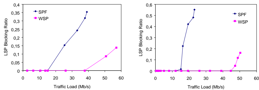
Fig. 5. LSP Blocking Ratio for audio and video traffic load
