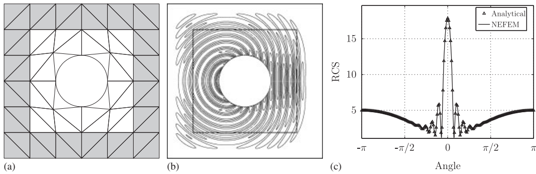
Figure 16. Scattering by a perfect conductor circle: (a) computational mesh with a 2\lambda thick PML; (b) transverse scattered field for a NEFEM solution with p=10 ; and (c) RCS.
