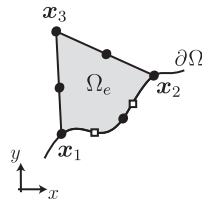
Figure 5. Triangle with a curved edge containing changes of NURBS definition (marked with □).
