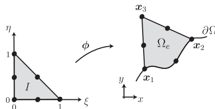
Figure 3. Exact mapping between the reference element I with local coordinates \xi , and the physical subdomain \Omega_e with Cartesian coordinates x .
