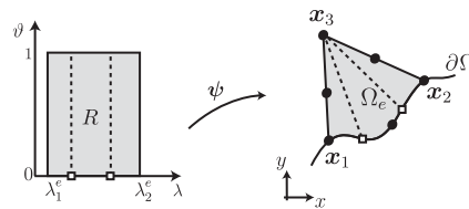
Figure 7. Numerical integration for 2D NEFEM: subdivision of the rectangle R = [\lambda_1^c, \lambda_2^c] \times [0, 1] to design a numerical quadrature taking into account changes of NURBS parametrization C(\lambda) at points marked with □.
