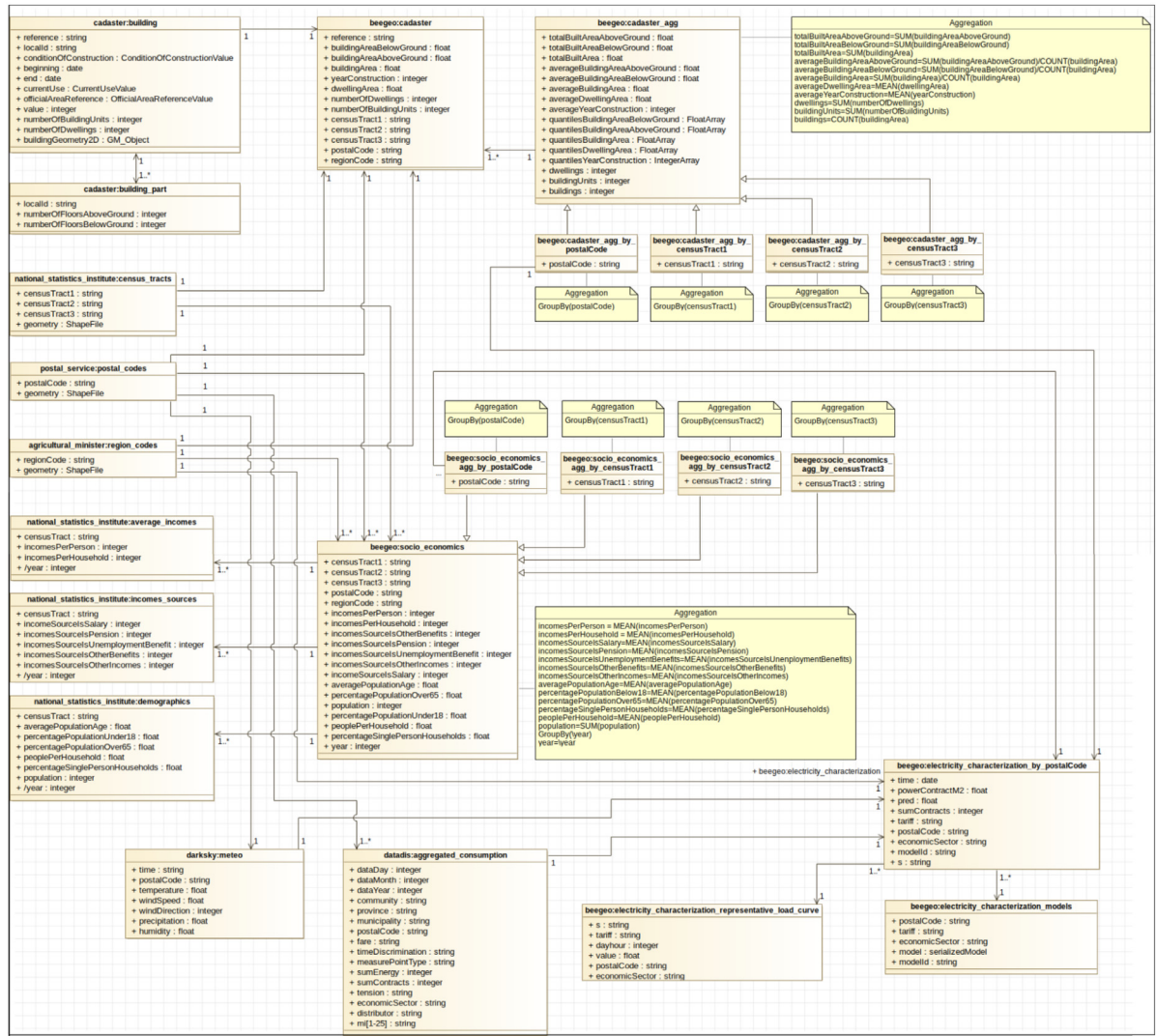
Fig. 2. UML of the used data model.
