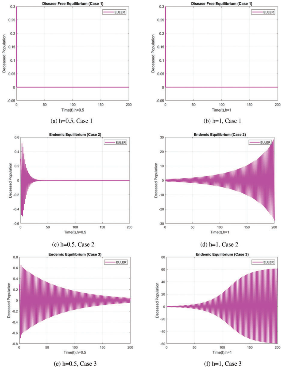
Figure 3: Deceased population at various step sizes using the forward Euler approach
