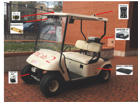
FIGURE 4: iCab with sensors.
