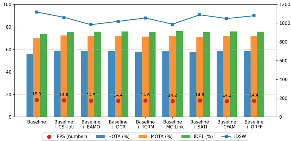
Figure 3: Ablation study: individual component performance on the MOT20 validation set
