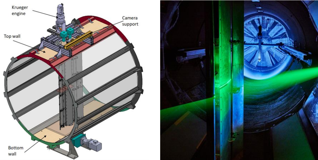
Figure 2: The ONERA wind tunnel set-up
