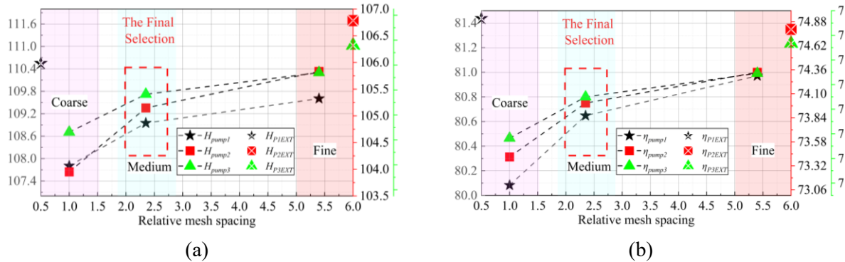
Figure 3: Grid dependence check: (a) Head H ; (b) Efficiency \eta .
