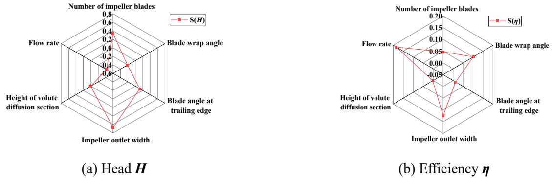
Figure 7: Sensitivity parameter S radar chart.
