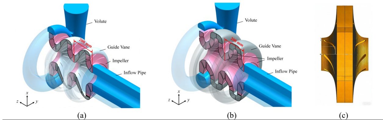
Figure 2: Centrifugal pump model: (a) Traditional channel design (Pump 1); (b) New channel design (Pump 2); (c) Double suction centrifugal pump impeller model (Pump 3).
