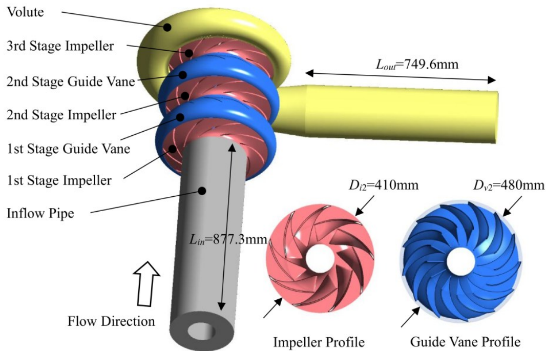
Figure 1: Three stage centrifugal pump model.
