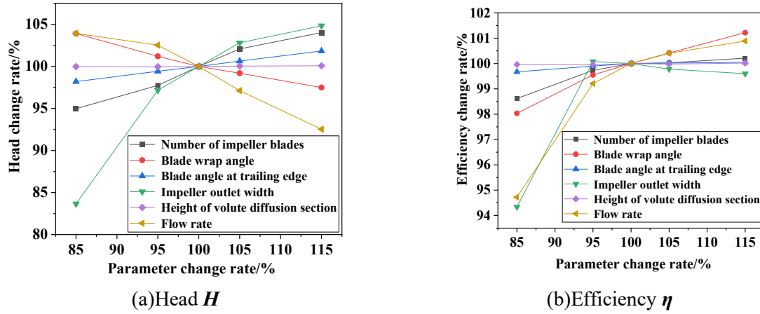
Figure 6: Curve of head and efficiency change rate versus variation law of various parameters.
