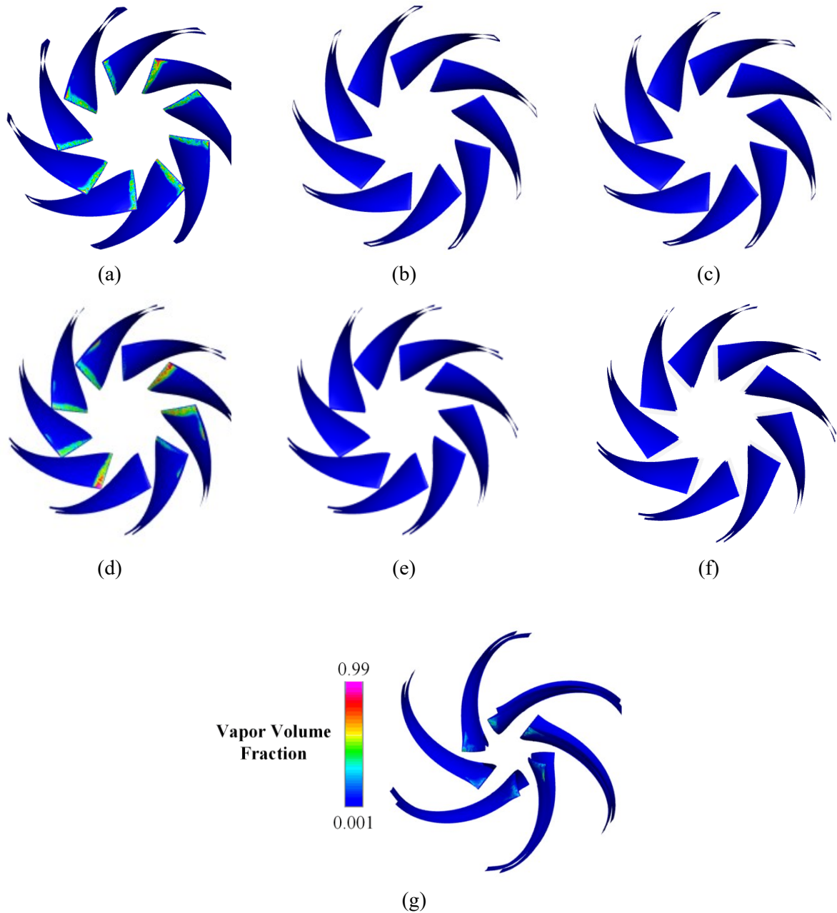
Figure 5: Distribution diagram of impeller air bubbles: (a) 1st stage blade of pump 1; (b) 2nd stage blade of pump 1; (c) 3rd stage blade of pump 1; (d) 1st stage blade of pump 2; (e) 2nd stage blade of pump 2; (f) 3rd stage blade of pump 2; (g) blade of pump 3.
