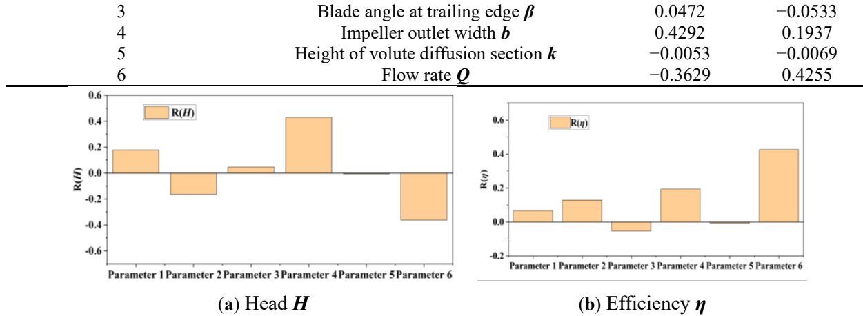
Figure 8: Comparative analysis chart of r results for LHS-PRCC.
