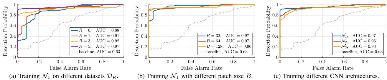
Fig. 2: ROC curves obtained with the proposed solutions: (a) network \mathcal{N}_1 for different numbers R of training B-scans from real acquisitions; (b) network \mathcal{N}_1 for different patch sizes B ; (c) different network configurations \mathcal{N}_1 , \mathcal{N}_2 and \mathcal{N}_3 , fixing B = 64 and R = 5 .
