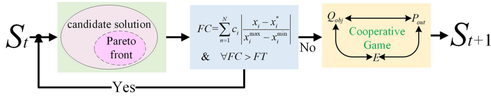
Figure 5: Dynamic decision-variable search strategy
