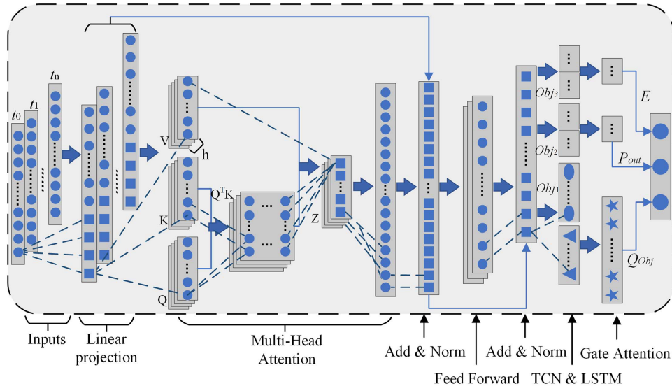
Figure 4: Linformer-TCN-LSTM model
