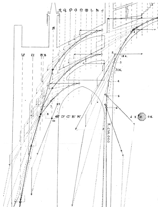
Fig. 11. Rubió's (1912) application of graphic statics to analyze the stability of Mallorca Cathedral (detail).
