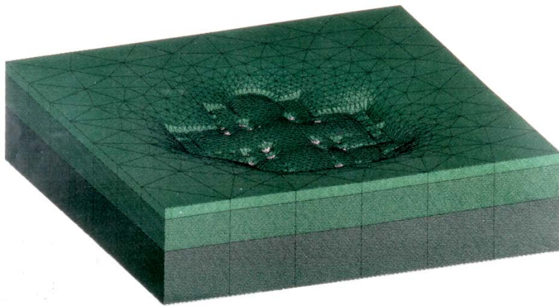
Fig. 2: The finite element model of the St. Mark's Basilica: Top: global discretization; Bottom: soil foundation discretization including deformation (Mola and Vitaliani 1995).
