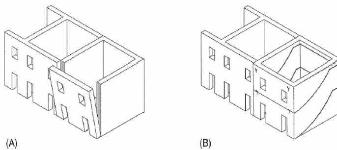
Fig. 12. Failure modes for buildings with no ties (a) and with ties anchoring the facade to lateral walls (Carocci, 2001).
