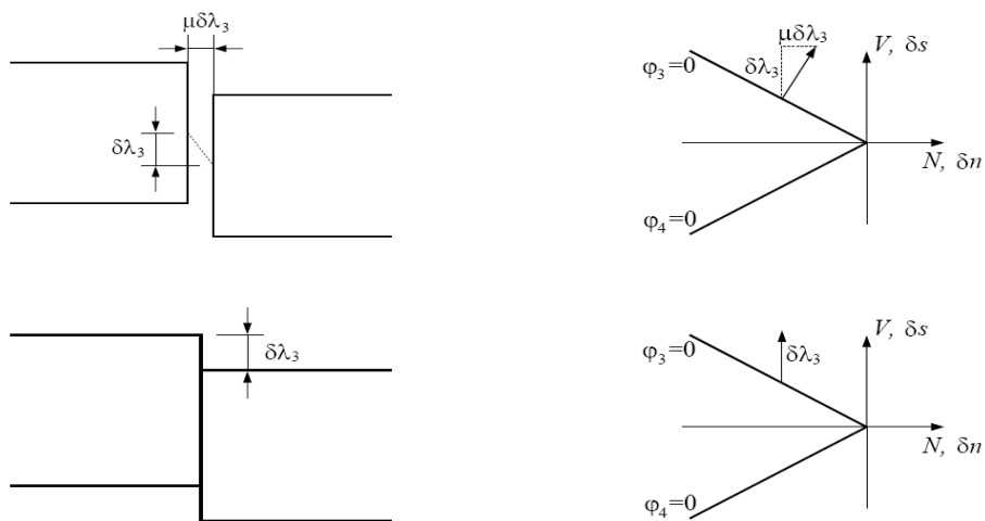
Fig. 16. Associated flow rule (top) with \mu=\tan\Phi=\tan\psi , and non-associated flow rule (below), with null dilatancy ( \tan\psi=0 ). The yield criterion is represented as relationship between the normal ( N ) and shear forces ( V ). The corresponding displacements are the normal ( \delta n ) and tangent ( \delta s ) ones.
