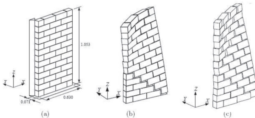
Fig. 15: Out of plane loaded wall, supported at one edge; (a) model; (b) FEM failure mechanism ( \alpha = 0.210 ); (c) limit analysis failure mechanism ( \alpha = 0.216 ) (Orduña and Lourenço, 2005b).
