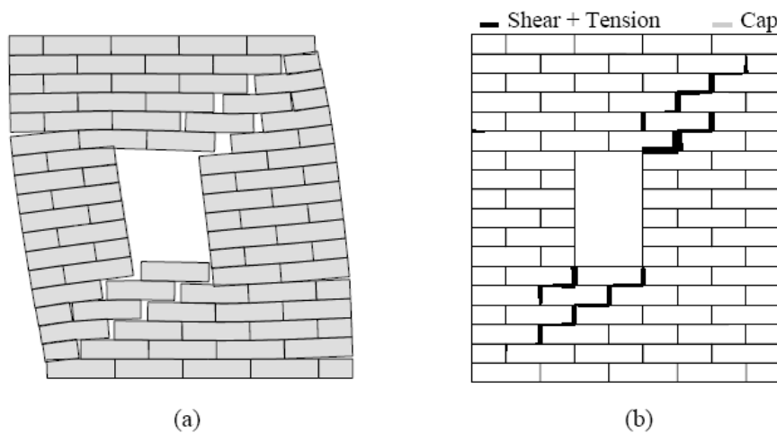
Fig. 27. Micro-modelling of masonry shear walls (Lourenço, 1996). Top: Load-displacement diagram. Bottom: Results of the analysis at a lateral displacement of 2.0 mm: (a) deformed mesh; (b) damage.
