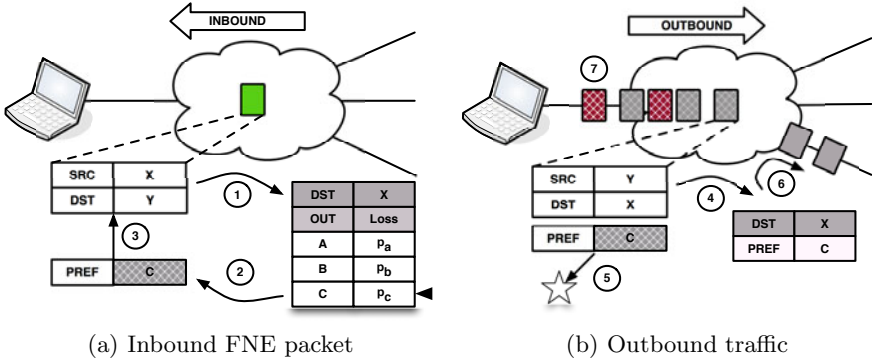
Fig. 1. PREFLEX architecture
