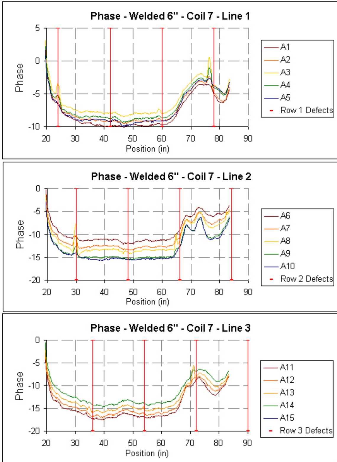
Figure 15: Results of scanning the 6" welded pipe with Coil 7.
