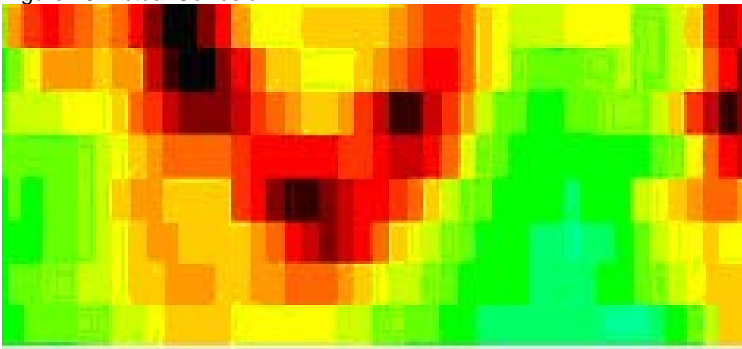
Figure 27: Corrosion as detected by GTI
