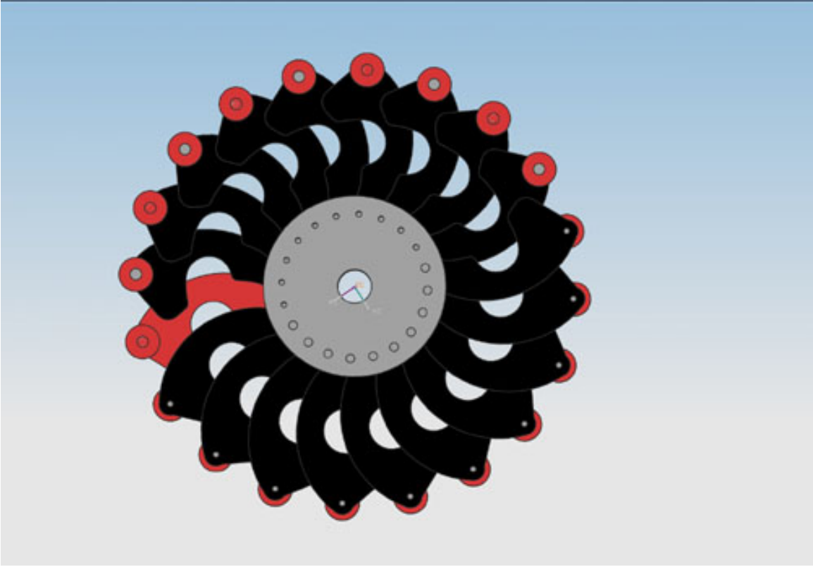
Figure 37: Design 2, top view, fully open.
