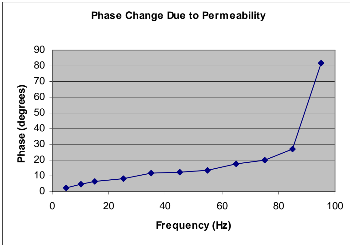
Figure 24: Phase change due to permeability
