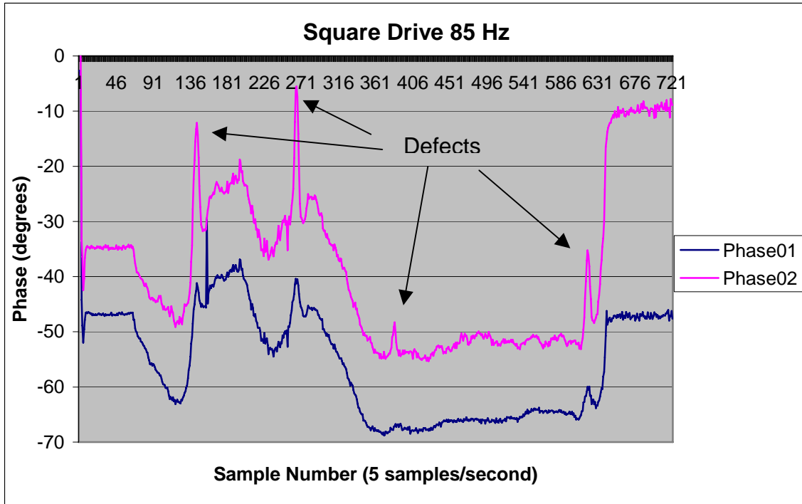
Figure 21: Phase data taken while driving the exciter coil with an 85Hz square wave.
