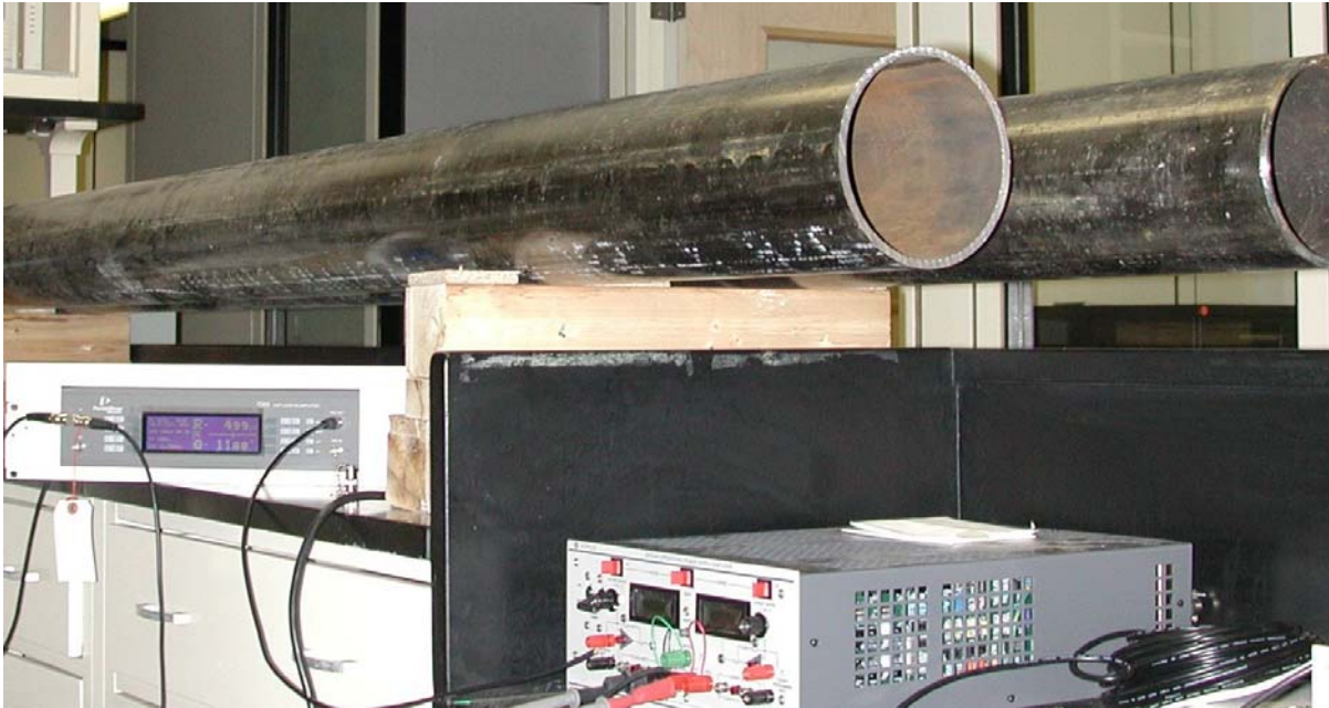
Figure 3: RFEC laboratory setup.
