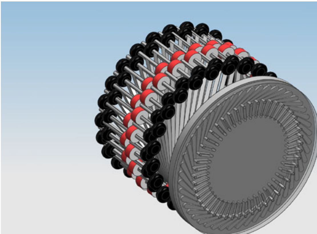
Figure 38: Final Design, isometric view, closed.
