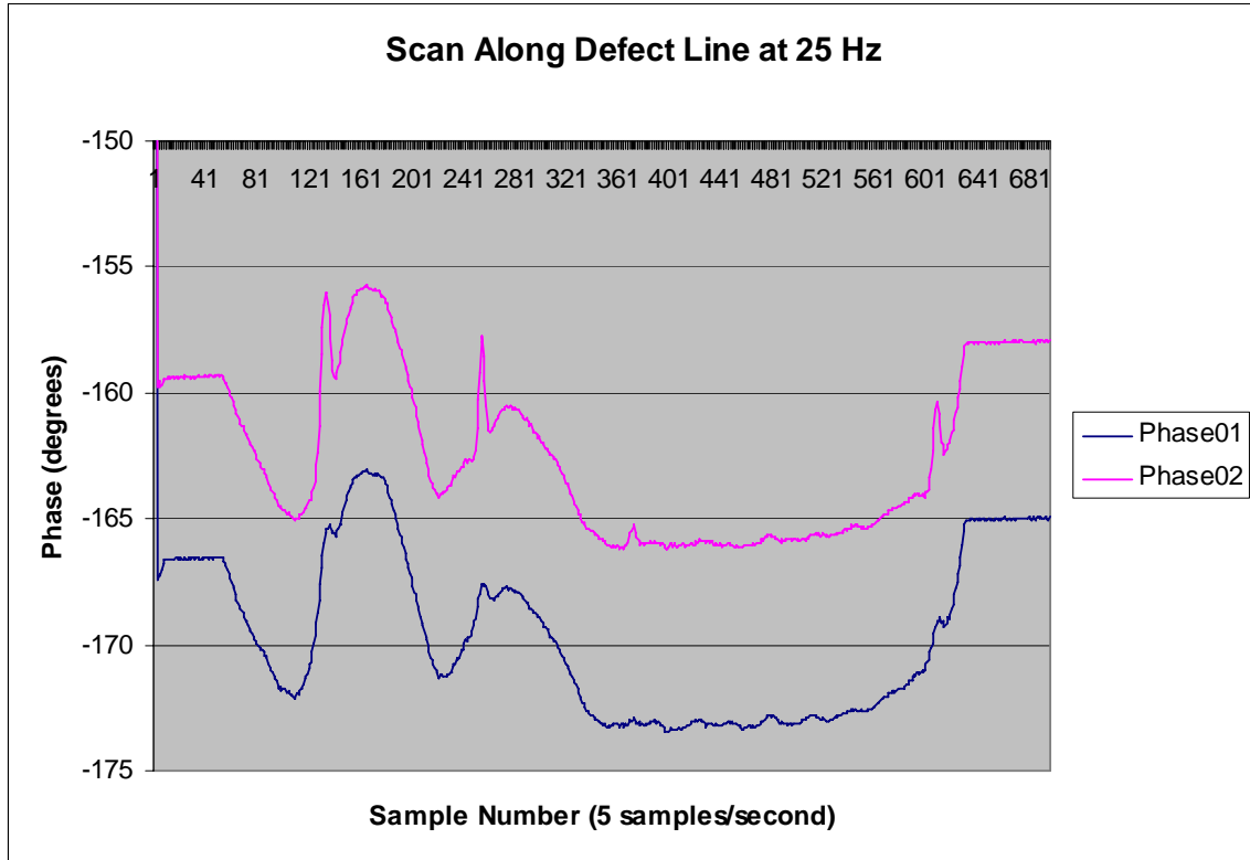
Figure 22: Defect scan at 25Hz
