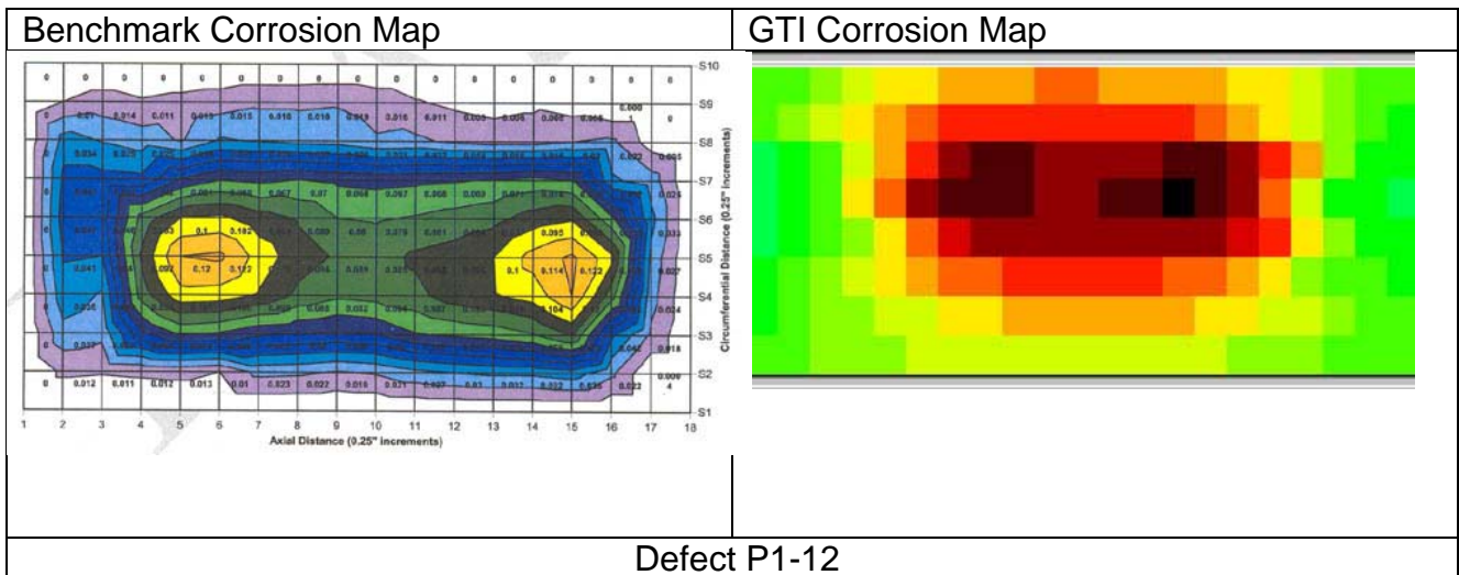
Figure 27: Corrosion as detected by GTI
