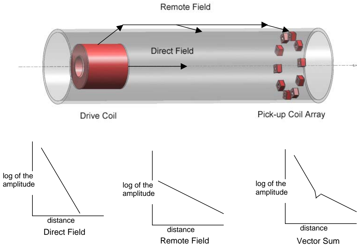
Figure 1: Variation of the amplitude of propagating fields with distance along a pipe.
