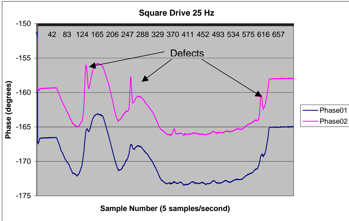
Figure 19: Phase data taken while driving the exciter coil with a 25Hz square wave.
