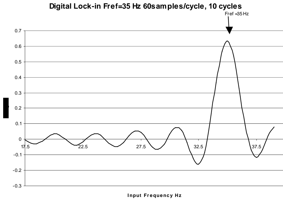
Figure 47: Digital lock-in response as a function of frequency: the lock frequency was 35 HZ.
