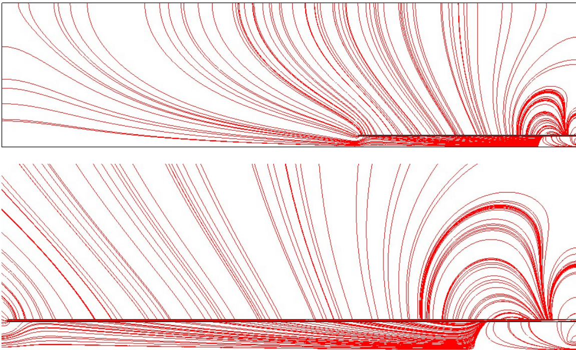
Figure 5: The FEA model of the 6" x 0.25" seamless pipe, showing lines of magnetic flux density.
