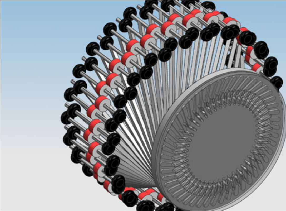
Figure 39: Final Design, isometric view, partially open.
