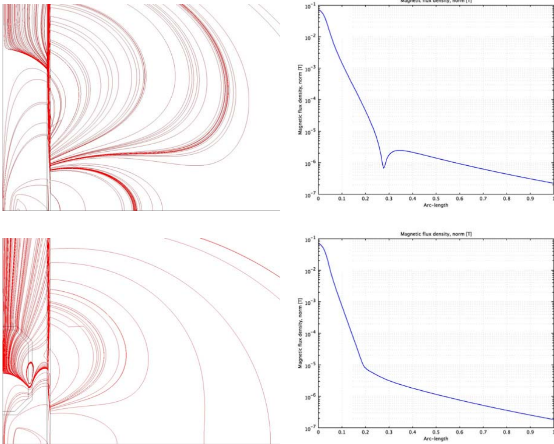
Figure 6: Robot modules attenuate the direct field more rapidly.
