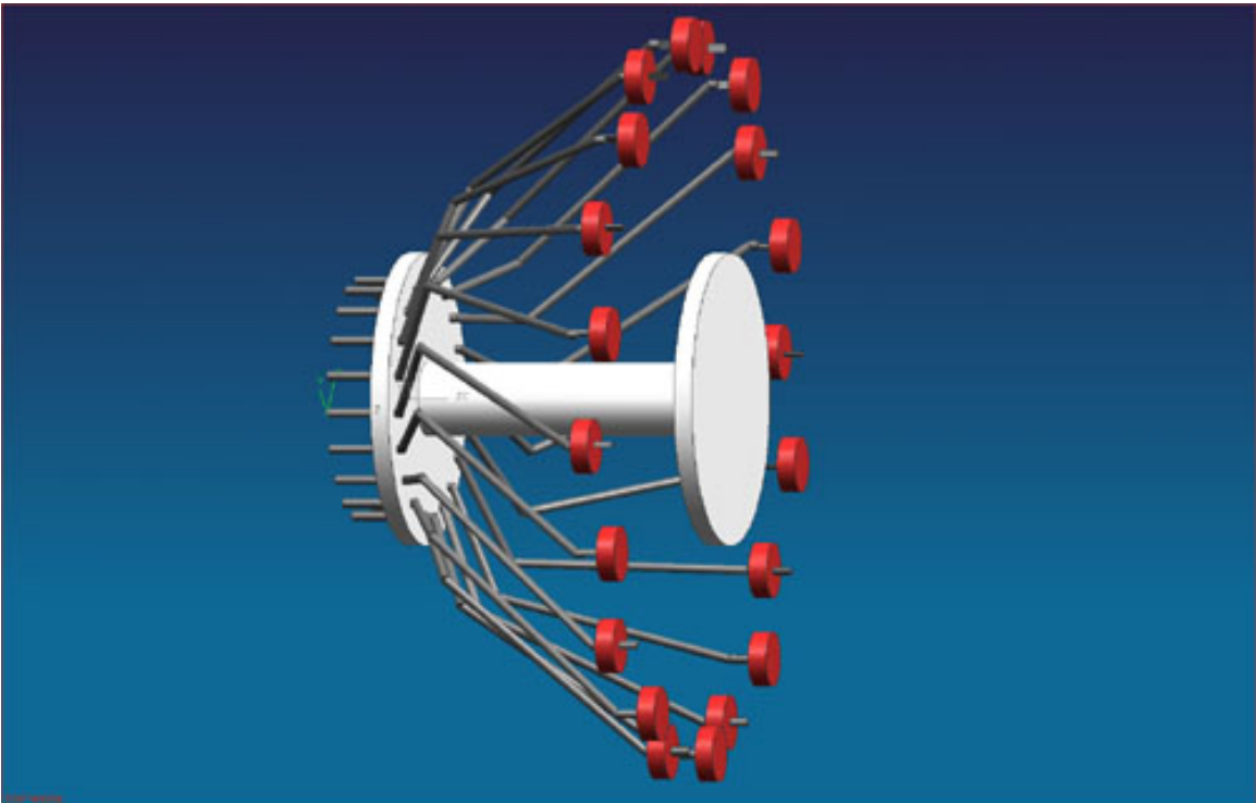
Figure 32: Design 1, side view, arms completely open.
