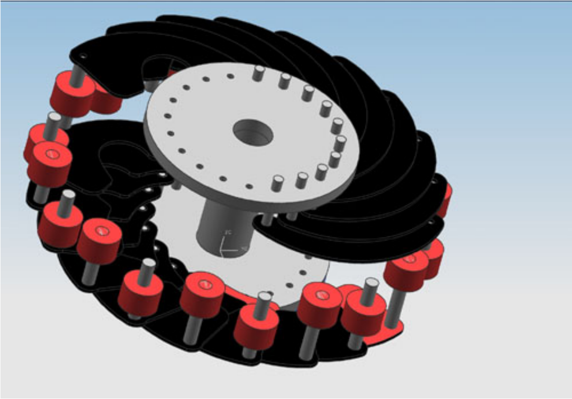
Figure 35: Design 2, isometric view, partially open.
