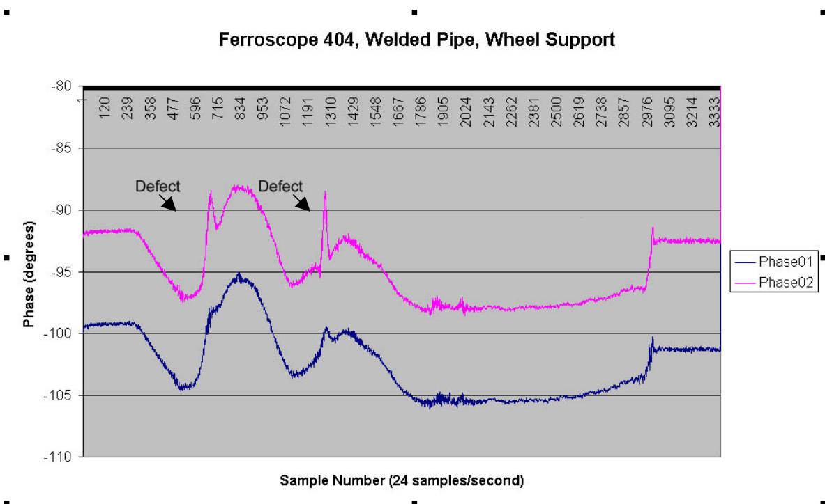
Figure 17: Phase data from defect line one of the seam welded pipe using the Russell boards with wheel supports.
