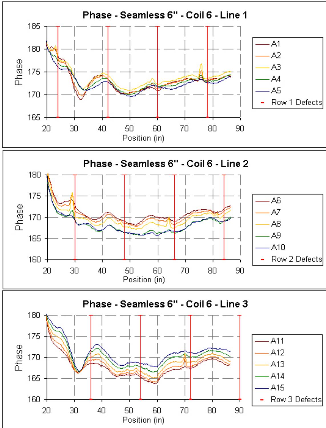
Figure 12: Results of scanning the 6" seamless pipe with Coil 6.
