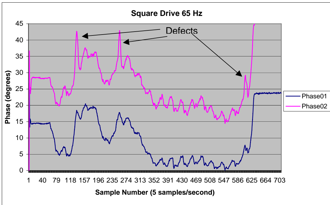
Figure 20: Phase data taken while driving the exciter coil with a 65Hz square wave.
