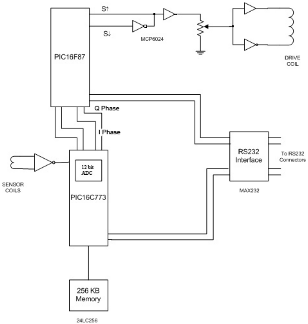
Figure 46: Block diagram of the electronic components.
