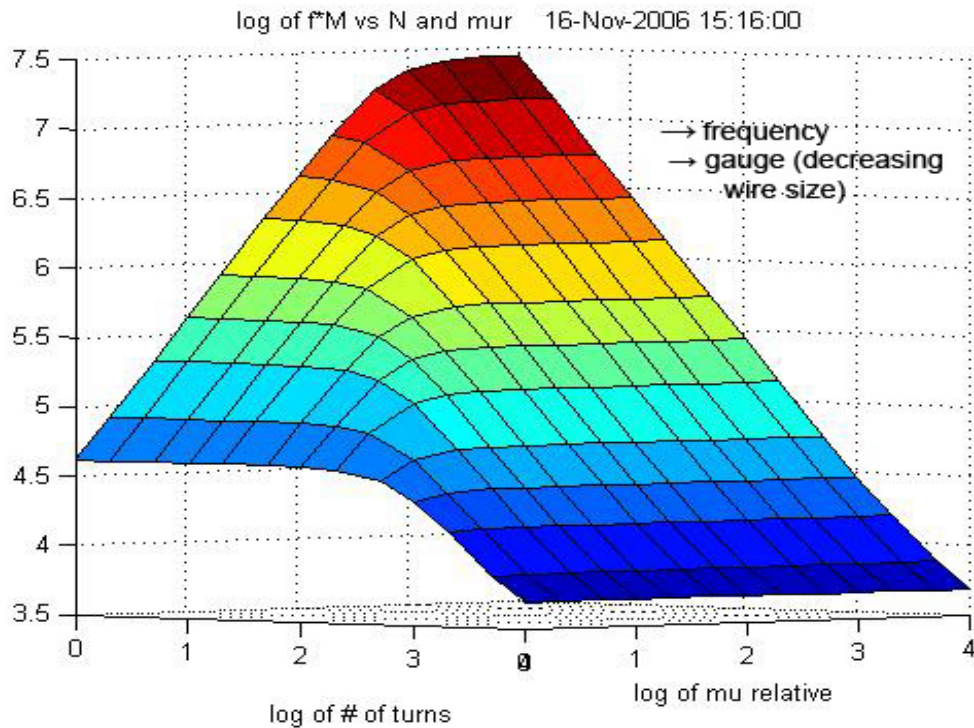
Figure 4: The logarithm of the dipole moment as a function of the number of turns and the relative permeability.
