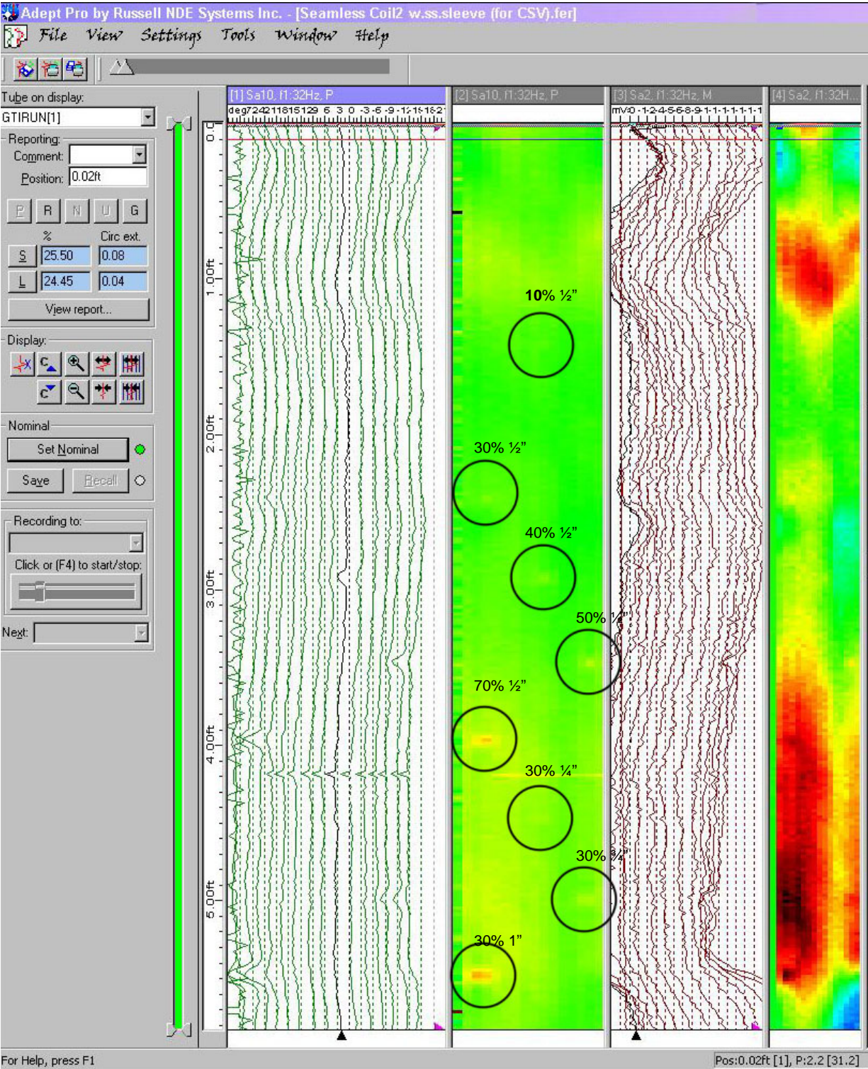
Figure 7: Screen shot of 6" seamless pipe scan from Adept Pro Software.
