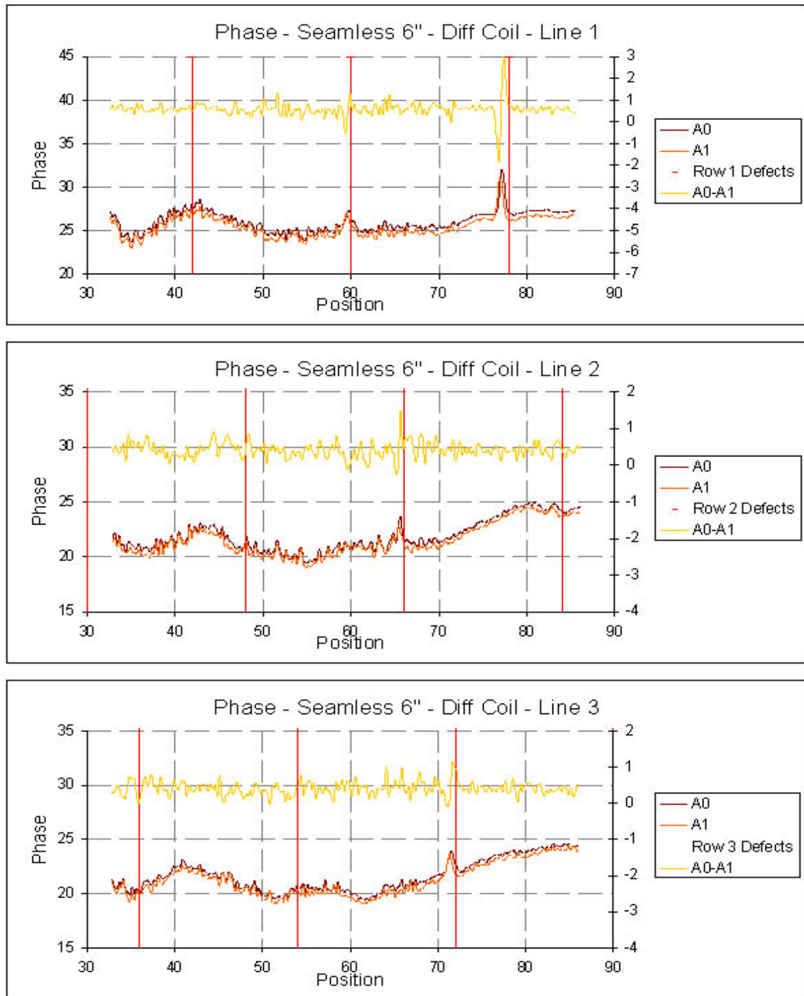
Figure 9: Results of scanning the 6" seamless pipe with differential coils.
