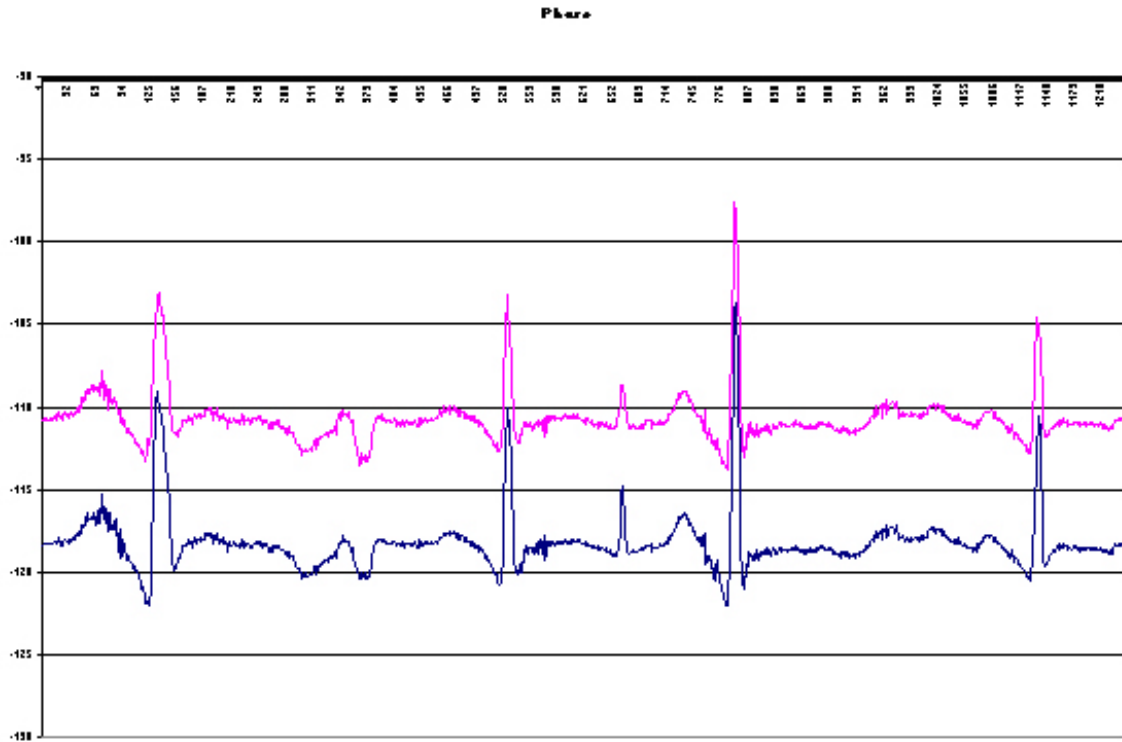
Figure 25: Results from scanning Pipe 3 using Russell equipment.
