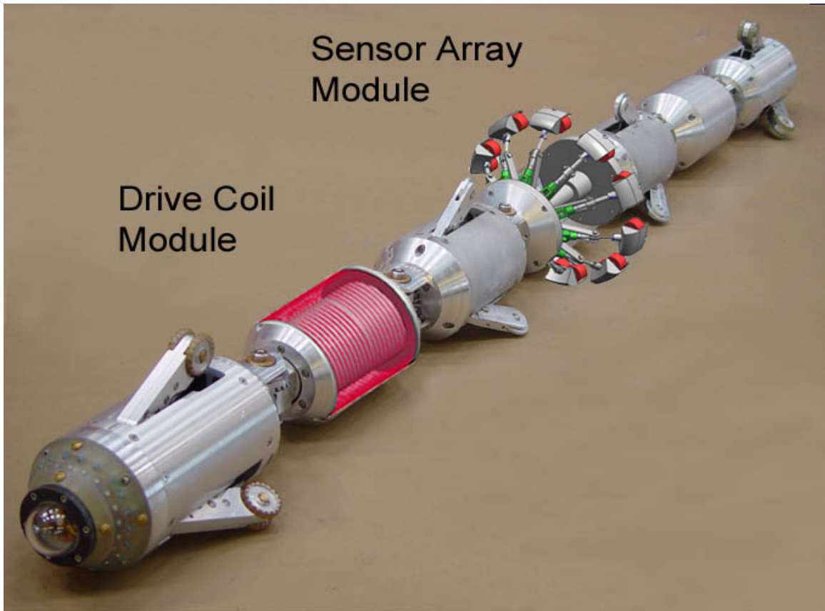
Figure 2: A simulated drawing of the RFEC technology integrated with Explorer.
