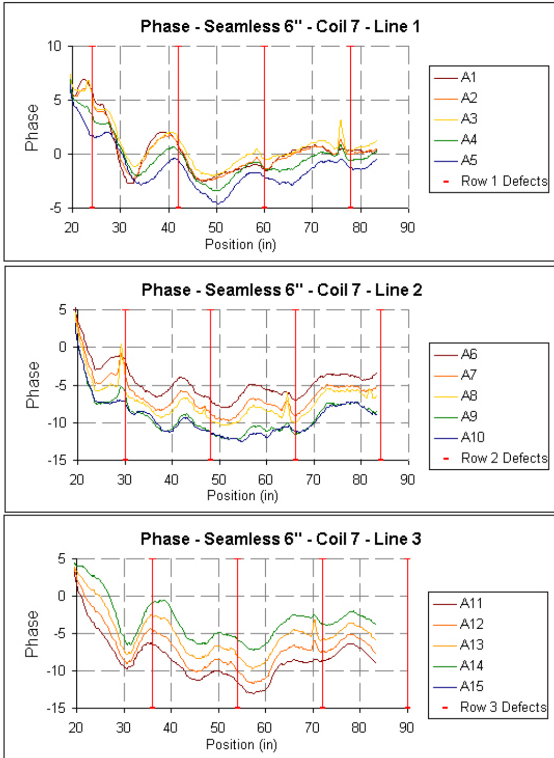
Figure 14: Results of scanning the 6" seamless pipe with Coil 7.
