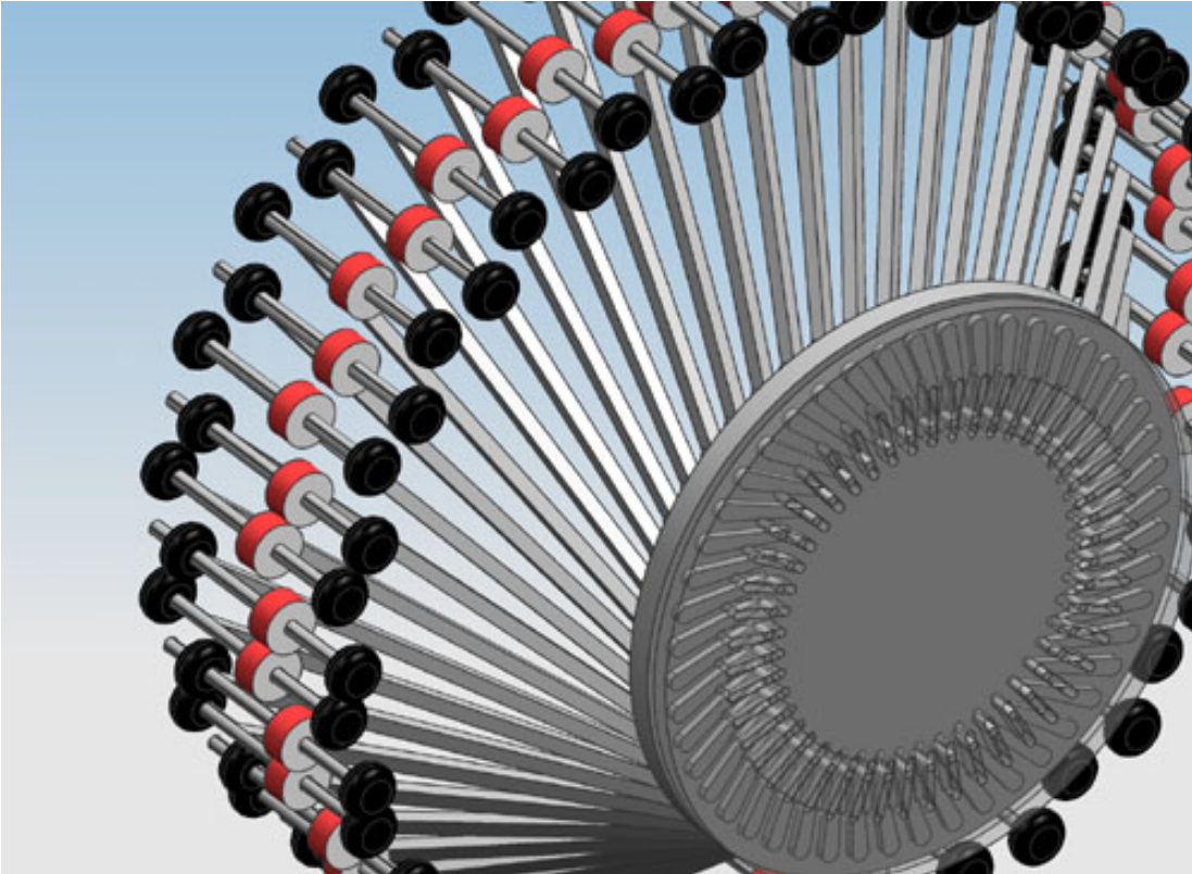
Figure 40: Final Design, isometric view, fully open.
