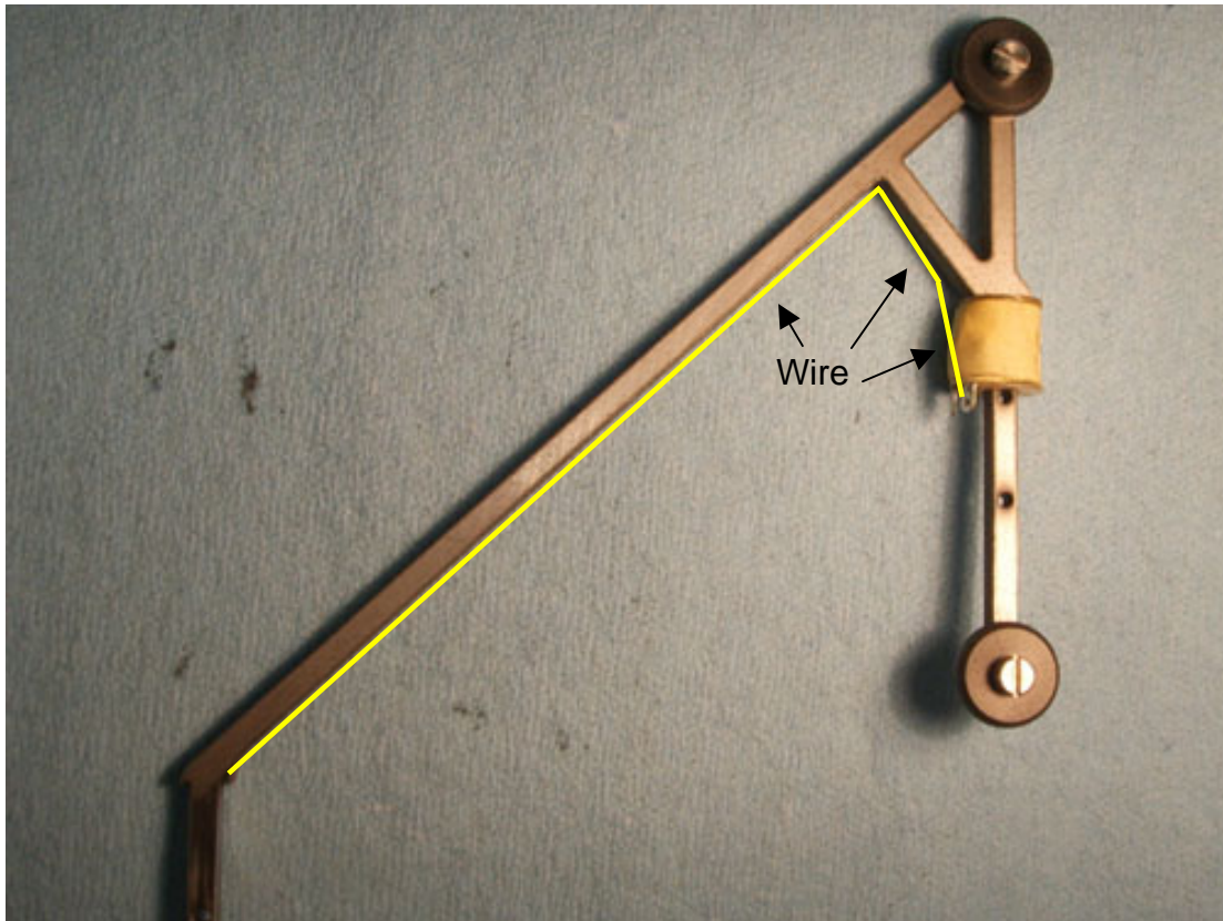
Figure 41: Single arm with coil.
