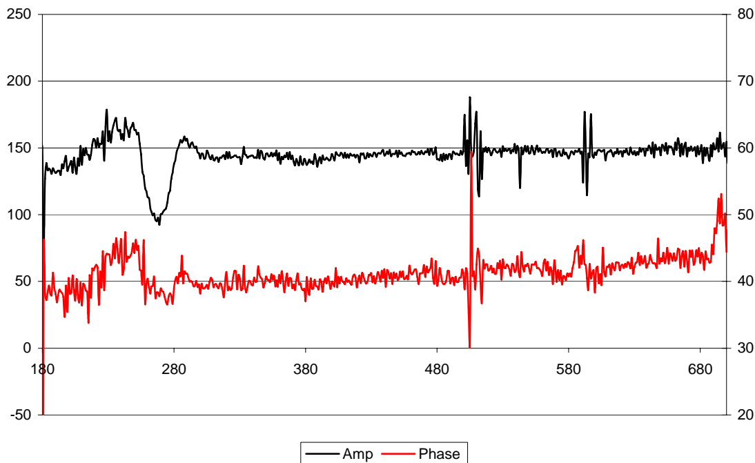
Figure 48: A test run of the electronic assembly using a master and one slave microprocessor programmed with a digital lock-in amplifier.
