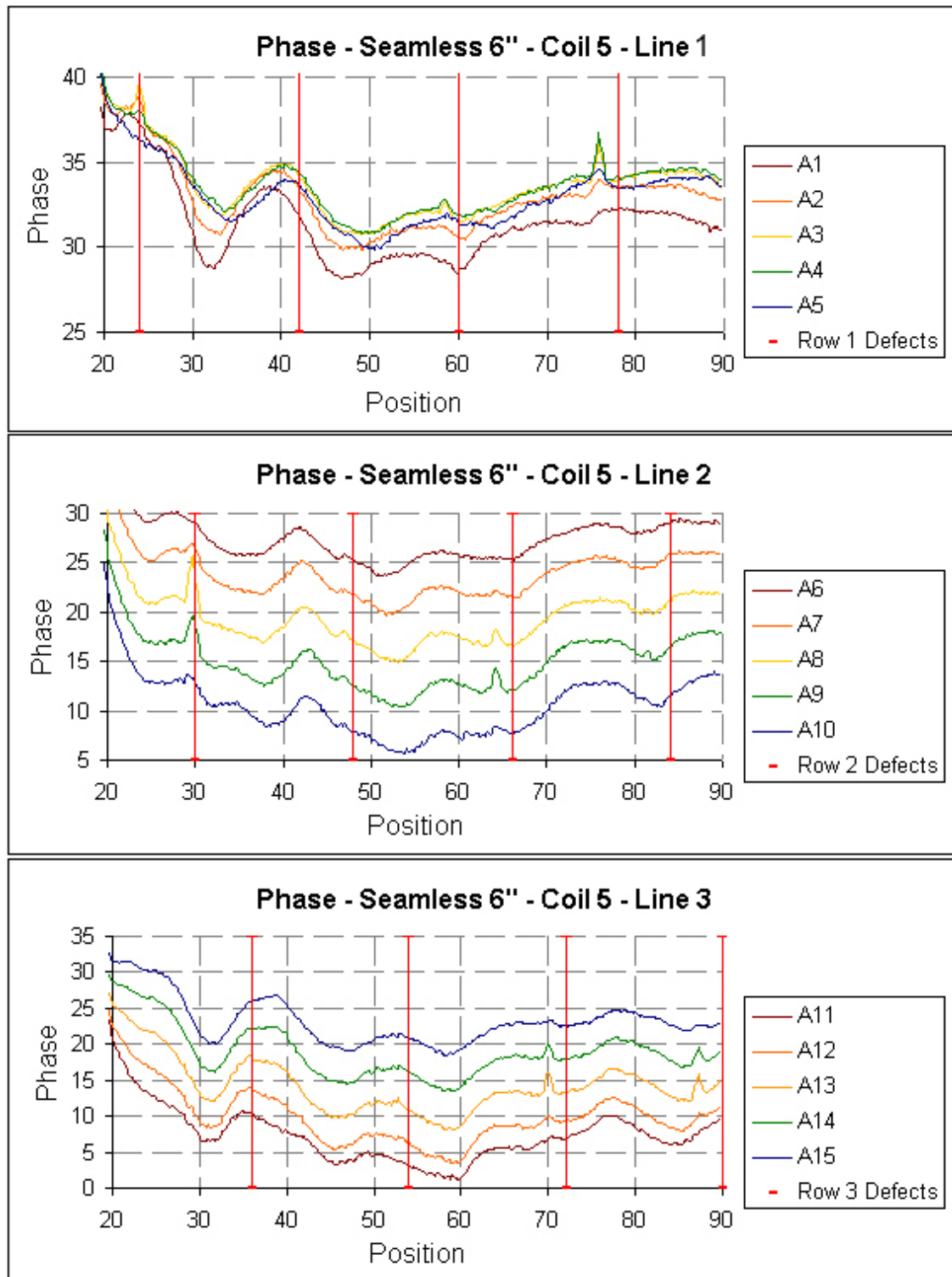
Figure 10: Results of 6" seamless pipe scan using Coil 5 with a mock module.
