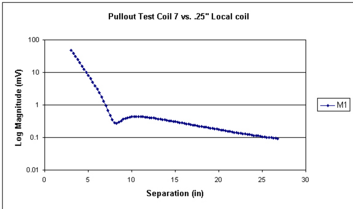
Figure 13: Results of a pullout test using Coil 7.
