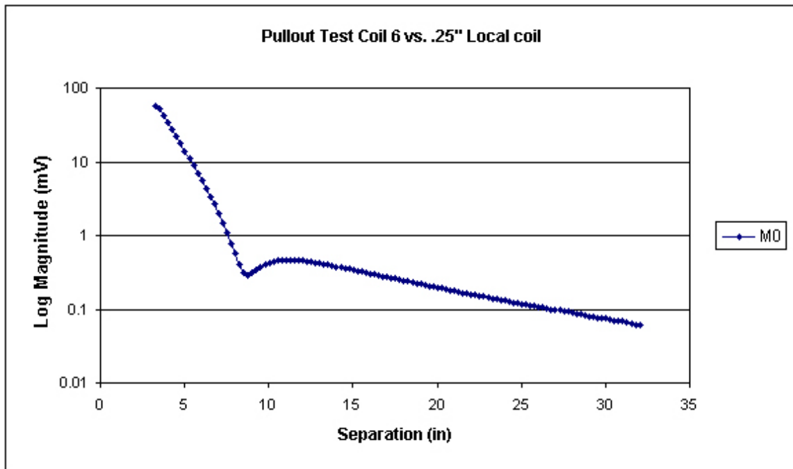
Figure 11: Results of a pullout test using Coil 6.
