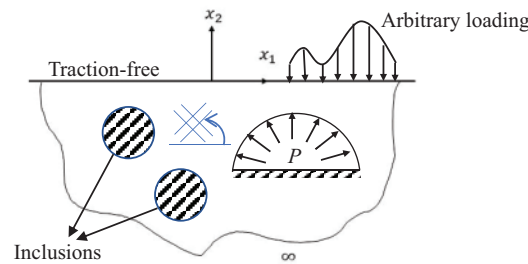
Figure 1: Anisotropic half-plane containing inclusion(s)/hole(s)
