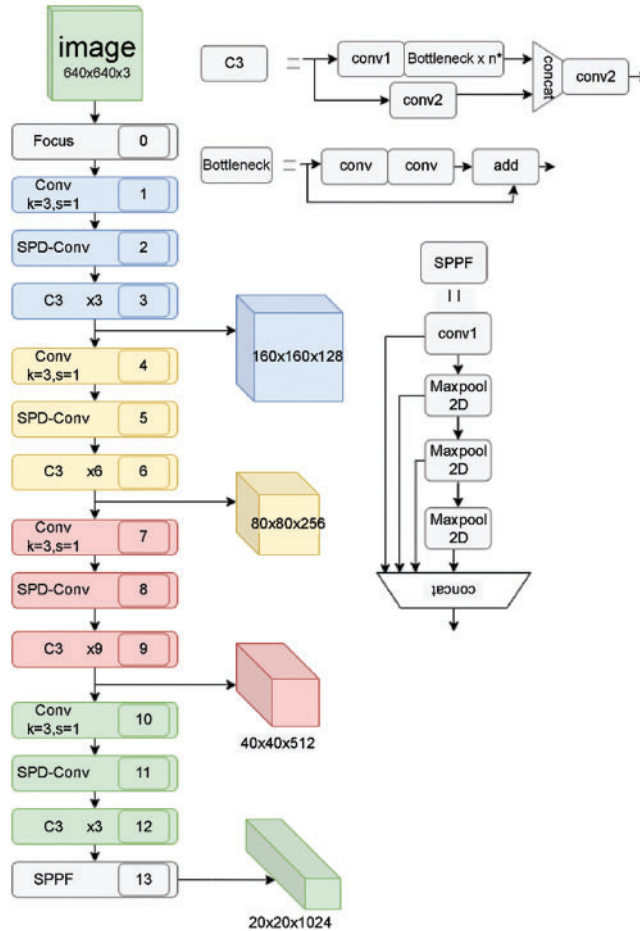
Figure 3: Backbone structure: The novel SPD-Conv module and additional feature map output channel address limitations in existing CNN architectures. This design preserves fine-grained texture information and enhances feature learning efficiency for rod-end joint bearings, particularly beneficial for smaller specimens. The structure mitigates information loss typically associated with strided convolutions or pooling layers, enabling more accurate and detailed analysis across various bearing sizes
