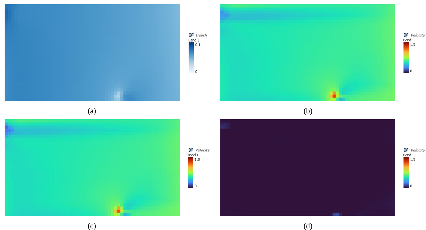
Fig. 7. Results at the end of the simulation: (a) flow depth; (b) flow velocity (modulus); (c) flow velocity in the X direction; (d) flow velocity in the Y direction.
