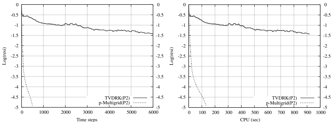
Fig. 34 Comparison of convergence history versus time steps (left) and CPU time (right) between TVBRK and p -multigrid methods using DG(P2) approximation on the coarse mesh for subsonic flow past a sphere at M_\infty = 0.5 .
