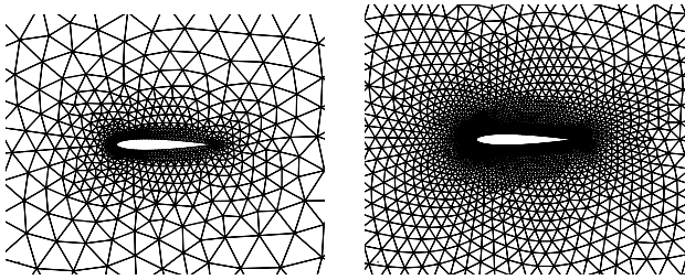
Fig. 16 Coarse (left, nelem = 1999 , npoin = 1048 , nboun = 97 ) and fine (right, nelem = 8006 , npoin = 4102 , nboun = 198 ) unstructured mesh used for computing transonic flow past a NACA0012 airfoil.
