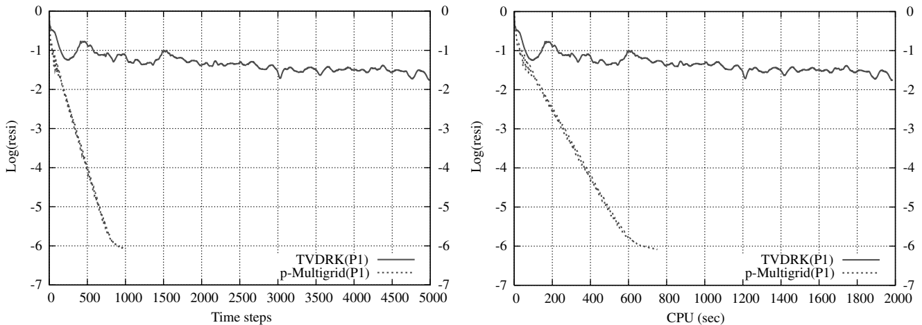
Fig. 33 Comparison of convergence history versus time steps (left) and CPU time (right) between TVBRK and p -multigrid methods for DG(P1) computation on the medium mesh for subsonic flow past a sphere at M_\infty = 0.5 .
