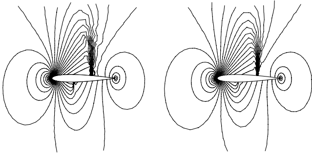
Fig. 17 Computed pressure contours in the flowfield by DG(P2) method on the coarse mesh (left) and FV(P1) method on the fine mesh (right) for transonic flow past a NACA0012 airfoil at M_\infty = 0.8 , \alpha = 1.25 deg.
