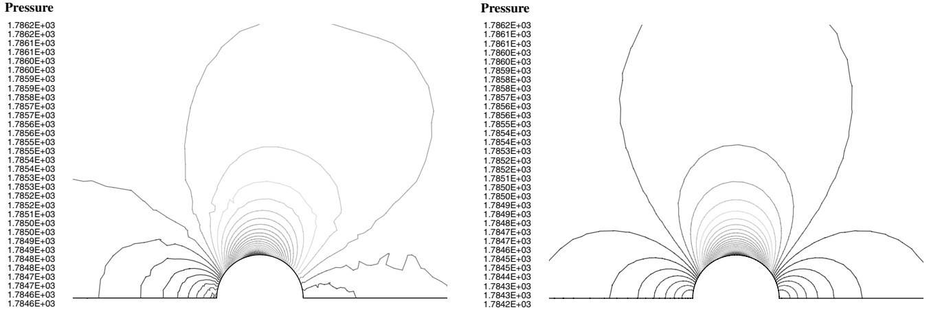
Fig. 15 Computed pressure contours obtained by the FV(P1) (left) and DG(P1) (right) methods for low-Mach-number flow past a circular cylinder at M_\infty = 0.01 .
