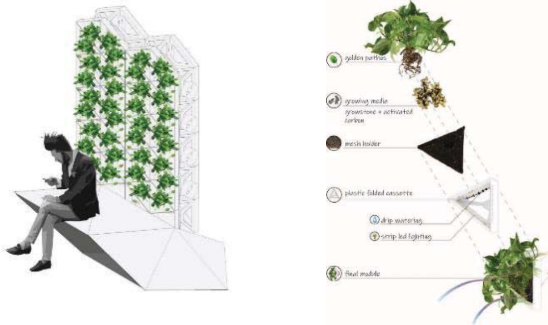
Figure 2. a. The double-sided prototype of plant-base air filtering system; b. Components of plant-based air filtering system.
