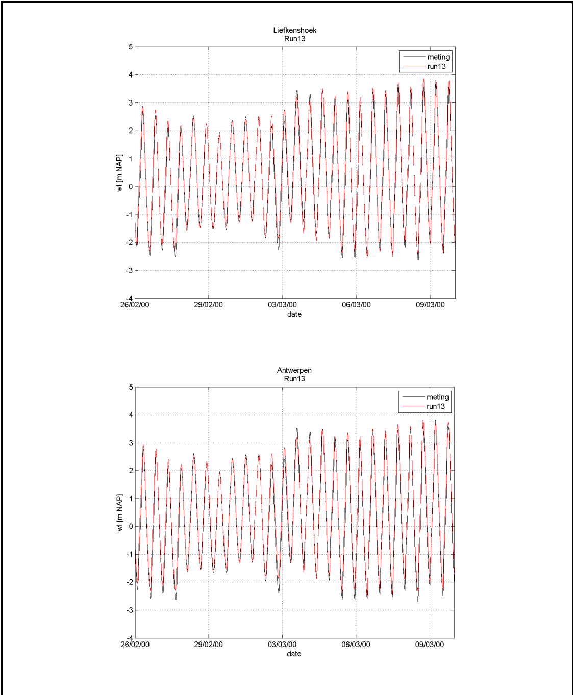
Figure A-18: Water level: computed results and measurements (26/02 to 09/03)
