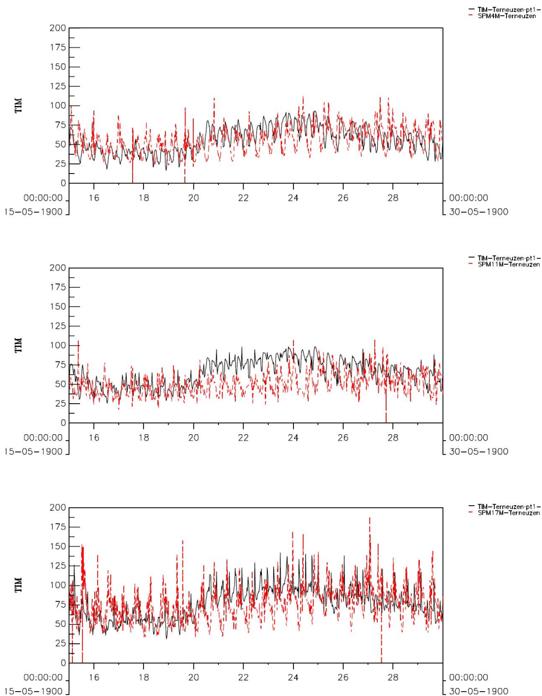
Figure B.9.2b: Computed SPM concentrations at DOW-jetty near Terneuzen for a neap-spring period (q10) . Observations are included in red and model results in black. Upper panel: obs. NAP-4m, model layer 1. Middle panel: obs. NAP-11m, model layer 2. Lower panel: obs. NAP-17m, model layer 4.
