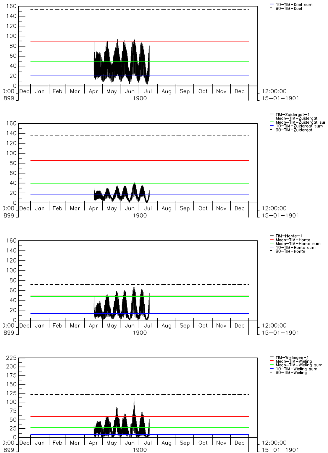
Figure B.9.1h: Computed SPM surface concentration at 4 stations along the Scheldt estuary for a 3-month simulation (q06). Observed mean levels are indicated with horizontal lines. In blue: 10-percentile level; in green: mean summer level; in red: mean winter level; dashed black: 90-percentile level..
