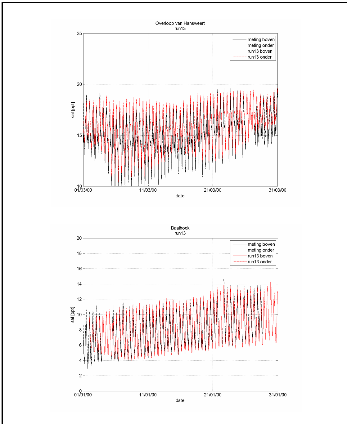
Figure A-32: Salinity: computed results and measurements
