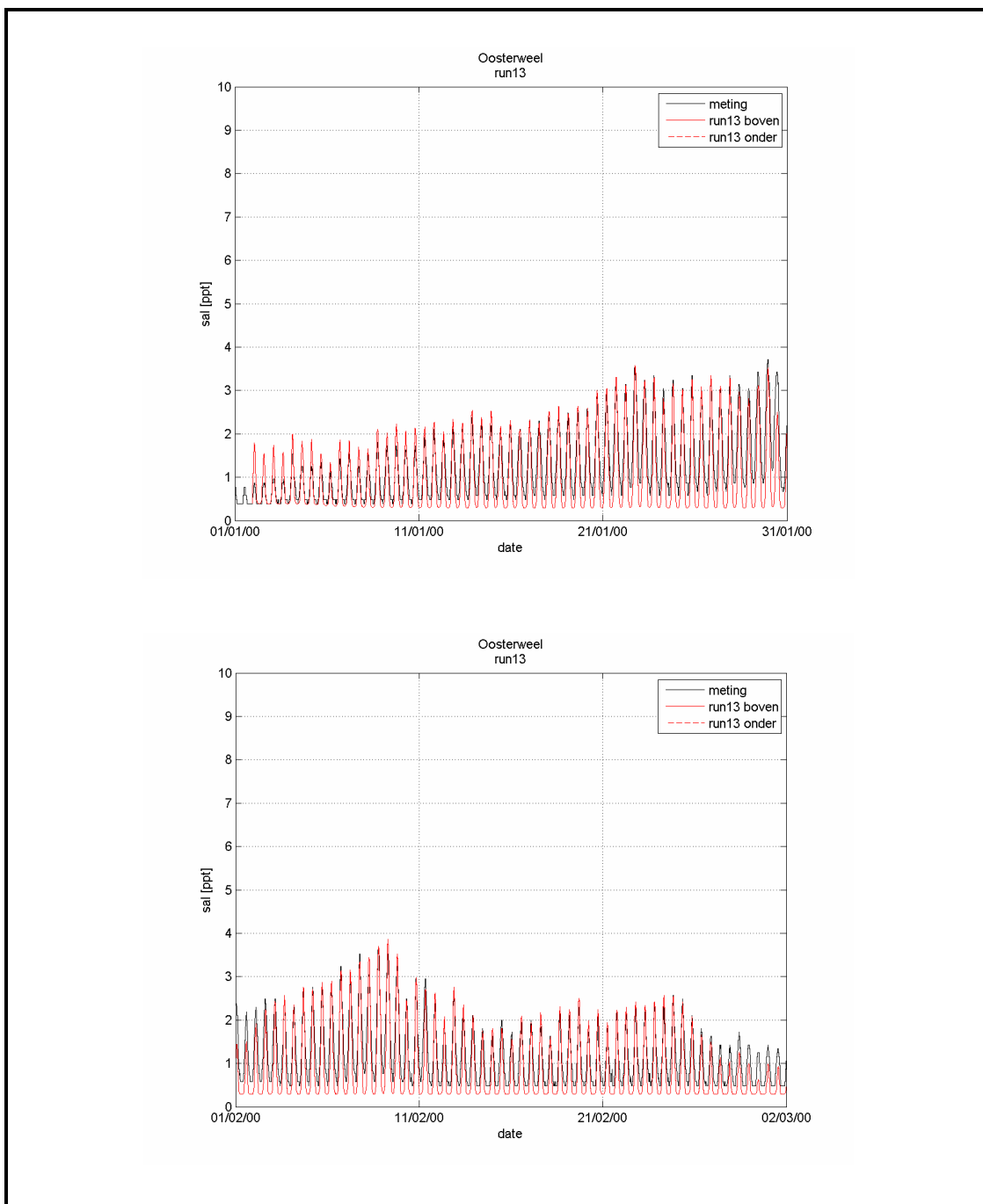
Figure A-34: Salinity: computed results and measurements
