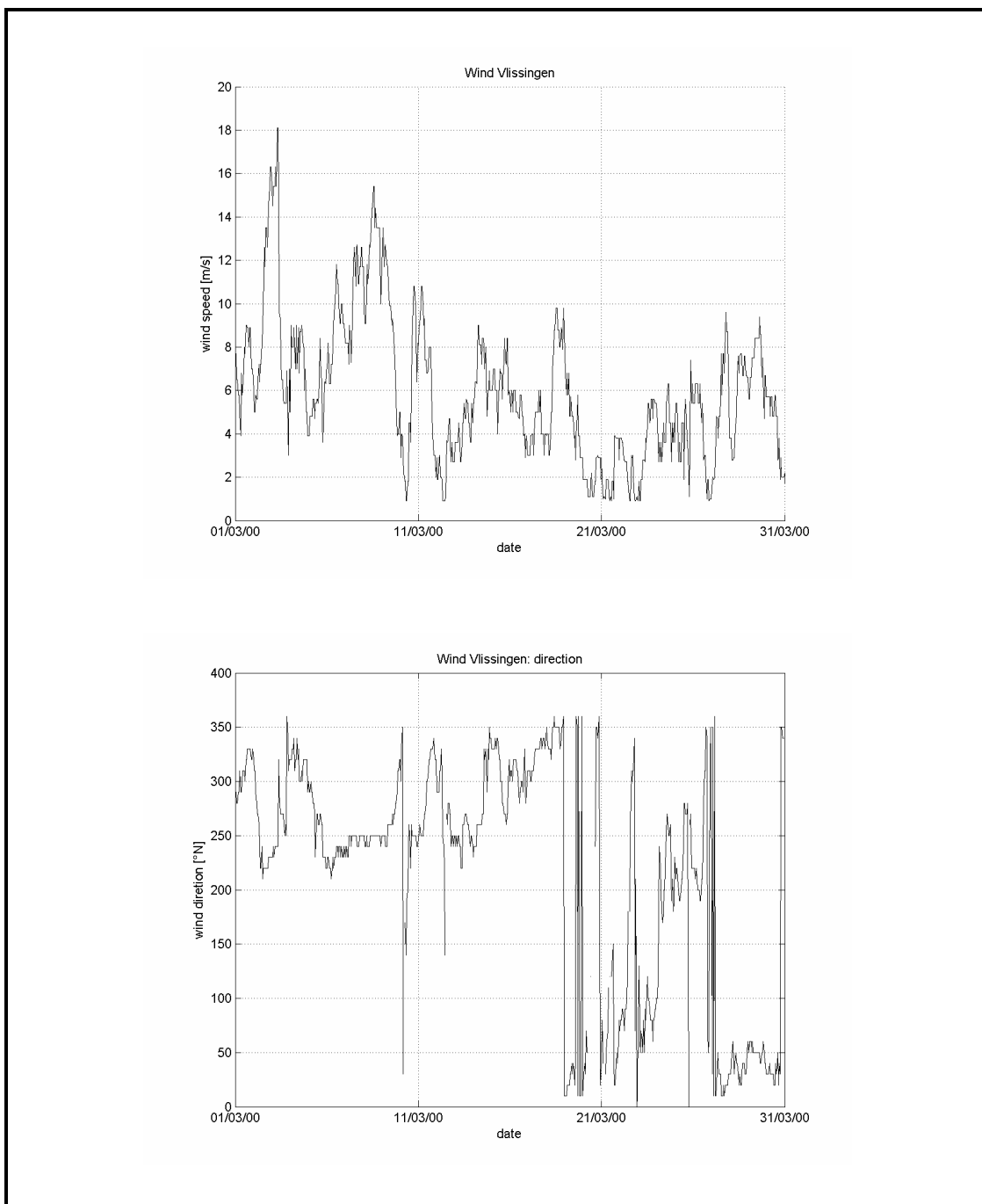
Figure A-14: Wind Vlissingen March. 10 minute mean windspeed (top) and direction (bottom)
