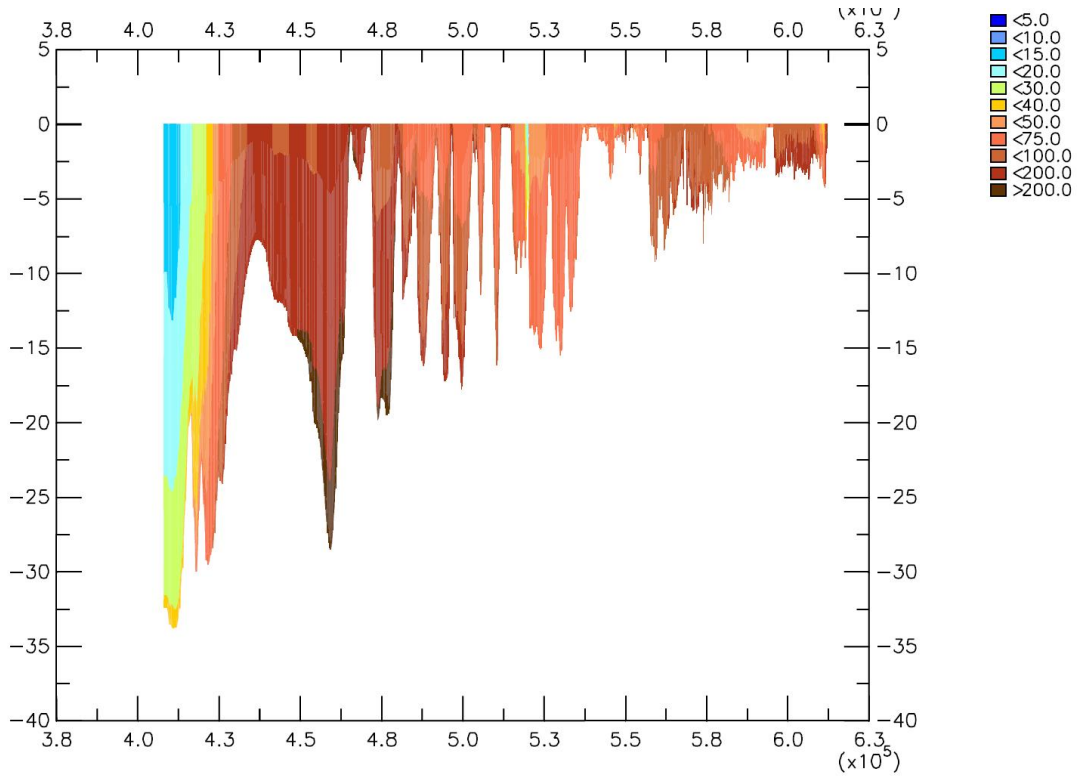
Fig. B.1c: 14-day winter averaged vertical SPM concentration transect (mg/l) along the estuary (left = sea), original dumping locations (ws15)
