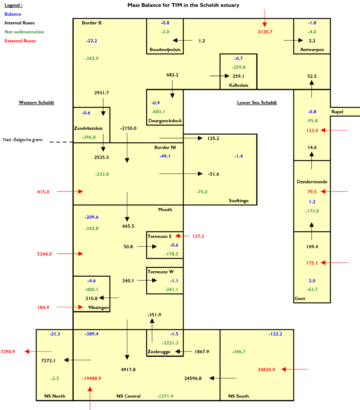
Figure B.8f: Mud balance for simulation Jan – Mar 2003 (q03), expressed in kton/year.
