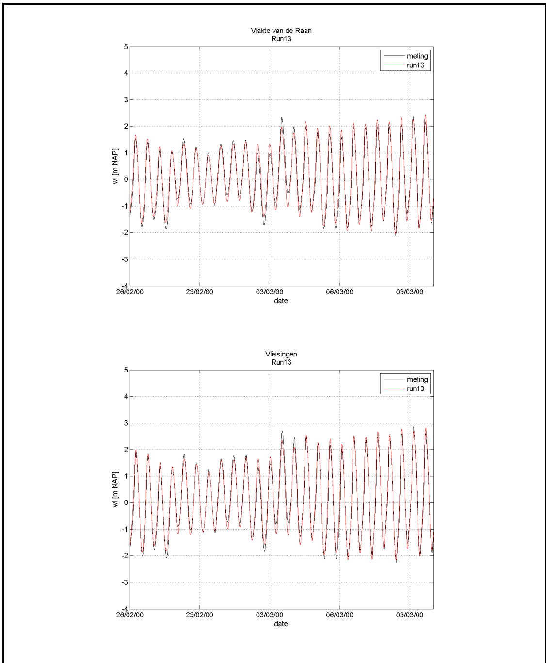
Figure A-16: Water level: computed results and measurements (26/02 to 09/03)
