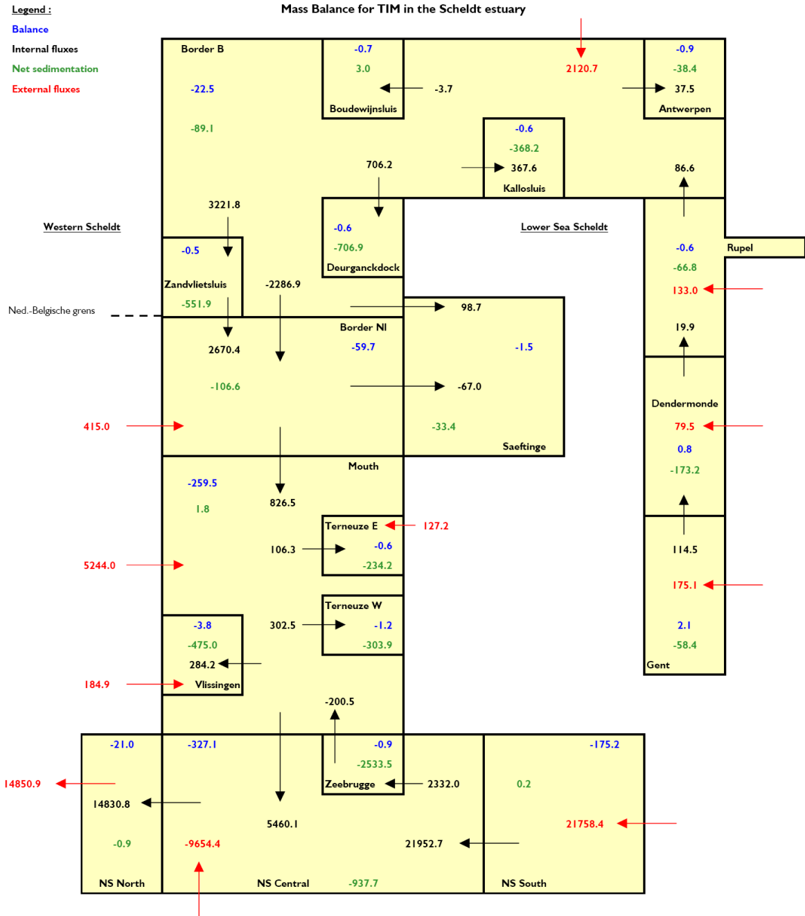
Figure B.10.3a: Mud balance for simulation Jan – Mar 2003 (q100|12km), expressed in kton/year.
