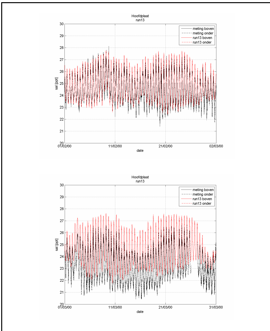
Figure A-30: Salinity: computed results and measurements
