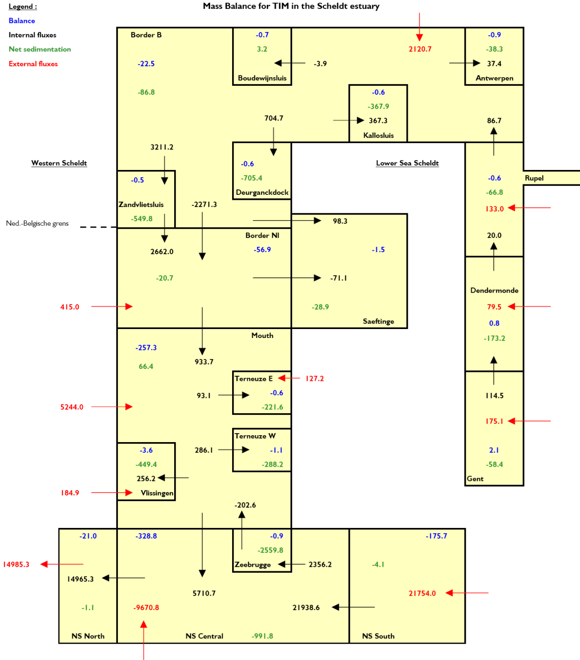
Figure B.10.5a: Mud balance for simulation Jan – Mar 2003 (q10W12km), expressed in kton/year.
