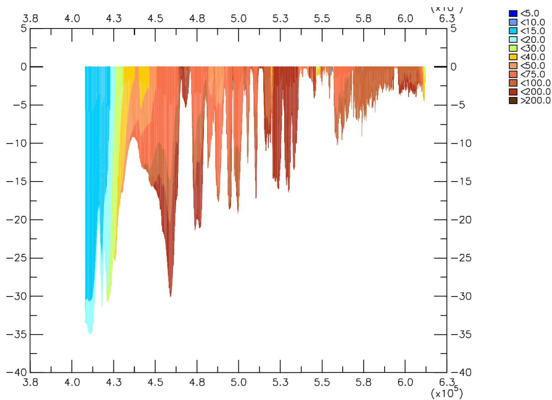
Fig. 4.5a: 14-day winter averaged vertical SPM concentration transect (mg/l) along the estuary (left = sea), 5 horizontal layers (05L01).
