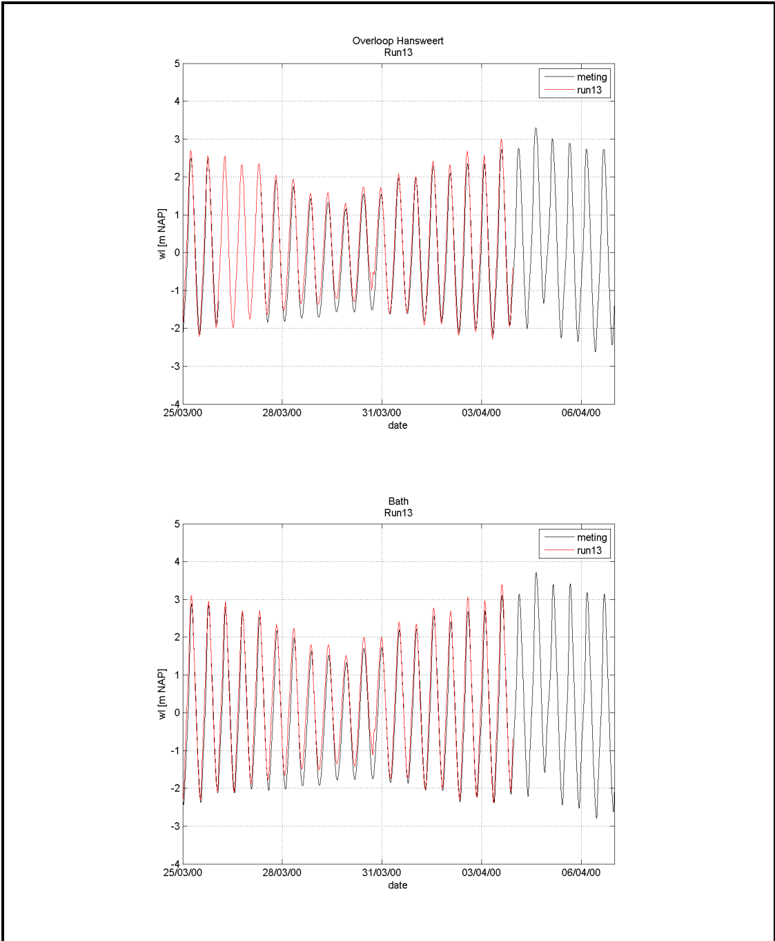
Figure A-20: Water level: computed results and measurements (25/03 to 06/04)
