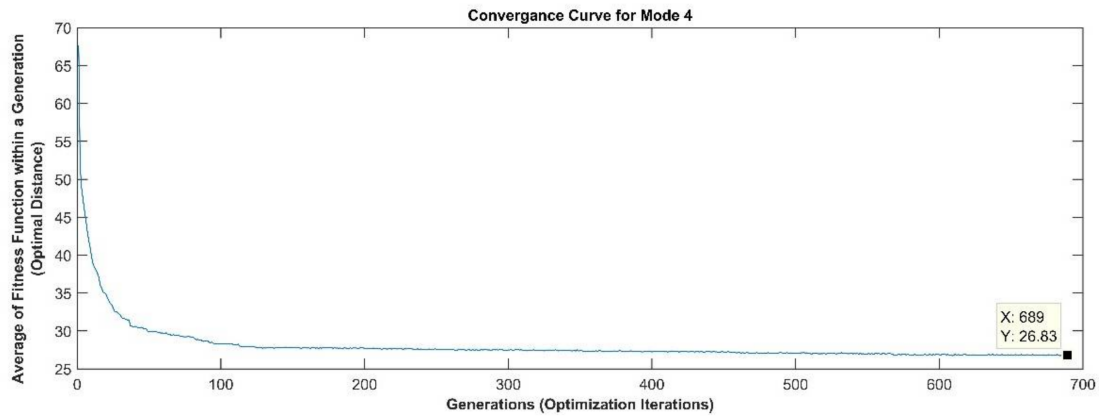
Figure 8. Convergence curve of the GA for Mode 4.
