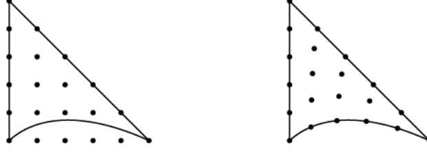
Figure 8. 5th-order nodal distributions in I_e : for equally-spaced nodes in the straight-side triangle (left) and adapted to the NURBS side (right)
