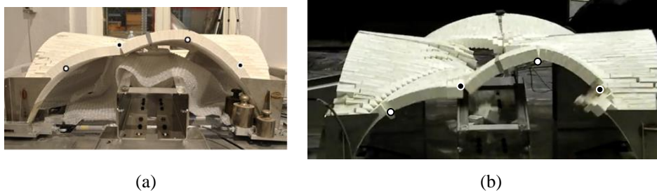
Figure 11. Comparison between the quasi-static [6] (a) and the shake table tests (b).
