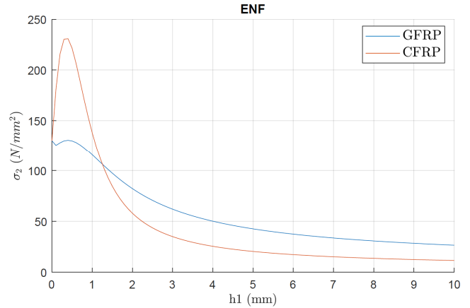
Figure 10. Bending strength of the 3D printed arm with respect to the reinforcement thickness (GFRP and CFRP) for an ENF specimen assuming G_{IIc} = 1 N/mm.
